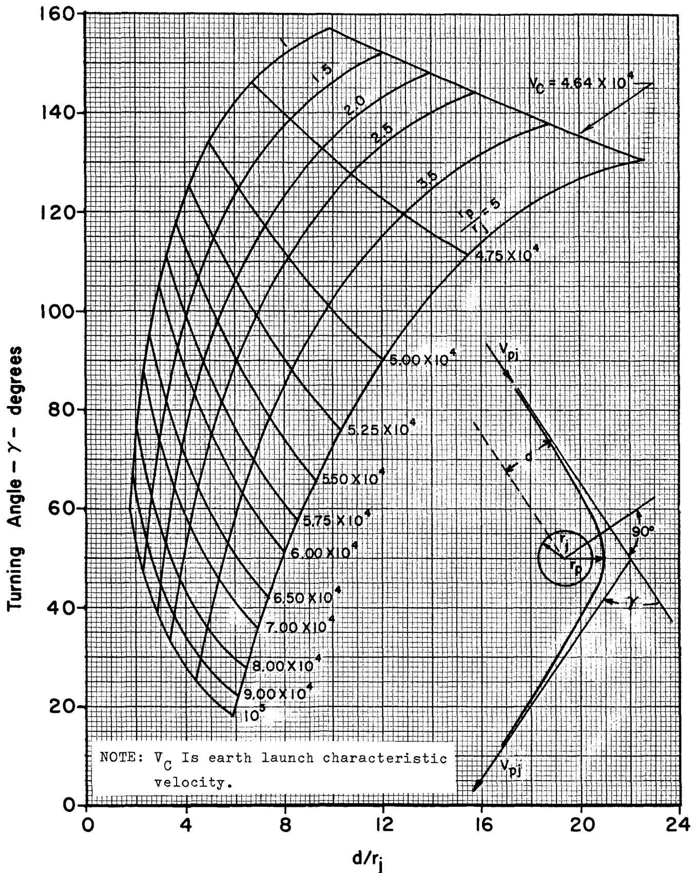
FIGURE B-4. TURNING ANGLE VERSUS MISS DISTANCE AT JUPITER
