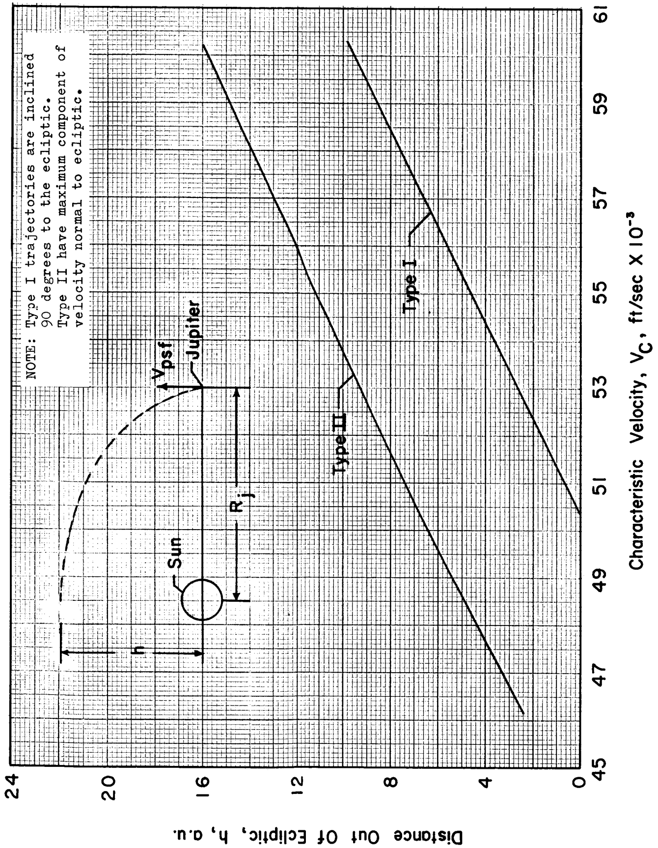
FIGURE 7. DISTANCE FROM ECLIPTIC AT SUN PASSAGE
