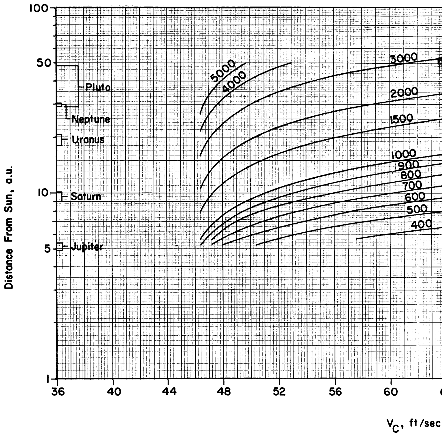
FIGURE I. VELOCITY REQUIRED FOR OUTER PLANETARY
