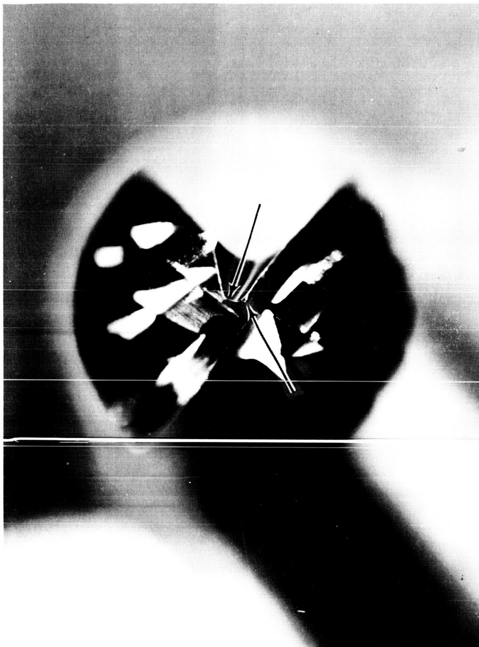
Figure 2-20 Enlarged view of burr drill point showing flat spot at chisel point of primary cutting edge. Weak burr point at chisel point, left side.
