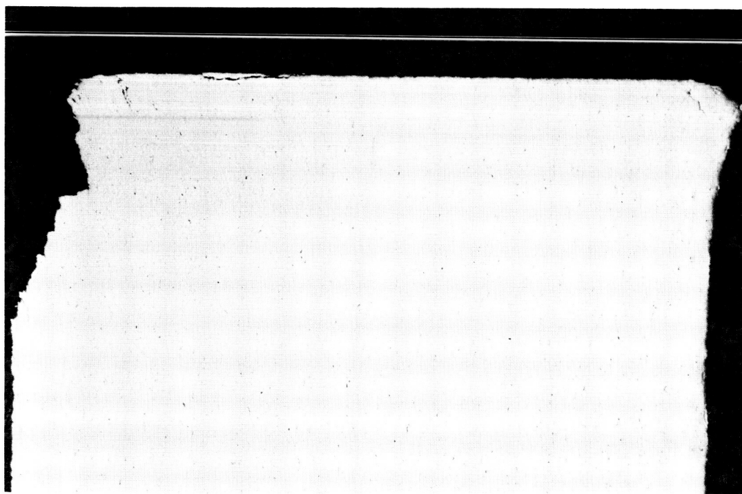
Figure 2-40 Cross-section of hole drilled using excessive feed rate. Note spalled region - unetched. (85X)
