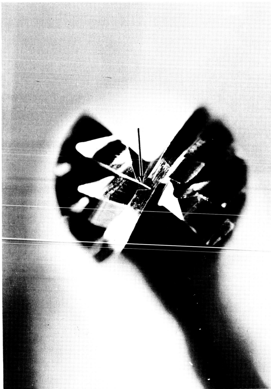
Figure 2-23 Enlarged microscopic view of burr drill point showing gash was allowed to progress into primary land at chisel point.
