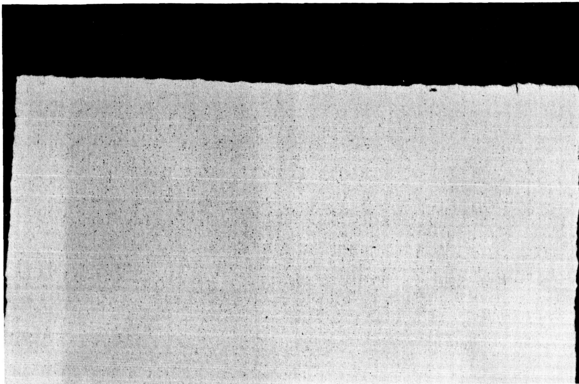
Figure 2-68 Cross-section of EDM finish cut at 130,000 CPS - metal removal rate .125 cu. in./hr. (83X)
