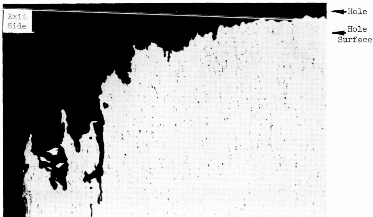
Figure 2-35 Cross-section of hole drilled with dull drill showing spalled edge (unetched). (500X)
