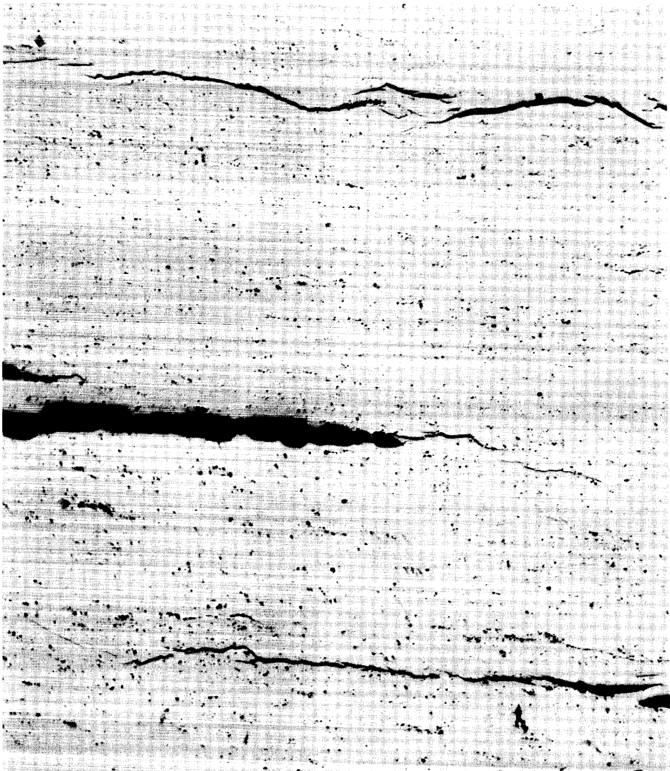
Figure 2-6 Improperly drilled hole through o.100 sheet showing delaminations. Hole wall near left of photograph. (500X)
