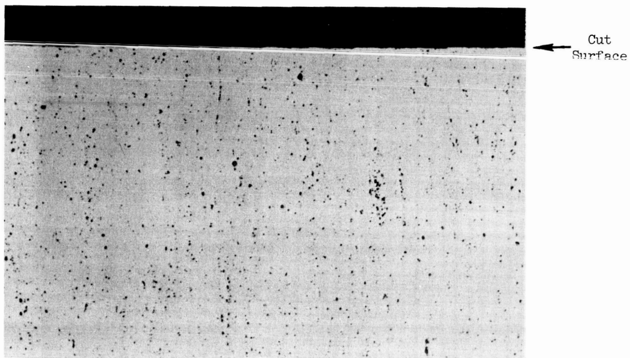
Figure 2-48 Cross-section of surface cut dry on abrasive wheel. Feed rate: 7.5 IPM at 8,240 SFM. (500X)
