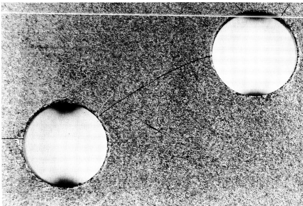
Figure 2-31 Hole drilled with dull drill showing radial cracking & bridging from hole to hole. (10X)
