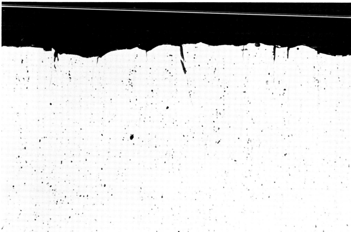
Figure 2-67 Cross-section of EDM finish cut at 130,000 CPS - metal removal rate .285 cu. in./hr. (500X)
