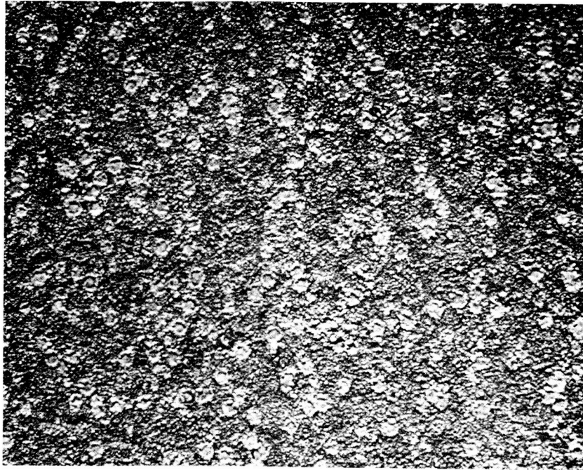
Figure 2-97 Macrograph of Area Chemically Milled with a 50% Phosphoric Acid - 20% Sulfuric Acid Solution (Specimen #4) (18X).
