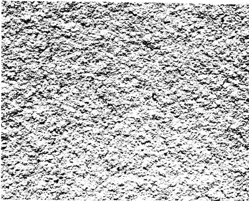
Figure 2-86 Macrograph of Area Chemically Milled with a 15% Solution of Ammonium Bifluoride (Specimen #10) (18X).
