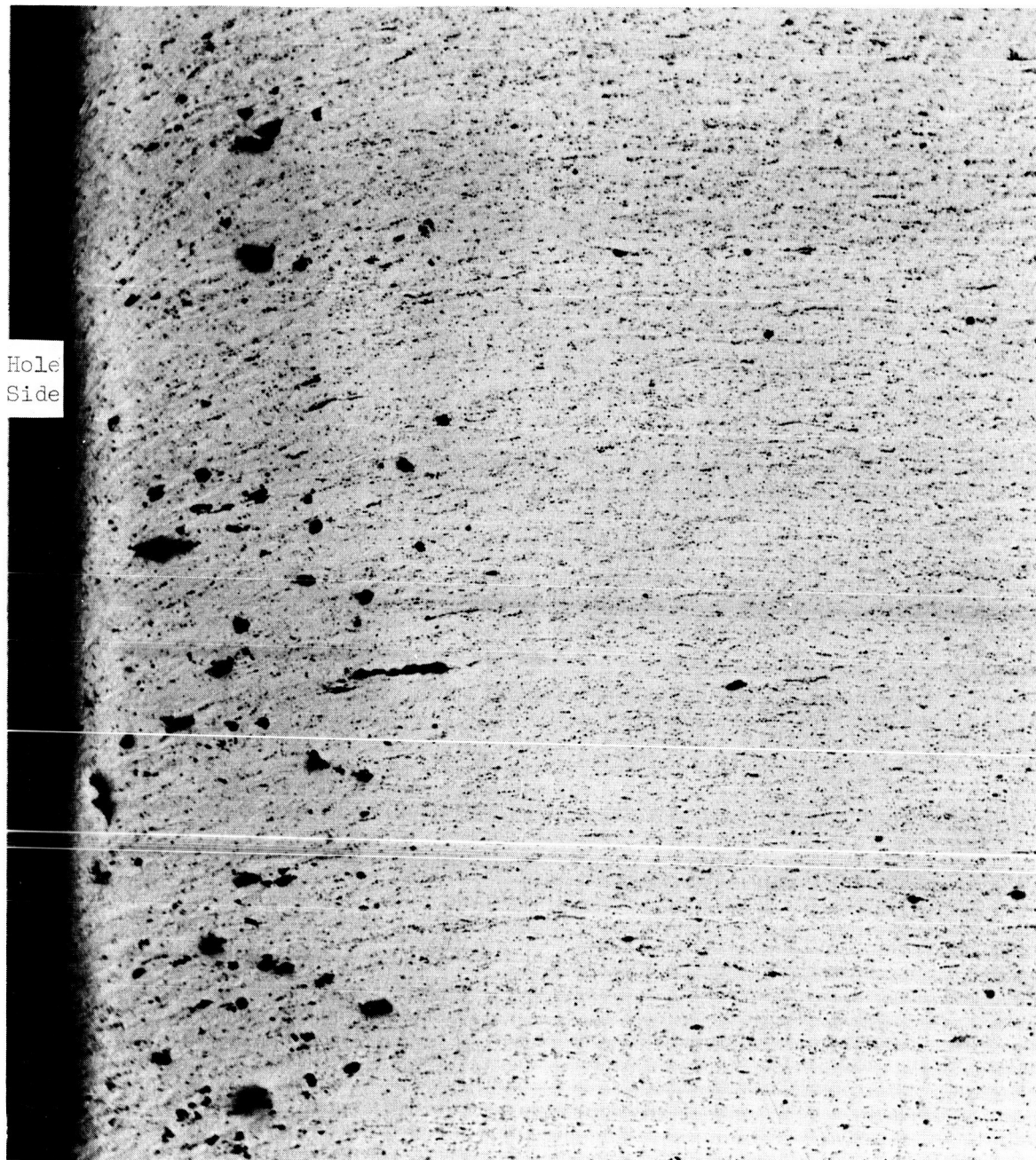
Figure 2-11 Punched hole cross-section. Note grain pull-out (porosity) & lines of basal plane deformation. (144X)
