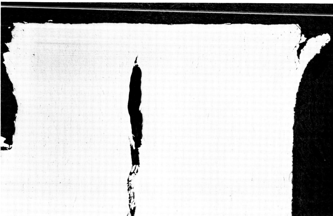
Figure 2-38 Cross-section through hole drilled with improperly sharpened drill - unetched. (85X)
