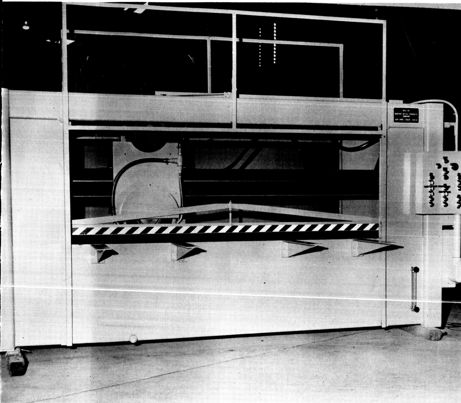
Figure 2-42 Large capacity precision abrasive cut-off saw.
