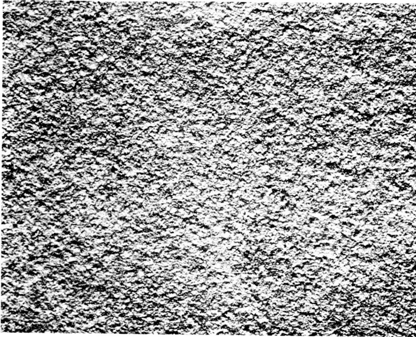
Figure 2-85 Macrograph of Area Chemically Milled with a 10% Solution of Ammonium Bifluoride (Specimen #6) (18X).
