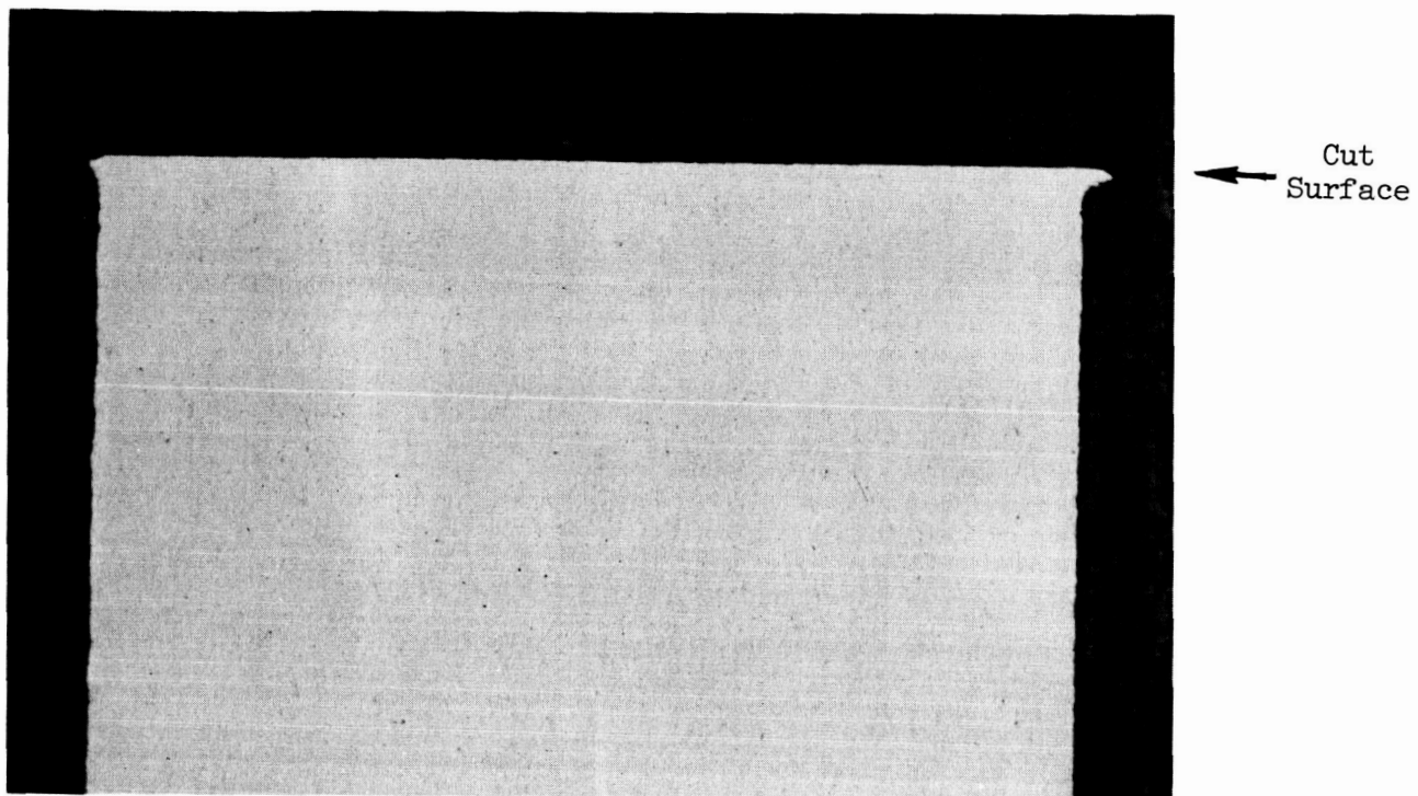
Figure 2-47 Cross-section of surface cut dry on abrasive wheel. Feed rate: 7.5 IPM at 8,240 SFM. (85X)
