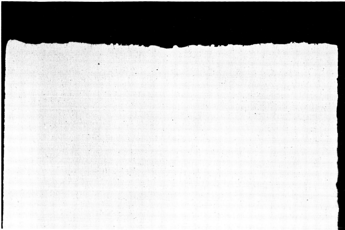
Figure 2-64 Cross-section of EDM finish cut at 8,000 CPS metal removal rate .38 cu. in./hr. (83X)
