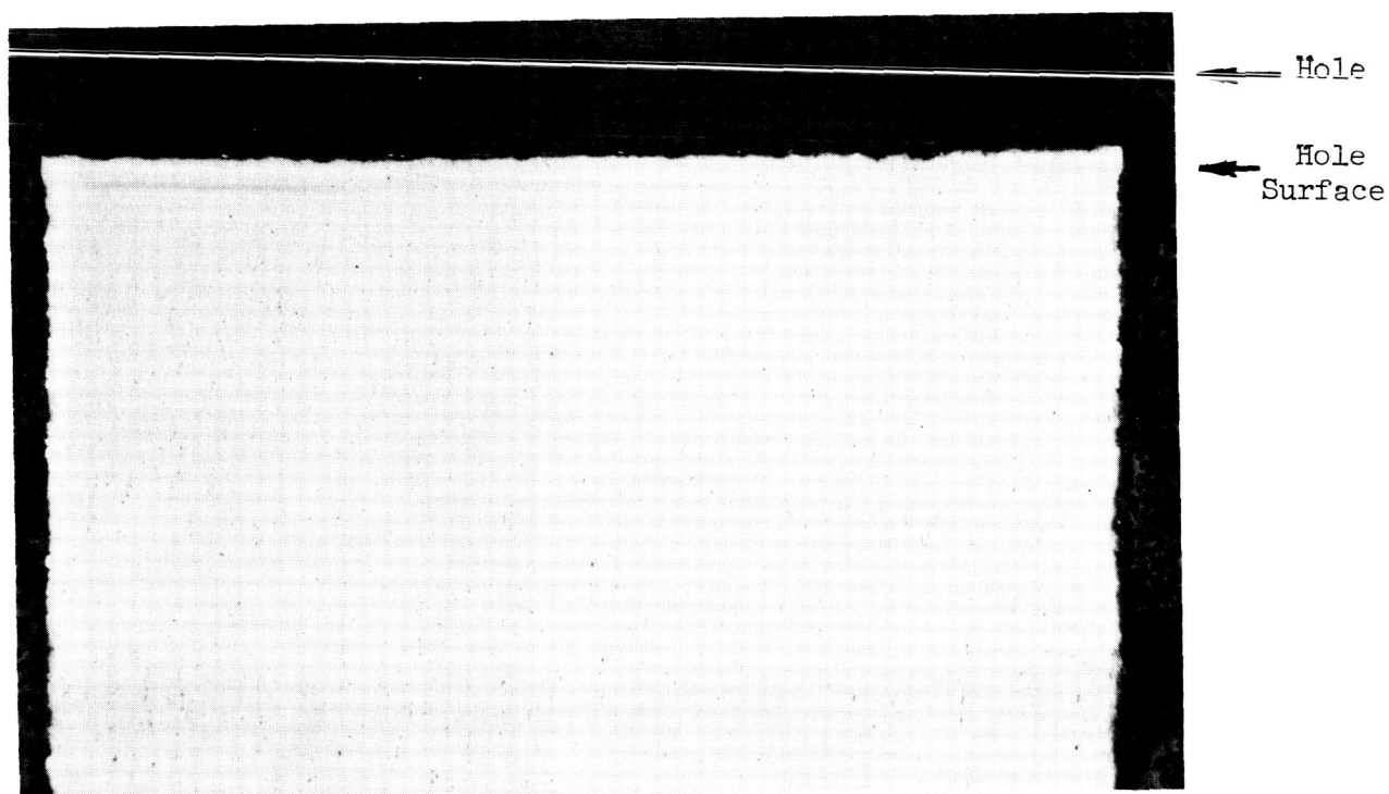
Figure 2-28 Cross-section through good hole using recommended procedures. (unetched) (85X)
