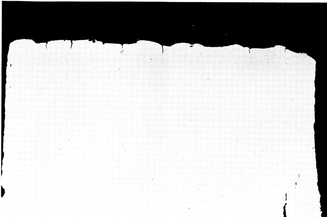
Figure 2-62 Cross-section of EDM finish cut at 2,000 CPS - metal removal rate 1.14 cu. in./hr. (83x)
