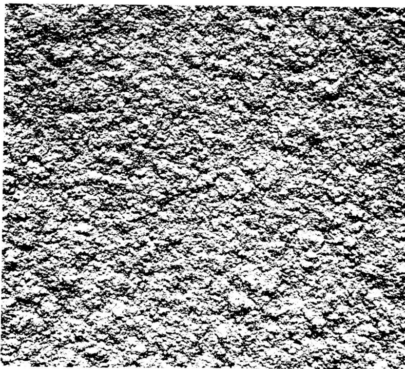
Figure 2-90 Macro photograph of Area Chemically Milled with a 30% Solution of Ammonium Bifluoride (Specimen #23) (18X).
