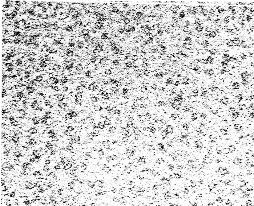
Figure 2-74 Macrograph of Area Chemically Milled with a 10% Solution of Sulfuric Acid (Specimen #12) (18X).
