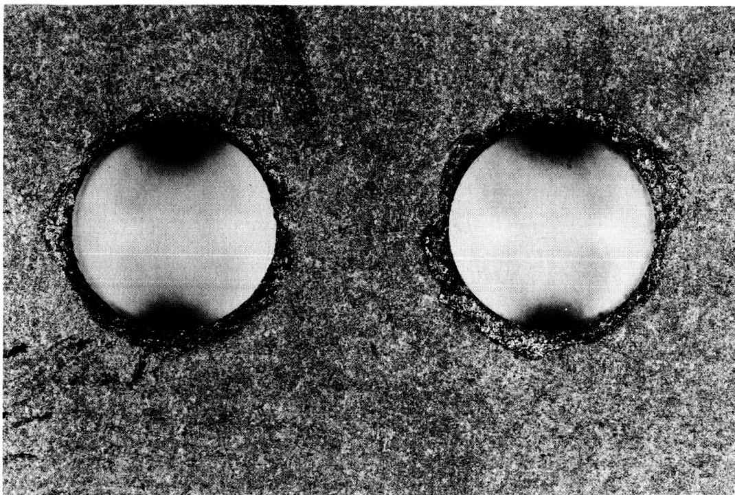
Figure 2-39 Holes drilled using excessive feed rates. Note spalling on exit side - unetched. (10X)
