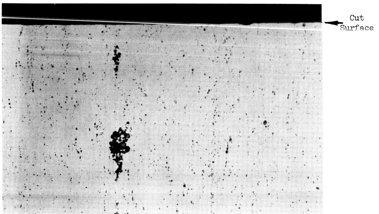
Figure 2-44 Cross-section of surface cut dry in abrasive wheel. Feed rate 4.0 IPM at 8,240 SFM. (500X) (Note large inclusion)
