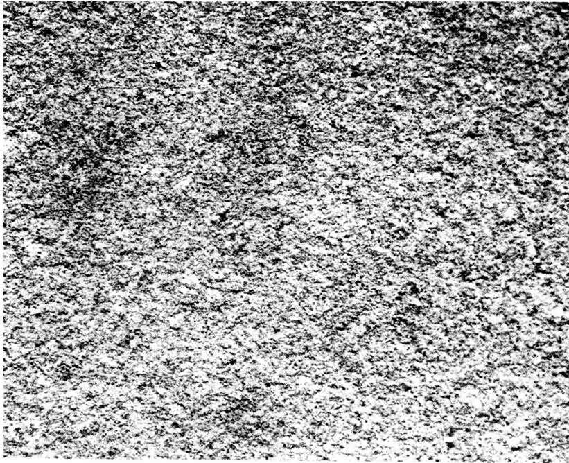
Figure 2-77 Macrograph of Area Chemically Milled with a 10% Solution of Sulfuric Acid (Specimen #21) (18X).
