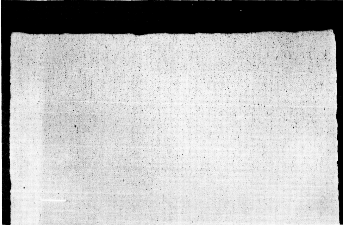
Figure 2-70 Cross-section of EDM finish cut at 32,000 CPS - metal removal rate .045 cu. in./hr. (83X)
