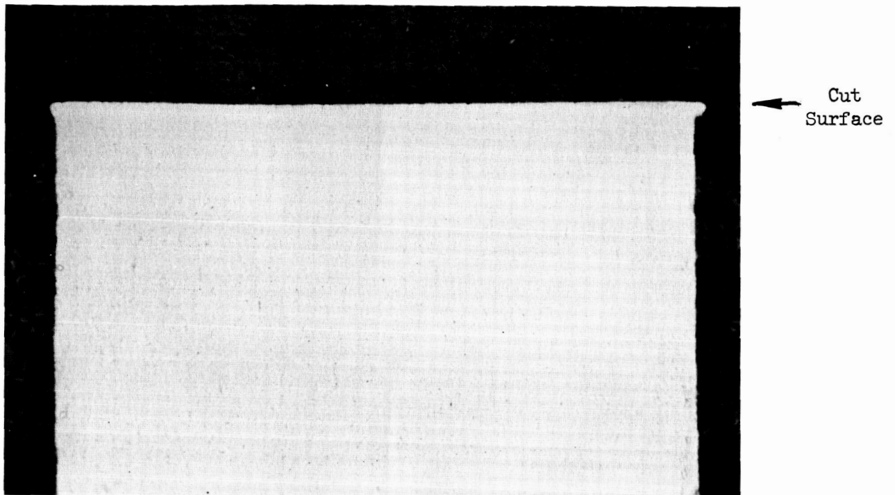
Figure 2-45 Cross-section of surface cut dry on abrasive wheel. Feed rate 6.0 IPM @ 8,240 SFM. (85X)
