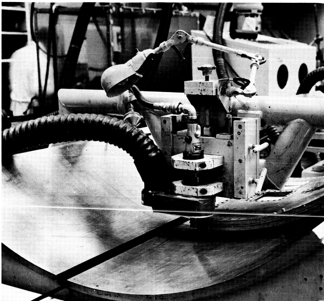
Figure 2-53 "Agena" panel in router fixture. Note substantial support structure and proximity of high velocity vacuum exhaust tube.
