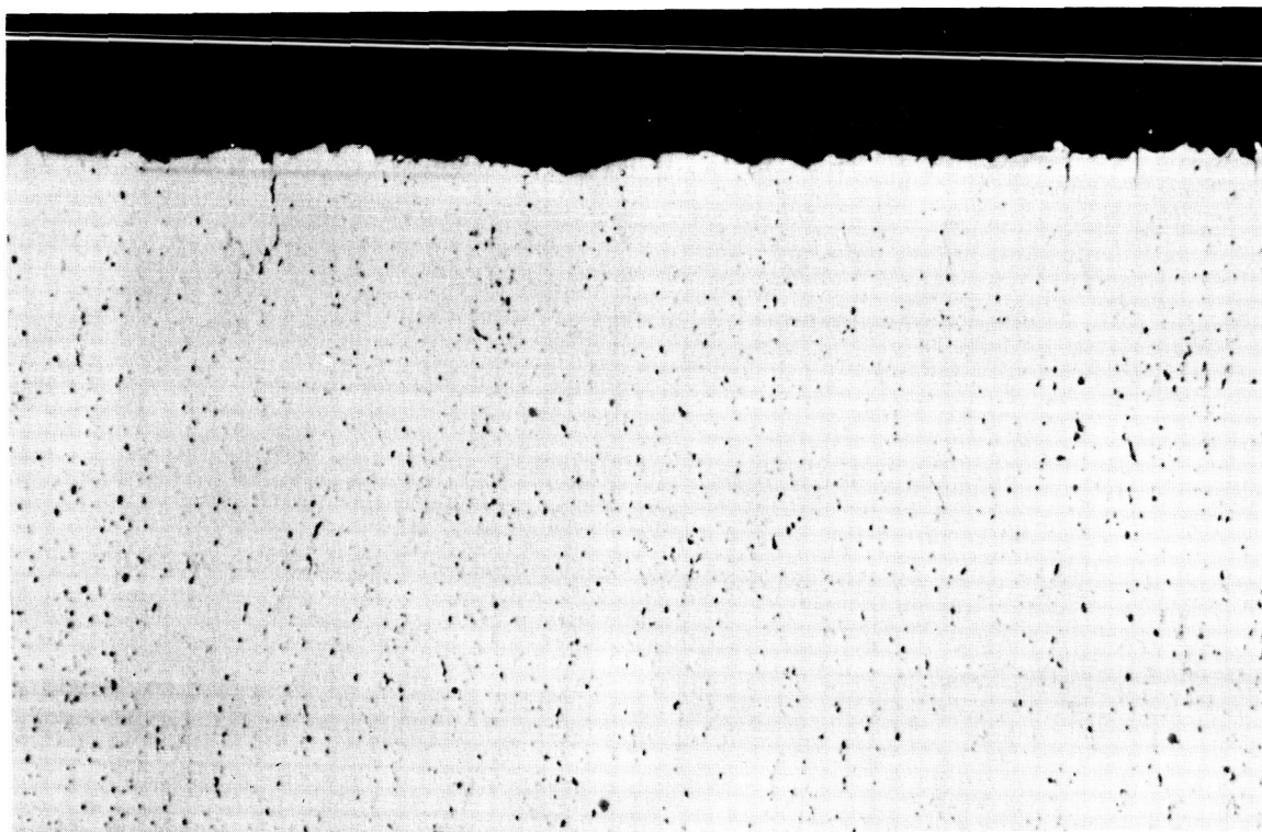
Figure 2-69 Cross-section of EDM finish cut at 130,000 CPS - metal removal rate .125 cu. in./hr. (500X)
