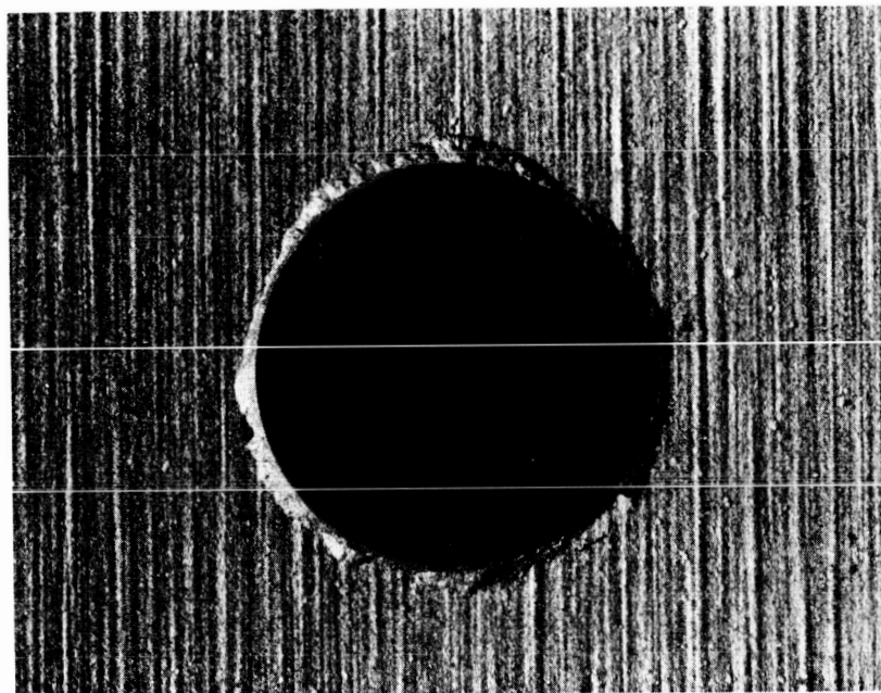
Figure 2-5 Break-out (spalling) of exit side of improperly drilled hole. (10X)
