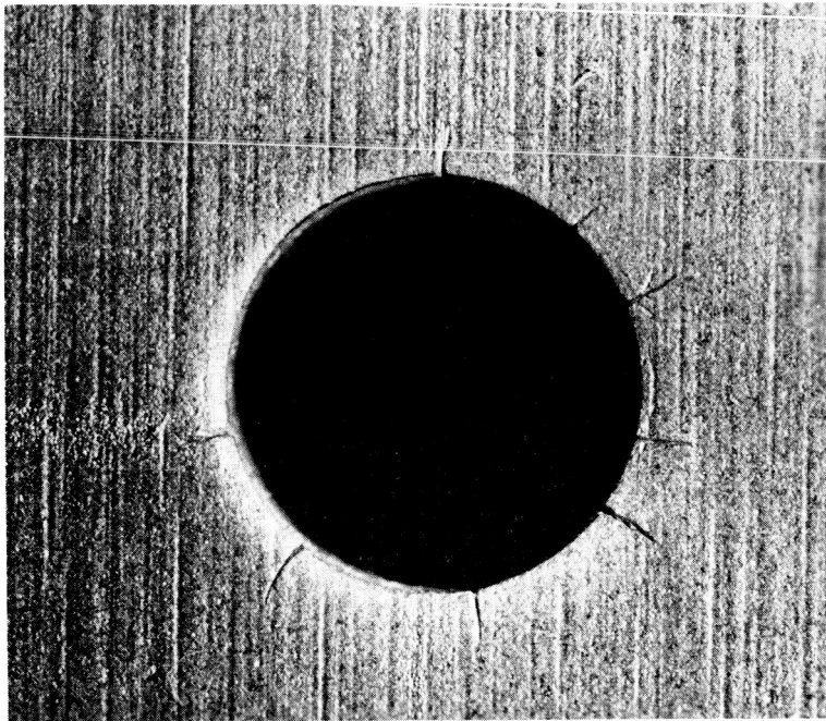
Figure 2-4 Radial cracking around punched & etched hole. - Entrance side. (10X)
