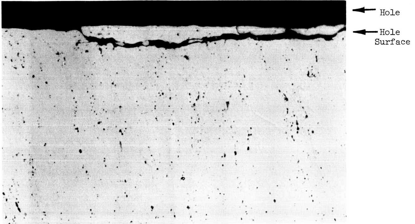
Figure 2-41 Cross-section of hole drilled at excessive feed rate. Note chipping on flat portion of hole surface. unetched (500X)
