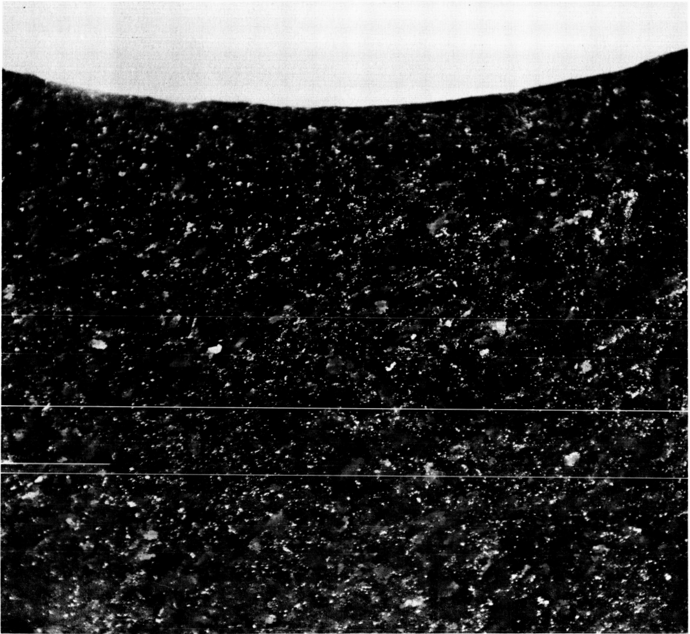
Figure 2-7 Drilled hole in 0.060 sheet - entrance surface. Representative of all drilled holes. (144X)
