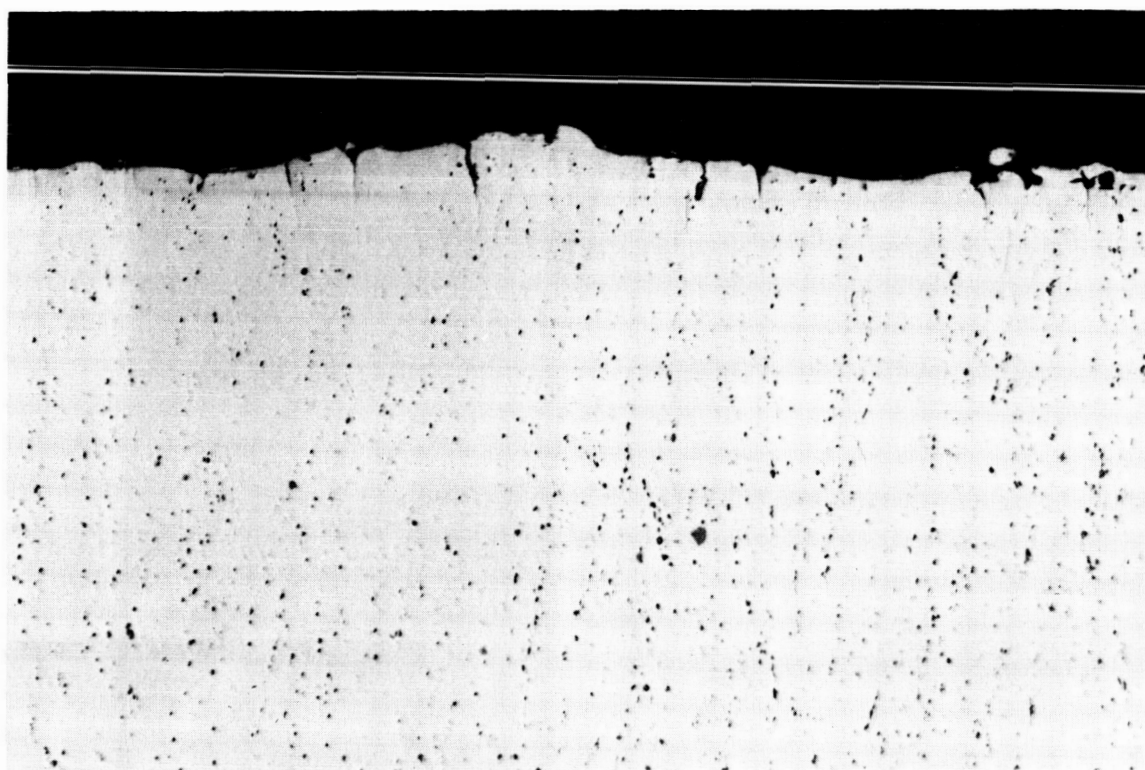
Figure 2-61 Cross-section of EDM roughing cut. (500X)
