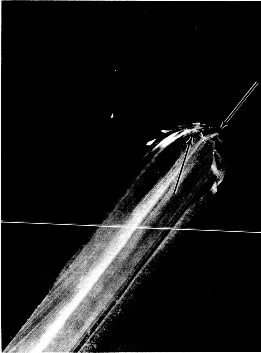
Figure 2-25 Enlarged view of primary cutting edge & length & depth of gash for cross-over of point.
