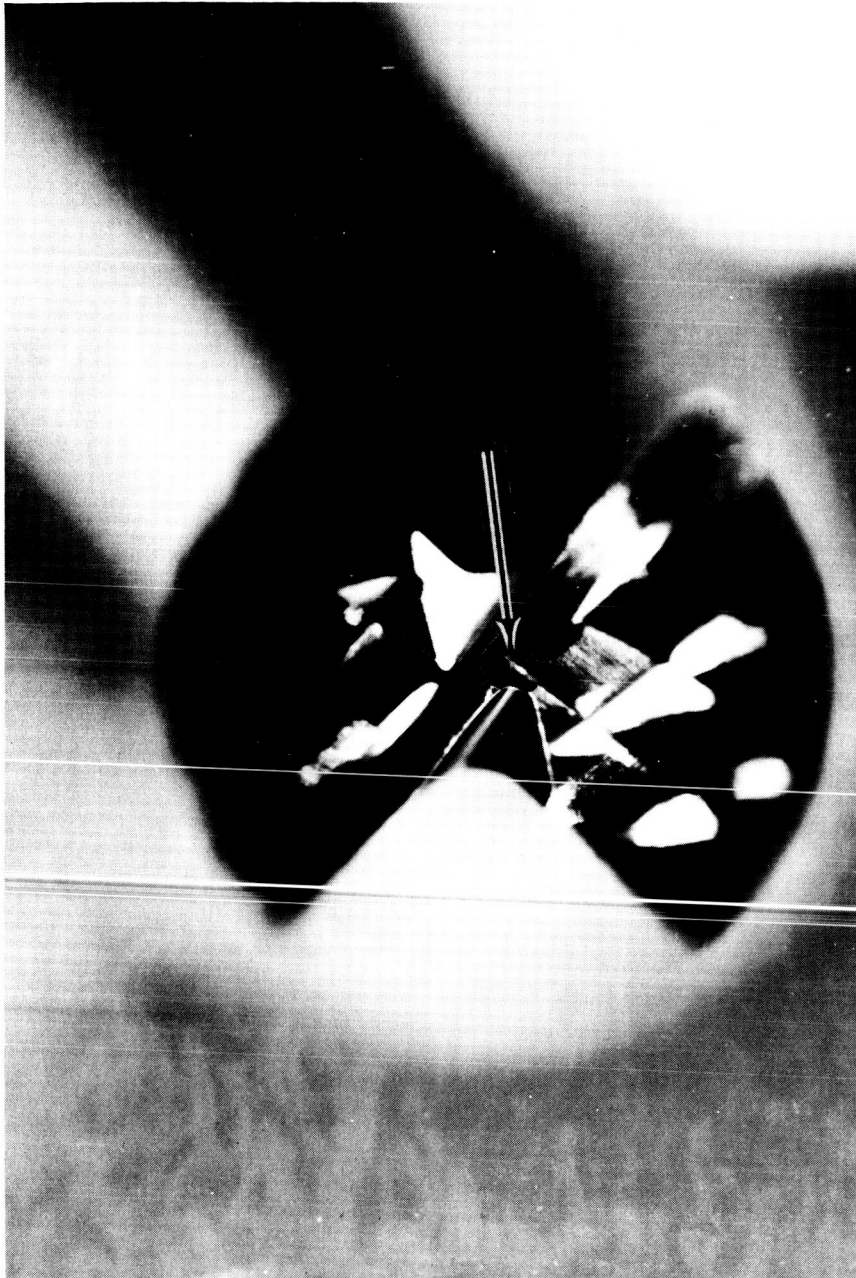
Figure 2-22 Enlarged microscopic view of burr drill point showing gash progressed into primary land near chisel point & in such a manner to weaken trailing burr to chisel fracture.
