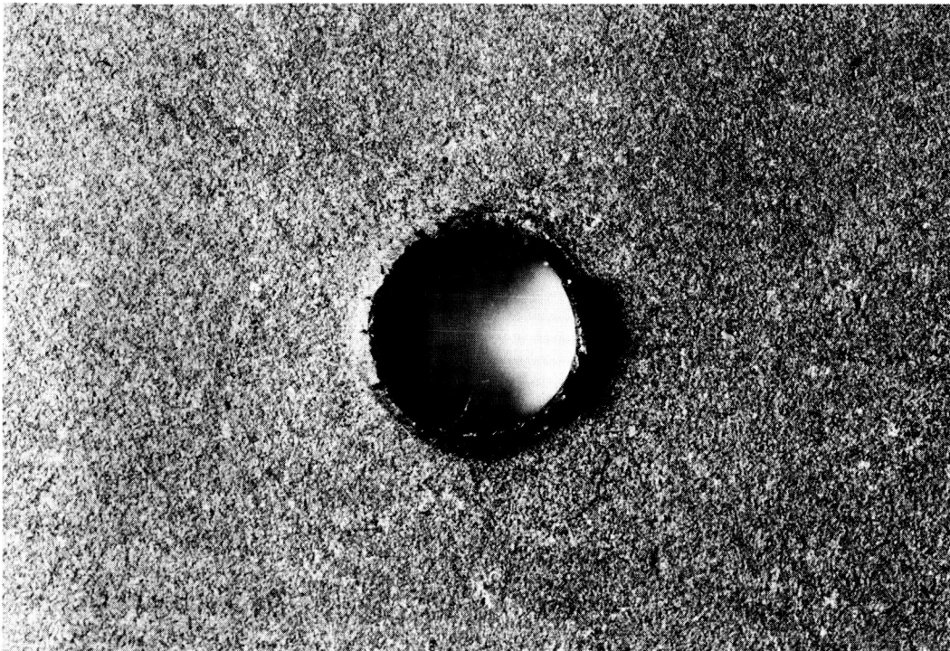
Figure 2-37 Hole drilled with improperly sharpened drill. Note heavy burr on exit side - unetched. (10X)
