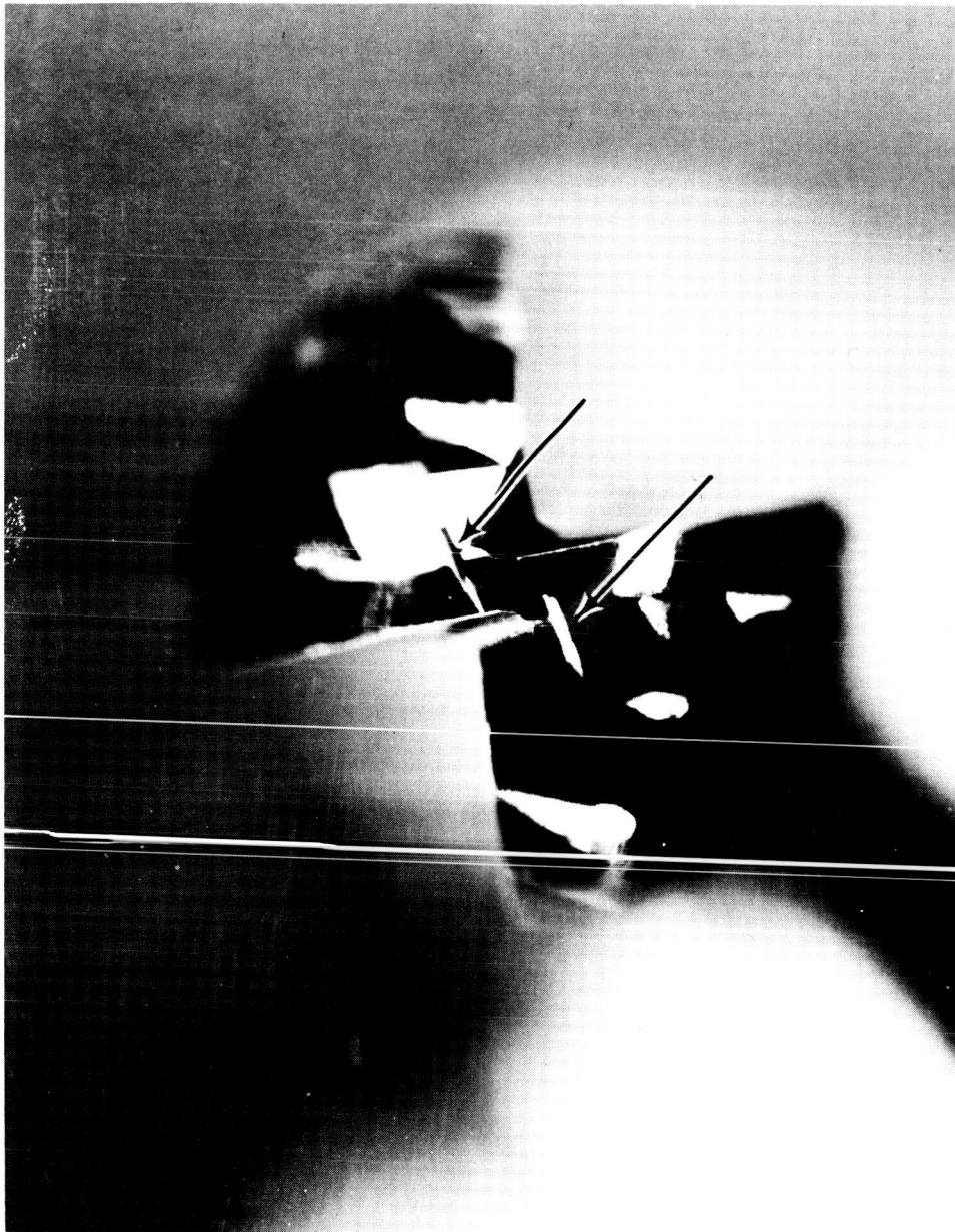
Figure 2-21 Enlarged microscopic view of burr drill point showing gashes allowed to progress into both primary lands
