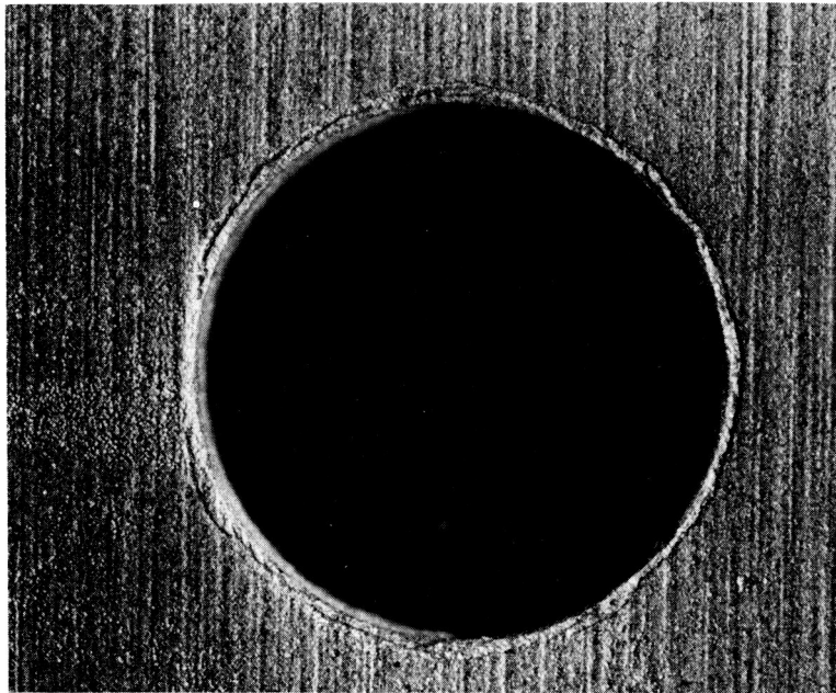
Figure 2-3 Circumferential cracking around punched & etched hole. - Entrance side. (10X)
