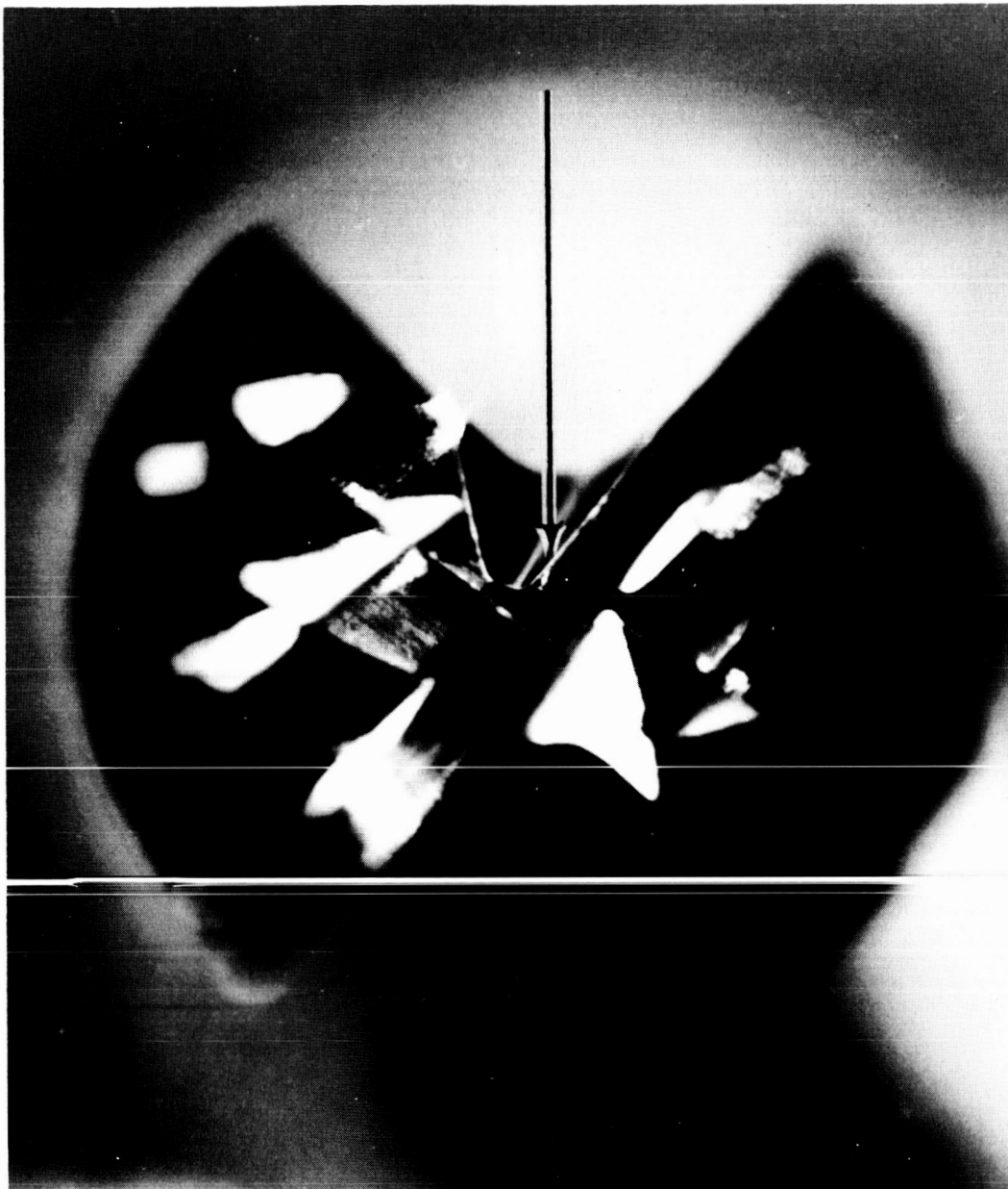
Figure 2-18 Enlarged microscopic view of burr drill point showing flat spot at chisel point progressing along right primary cutting edge.
