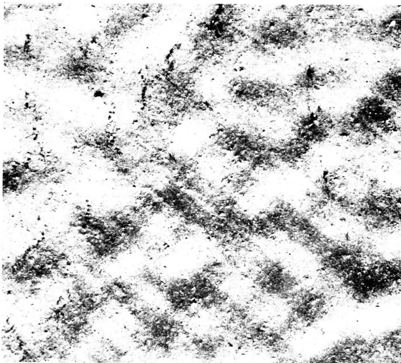
Figure 2-98 Macrograph of Area Chemically Milled with a 5 Parts (Vol.) Phosphoric Acid - 2 Parts (Vol.) Sulfuric Acid - 5 Parts (Vol.) Water Solution (Specimen #8) (18X).
