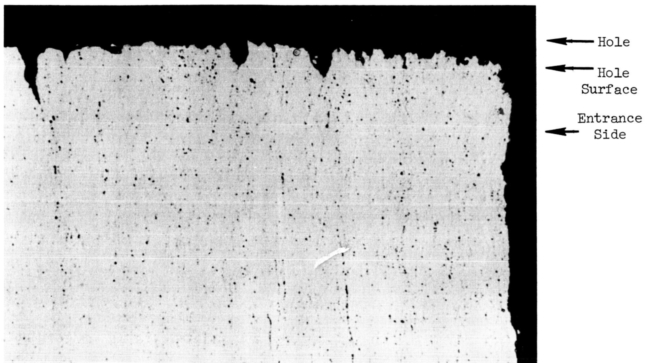
Figure 2-36 Cross-section of hole drilled with dull drill at high magnification - unetched. (500X)
