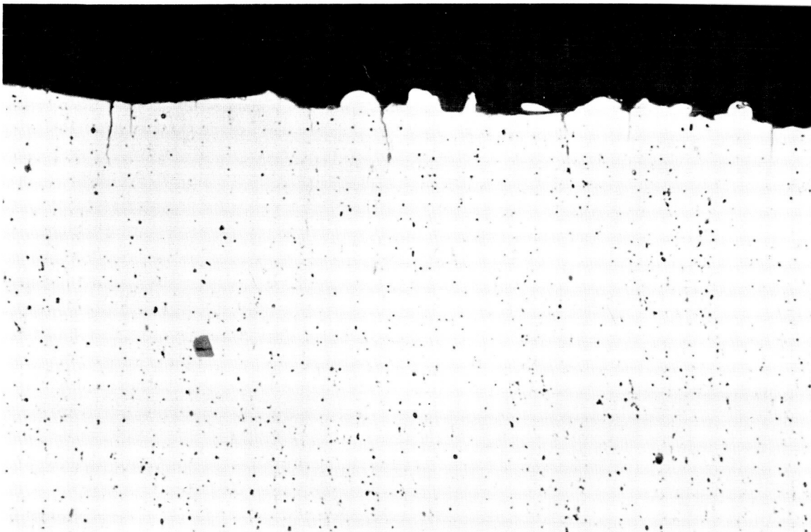
Figure 2-65 Cross-section of EDM finish cut at 8,000 CPS - metal removal rate .38 cu. in./hr. (500X)
