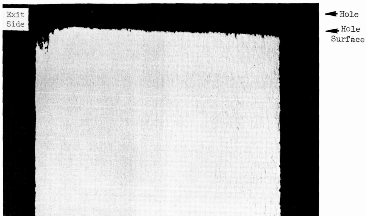
Figure 2-34 Cross-section of hole drilled with dull drill (unetched). (85X)
