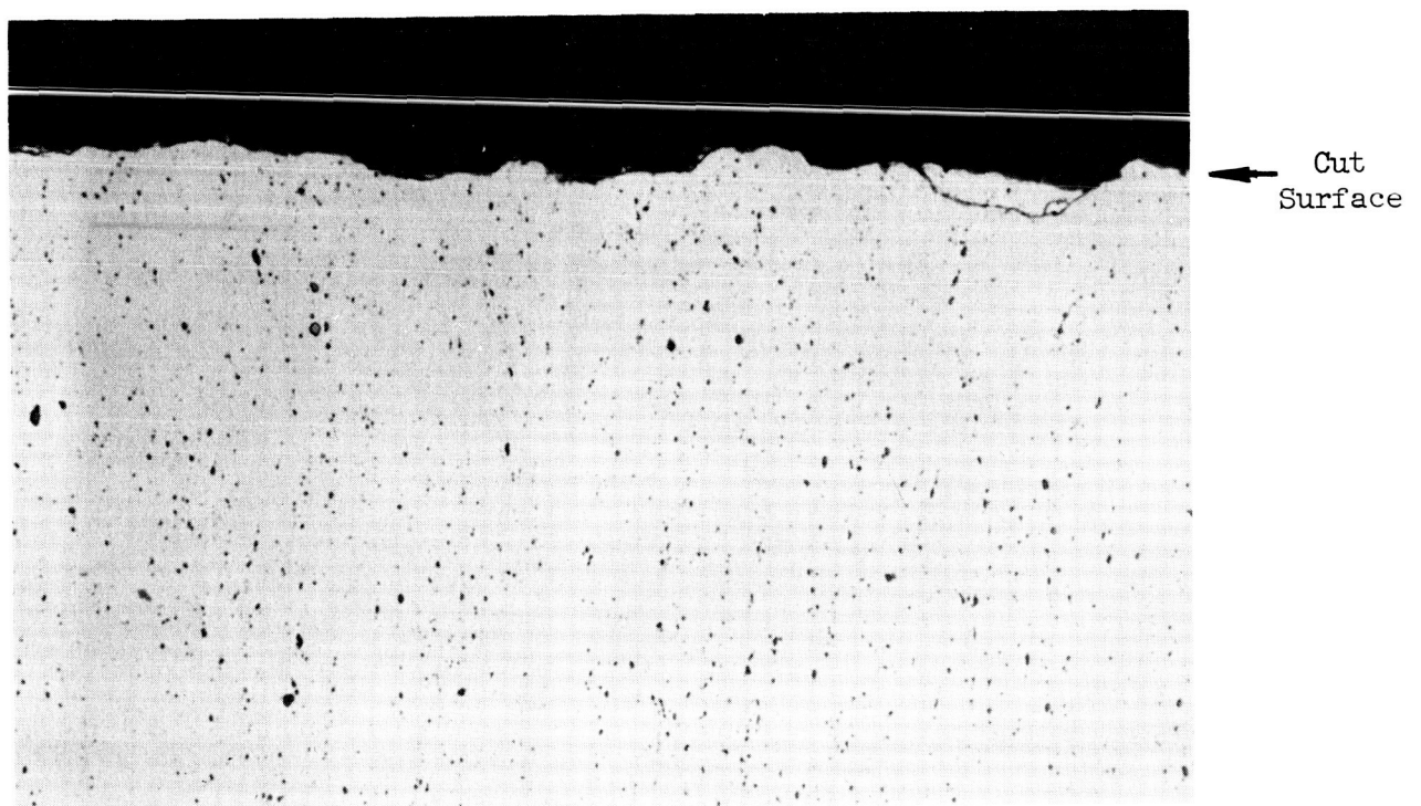
Figure 2-56 Cross-section of router cut surface.(500X)
