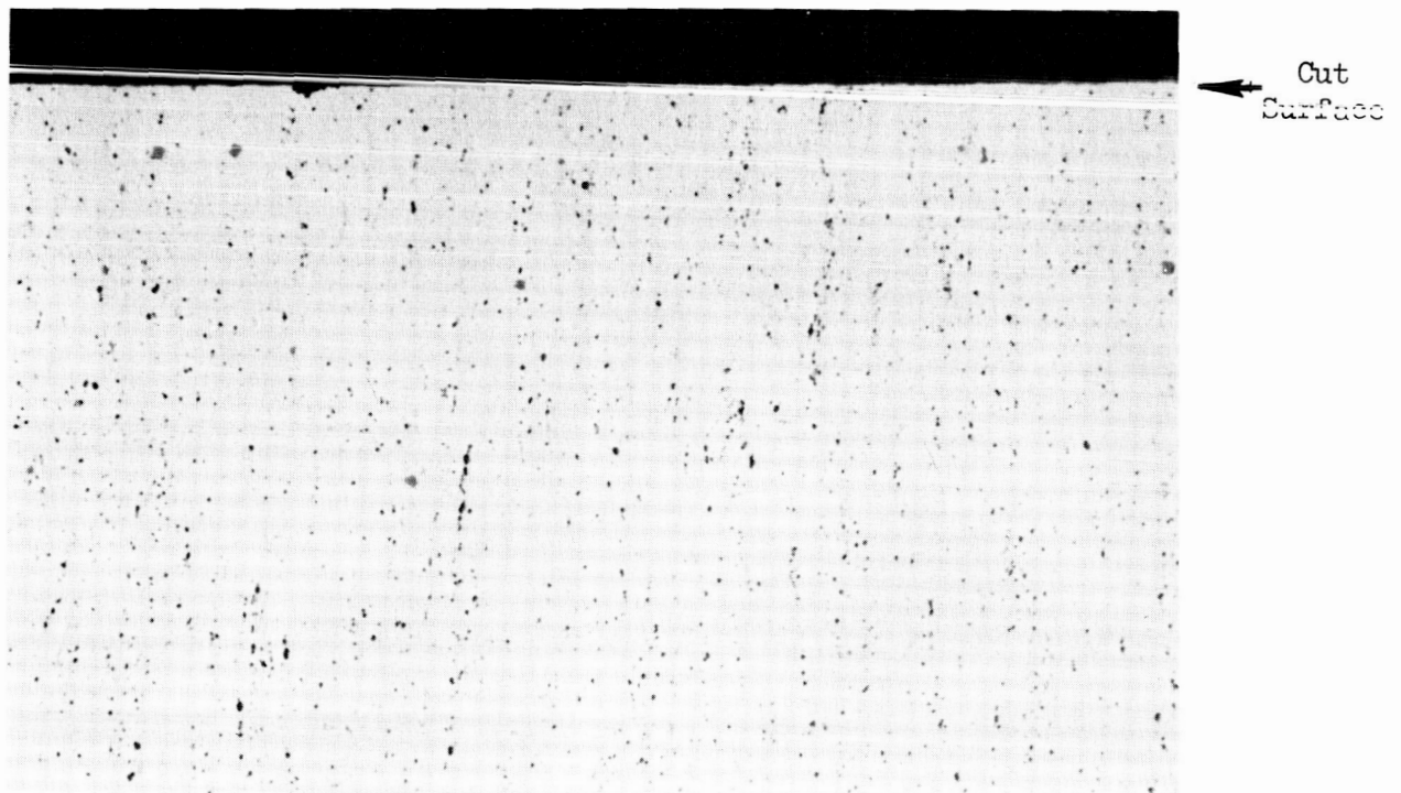
Figure 2-46 Cross-section of surface cut dry on abrasive wheel. Feed rate: 6.0 IPM at 8,240 SFM (500X)
