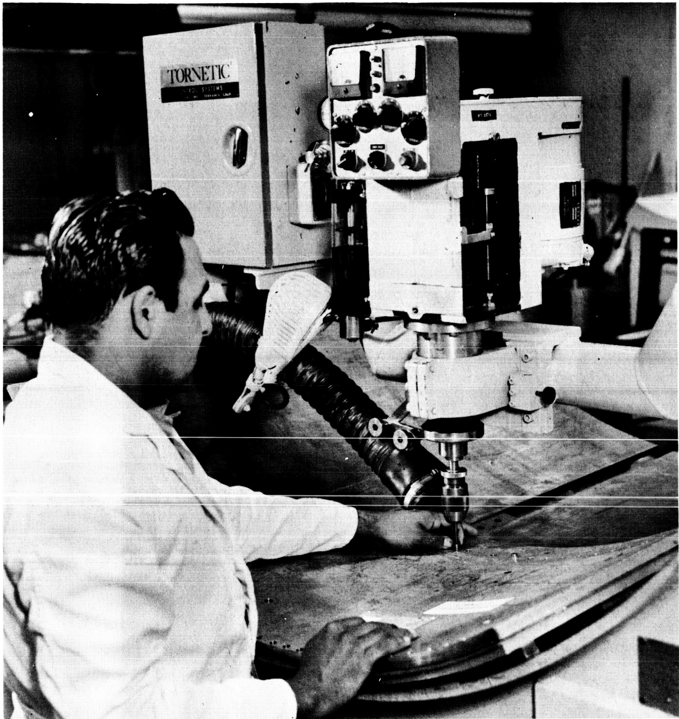
Figure 2-12 "Agena" panel being drilled using "Tornetic" control head - Note substantial fixturing and proximity of high velocity vacuum exhaust tube.
