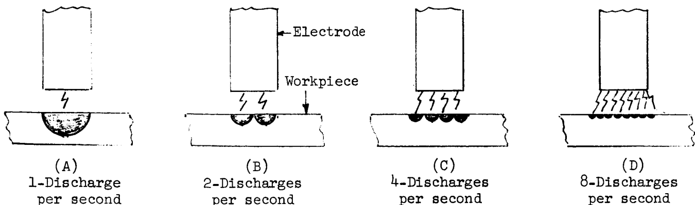
Figure 2-58: Relationship Between Surface Finish and Discharge Frequency.
