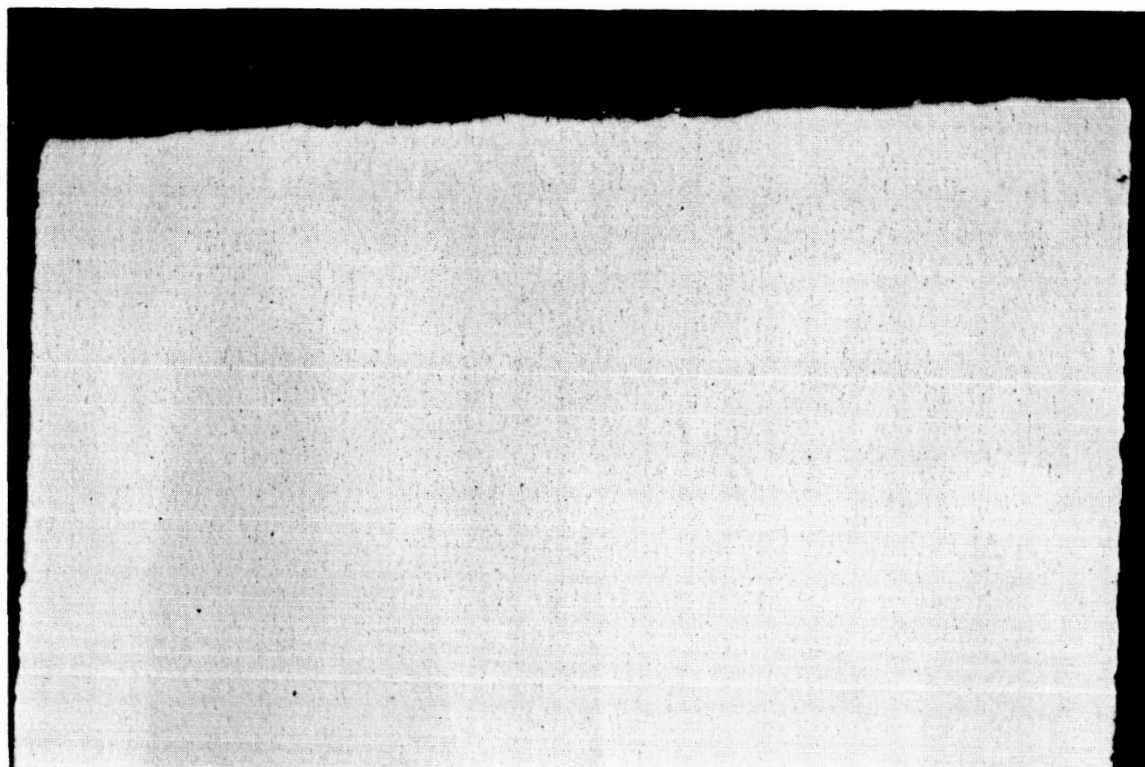
Figure 2-60 Cross-section of EDM roughing cut. (83X)
