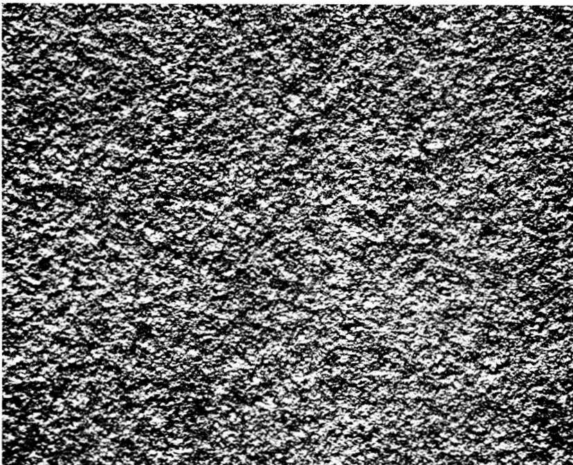
Figure 2-82 Macrograph of Area Chemically Milled with a 7.5% Solution of Ammonium Bifluoride (Specimen #15) (18X).
