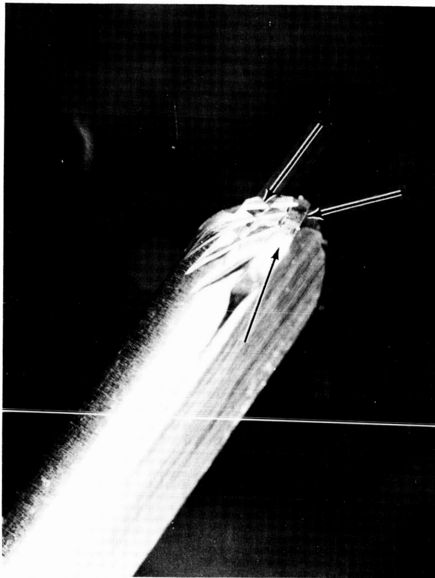
Figure 2-26 Enlarged view of angles of burr points, primary cutting edge and angle of relief of primary land.
