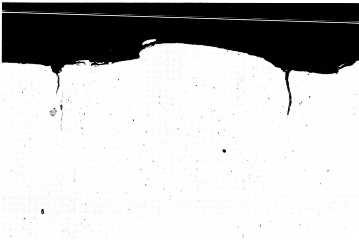
Figure 2-63 Cross-section of EDM finish cut at 2,000 CPS - metal removal rate 1.14 cu. in./hr. (500x)
