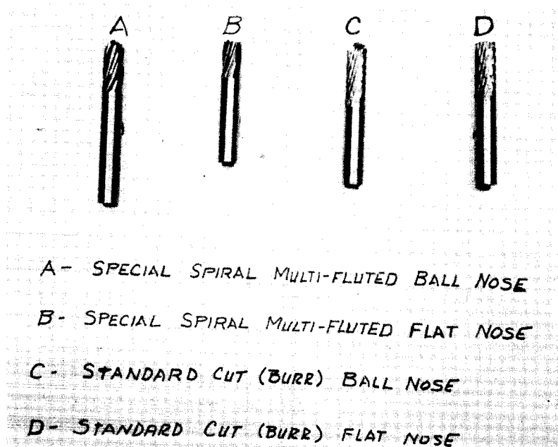
Figure 2-54 Types of cutters used in routing beryllium sheet.
