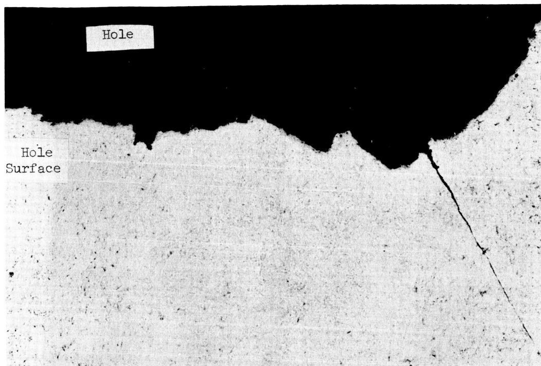
Figure 2-32 Hole drilled with dull drill. Surface of sheet showing radial crack emanating from rough surface of hole - unetched. (85X)
