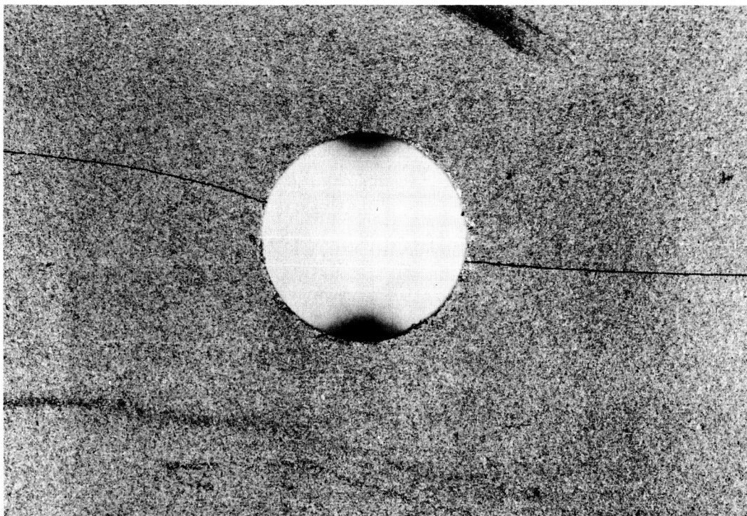
Figure 2-30 Hole drilled with dull drill showing radial cracking (unetched) (10X)
