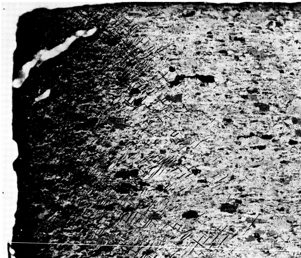
Figure 2-9 Cross-section through punched hole showing extent of surface damage & twinning. (144X)
