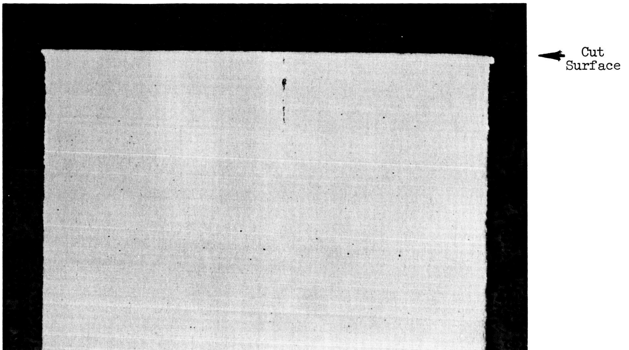
Figure 2-43 Cross-section of surface cut dry on abrasive wheel. Feed rate 4.0 IPM @ 8,240 SFM. (85X)
