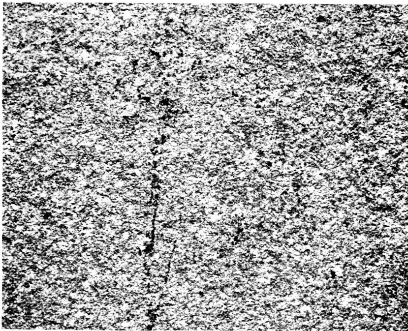
Figure 2-78 Macrograph of Area Chemically Milled with a 7.5% Solution of Sulfuric Acid (Specimen #16) (18X).
