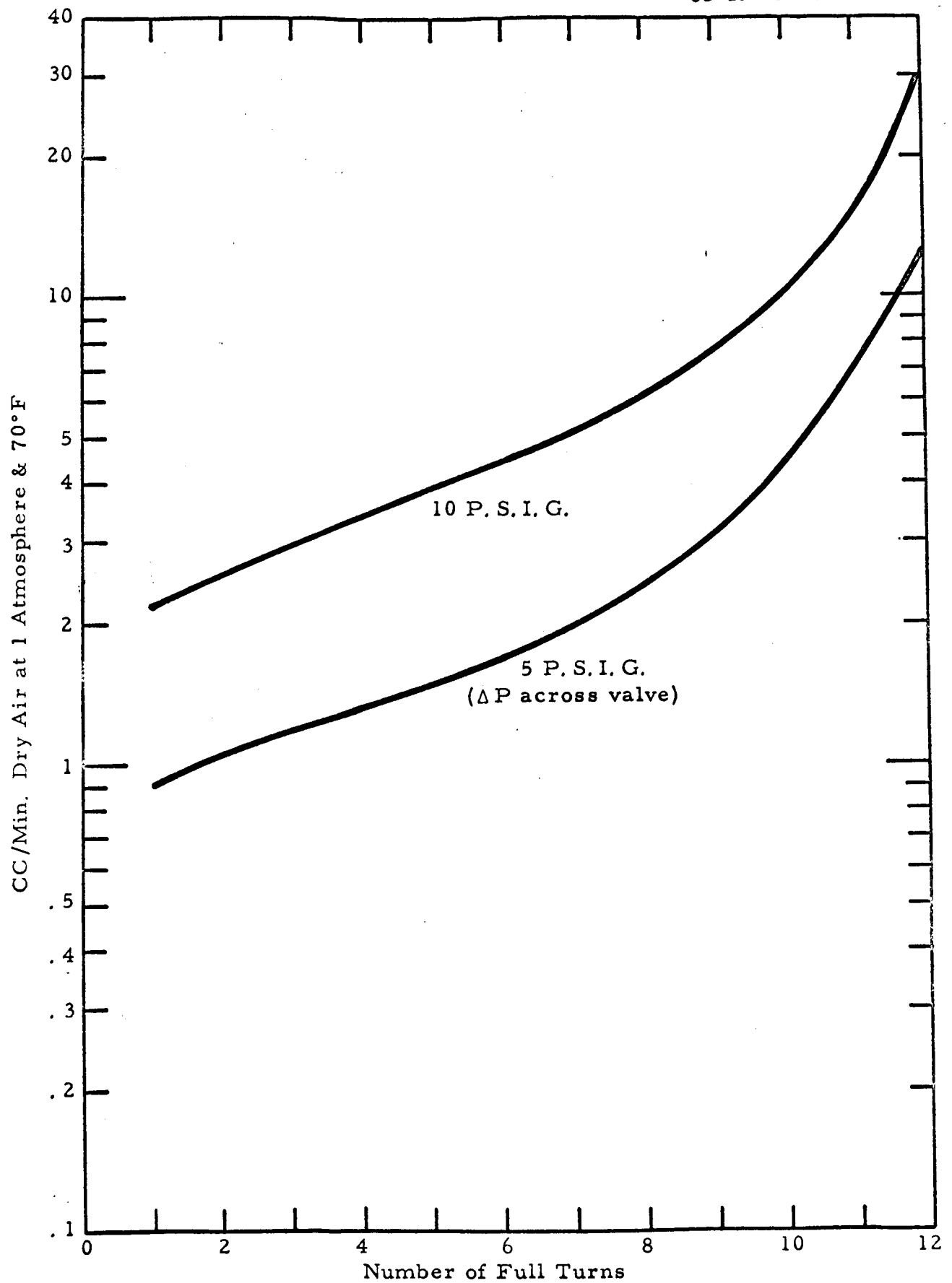
Figure II-4. Characteristic of Microflow Valve.
