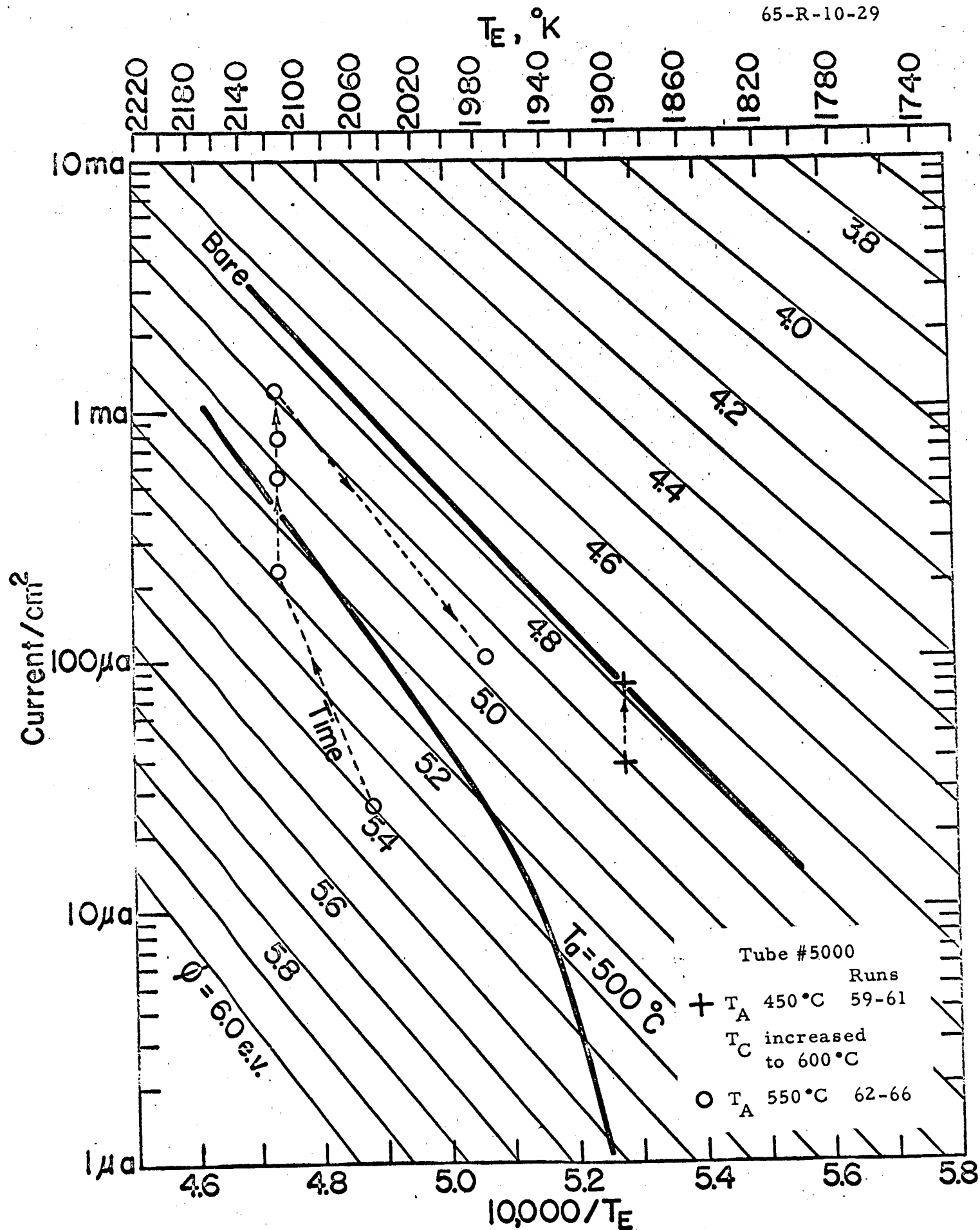
Figure V-5. Emitter Work Function with Additive as a Function of Emitter Temperature at Higher Additive Pressure.
