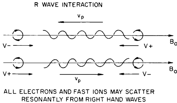
Fig. XI-30. Right-hand wave interaction.
