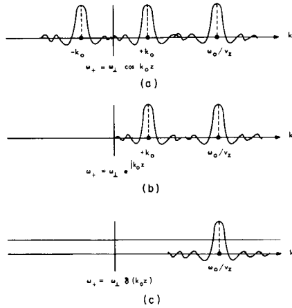
Fig. XI-31. Diffusion coefficient factors in k space.
