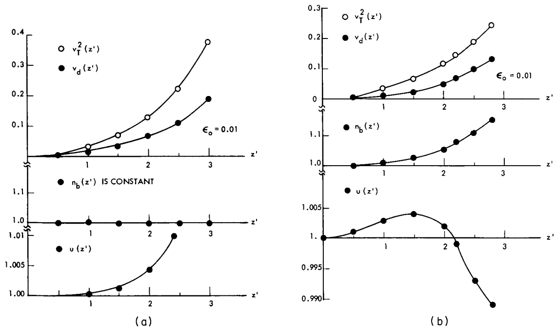
Fig. XI-24. Normalized thermal velocity v_T , velocity decrease of the beam v_d , beam density n_b , and beam energy density u as functions of z' (a) in the limit f_0(v_z) \rightarrow 0 unless v_z \approx v_0 and (b) computed exactly by numerical integration of Eq. 21.
