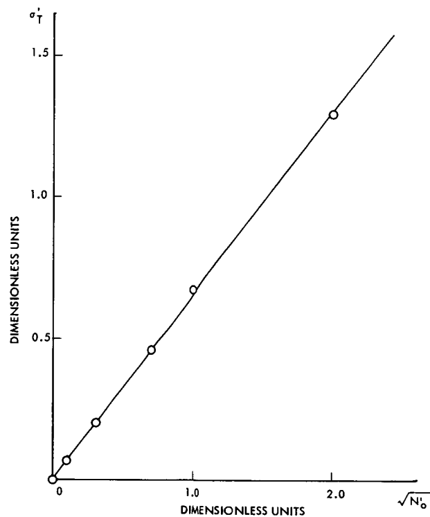
Fig. XIII-10. Jitter standard deviation \sigma_T^j vs \sqrt{N_O^j} (in dimensionless units).
