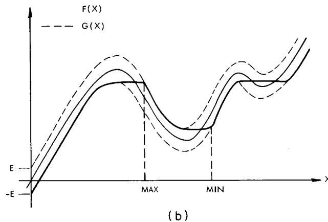
Fig. XV-13. Hysteresis smoothing.
