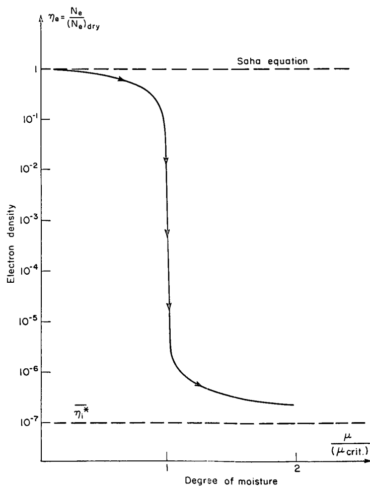
Fig. XII-20. Typical electron density variation with degree of moisture at constant electron temperature and mean drop size.
