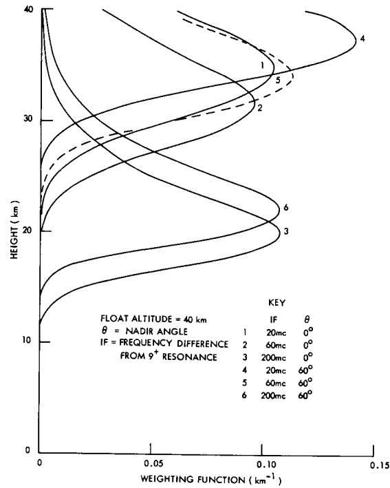
Fig. III-1. Weighting functions.
