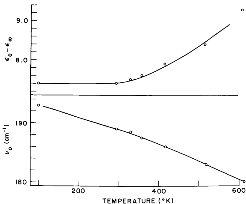
Fig. IV-2. Temperature dependence of the infrared eigenfrequency \omega_0 and the oscillator strength (\epsilon_0 - \epsilon_\infty) of \text{Mg}_2\text{Sn} .
