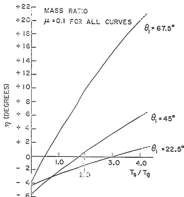
Fig. VII-6. Characteristics of the approximate analysis: The temperature dependence of \eta , the angular deviation from the specular direction, for several values of the angle of incidence, \theta_o .
