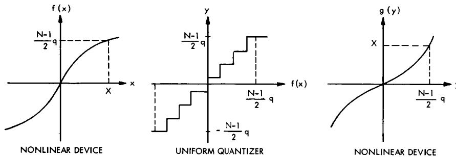
Fig. XIII-6. Nonuniform quantizer.
