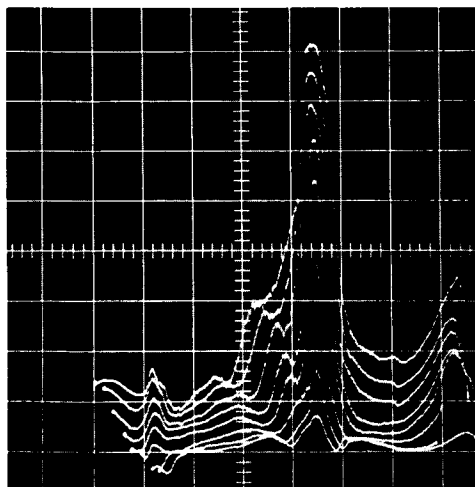
Fig. IX-6. Resonance curves at different applied voltages. Peak-to-peak applied voltage of 600 – 425 volts in steps of 25 volts. Hydrogen pressure, 18 \mu .
