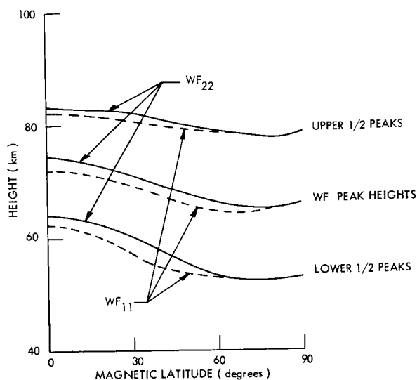
Fig. III-7. Height variation of weighting-function peaks.
