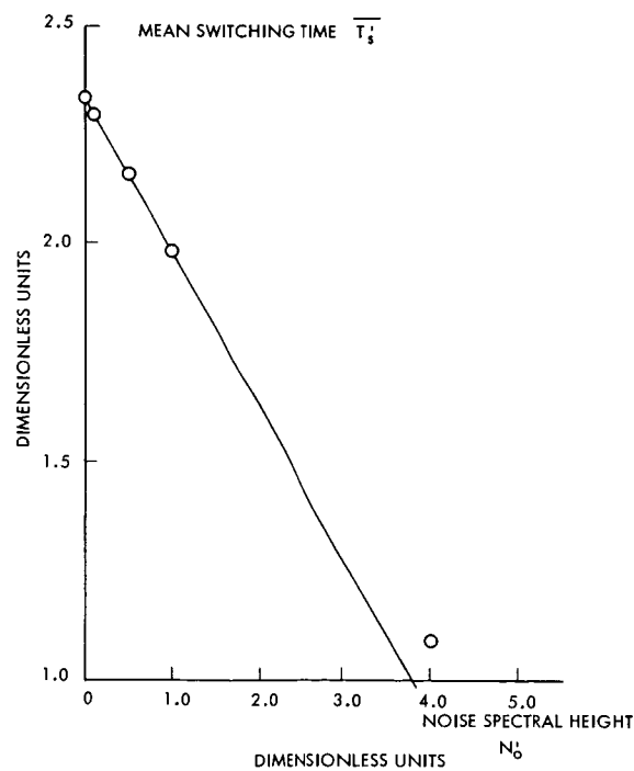
Fig. XIII-11. Mean switching time \overline{T_s^j} vs N_O^j (in dimensionless units).
