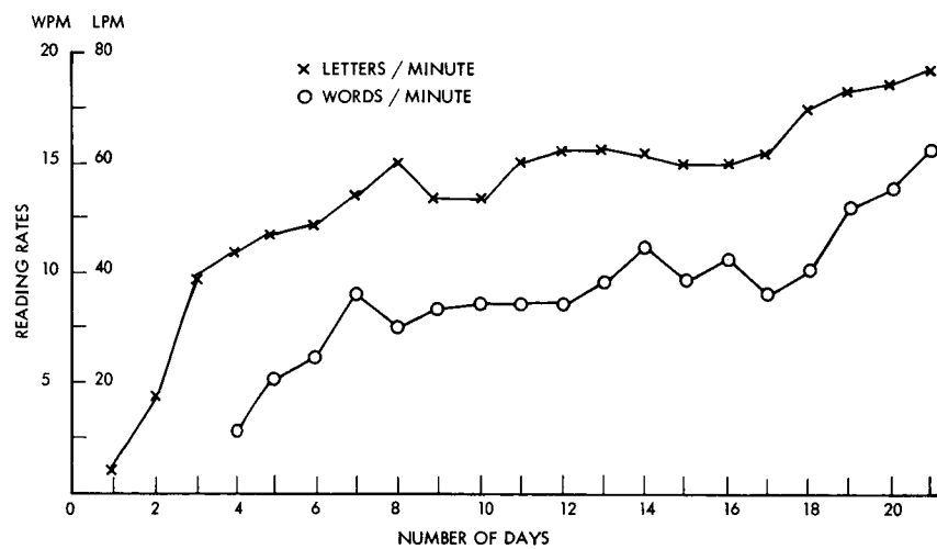
Fig. XV-19. Reading rates—Team 1.
