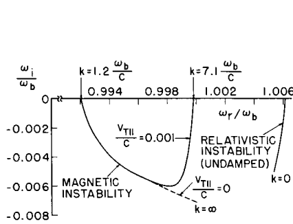
Fig. XI-6. Zero drift real k locus for finite temperature.
