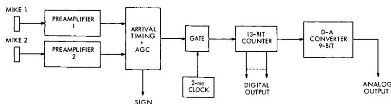
Fig. XV-11. System diagram.
