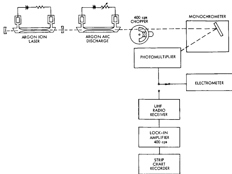
Fig. V-2. Experimental arrangement.
