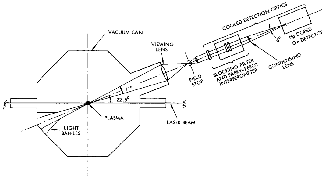
Fig. XI-33. Detection optics.
