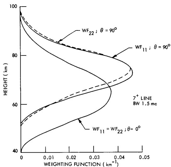
Fig. III-6. Weighting functions, 7^+ line, 1.5-Mc bandwidth.
