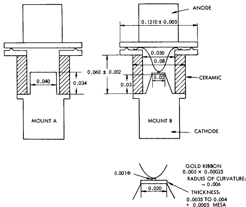
Fig. III-11. Diode mounts.
