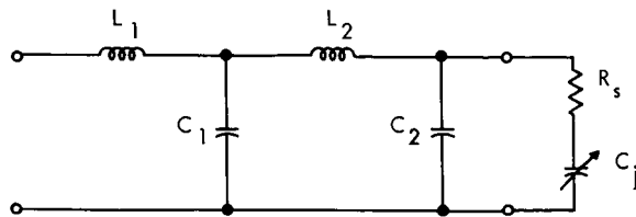
Fig. III-12. Double LC equivalent circuit.
