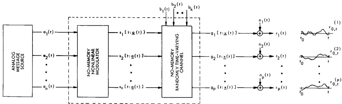
Fig. XIII-15. Communication model.
