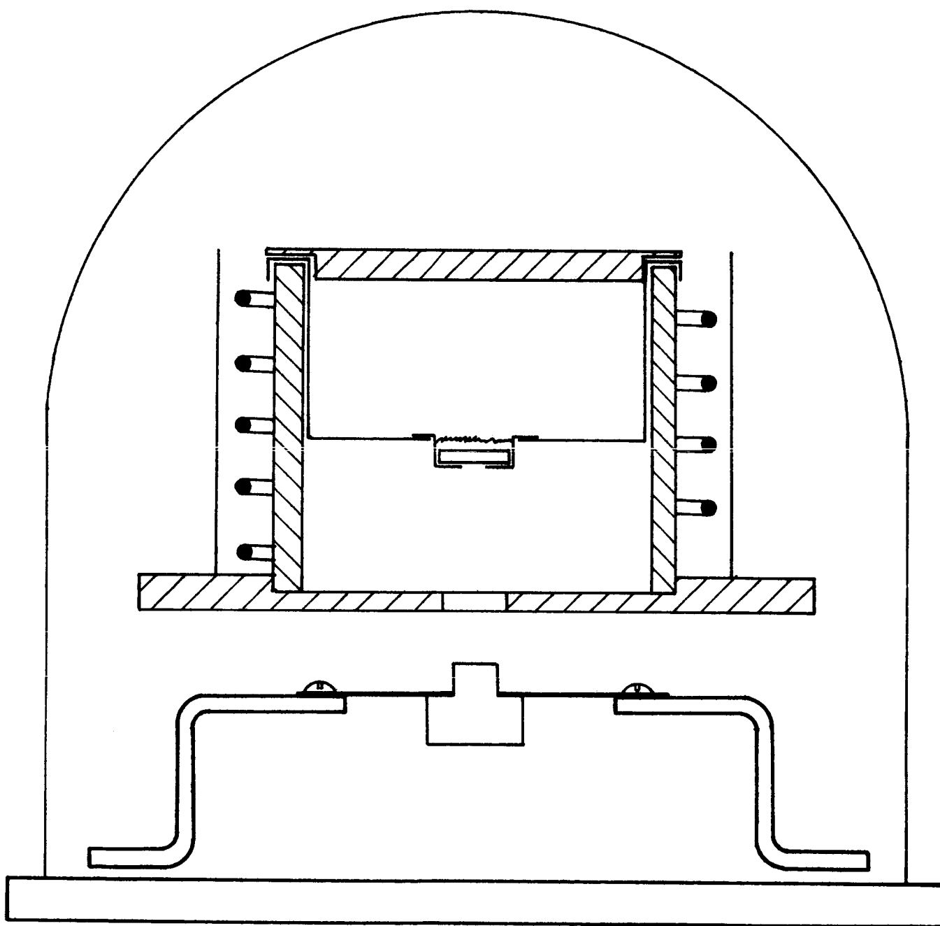
Fig. 14. Basic components of the thin-film transducer evaporating station.
