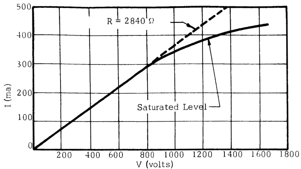
Fig. 20. V-I curve for a CdS sample showing current saturation.
