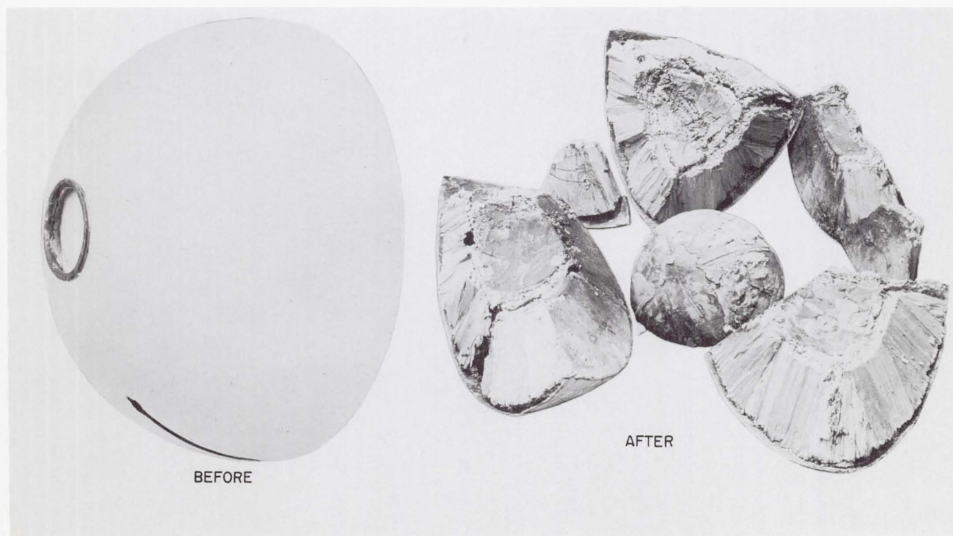
Fig. 12. Impact limiter segment removal test
