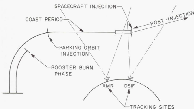
Fig. 1. Spacecraft flight sequence
