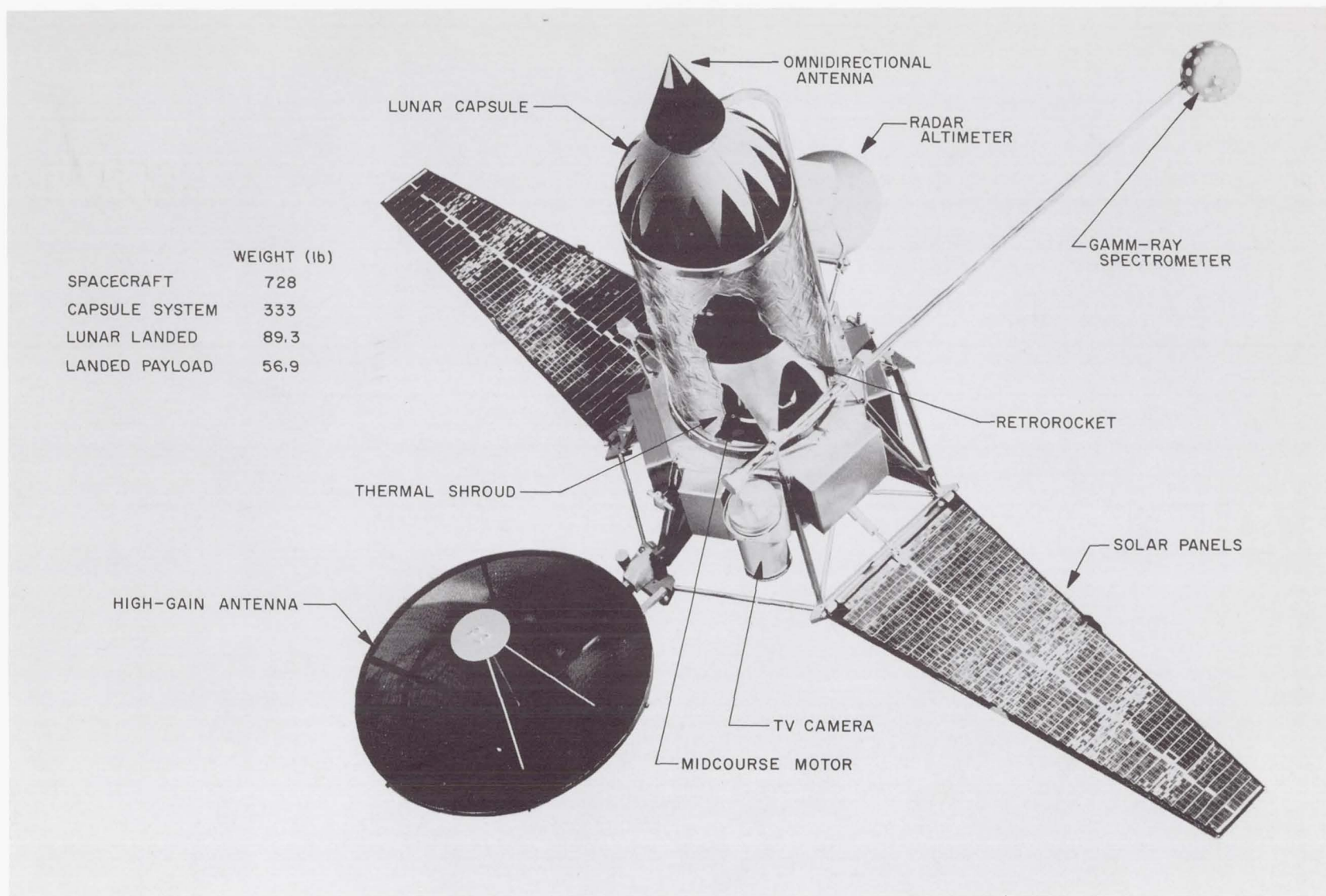
Fig. 8. Ranger spacecraft
