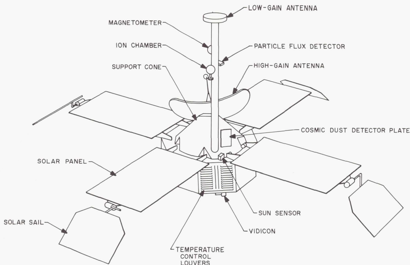
Fig. 3. Mariner spacecraft
