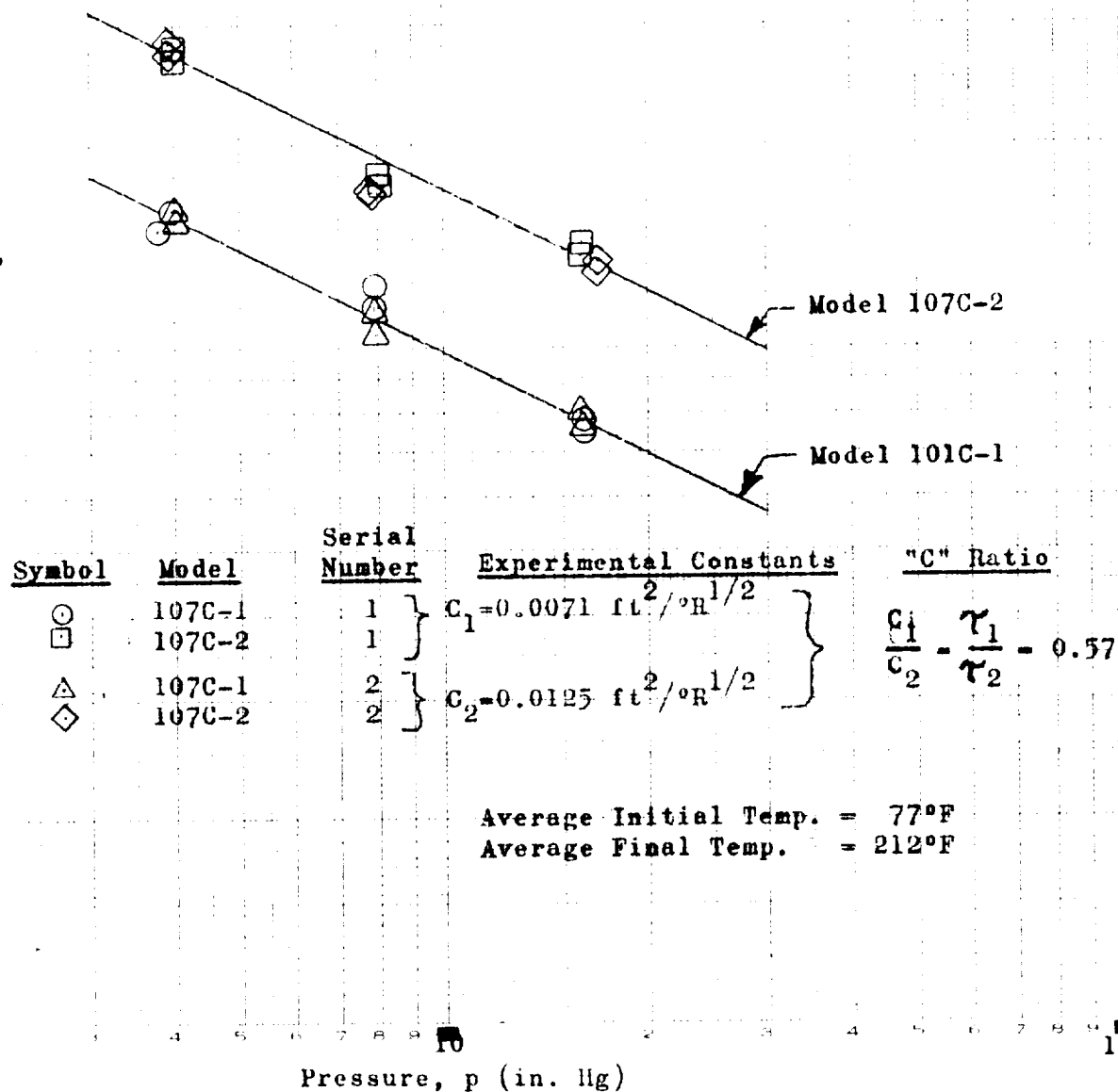
Figure 49: Calibration Data for Four Final Total Temperature Sensors
