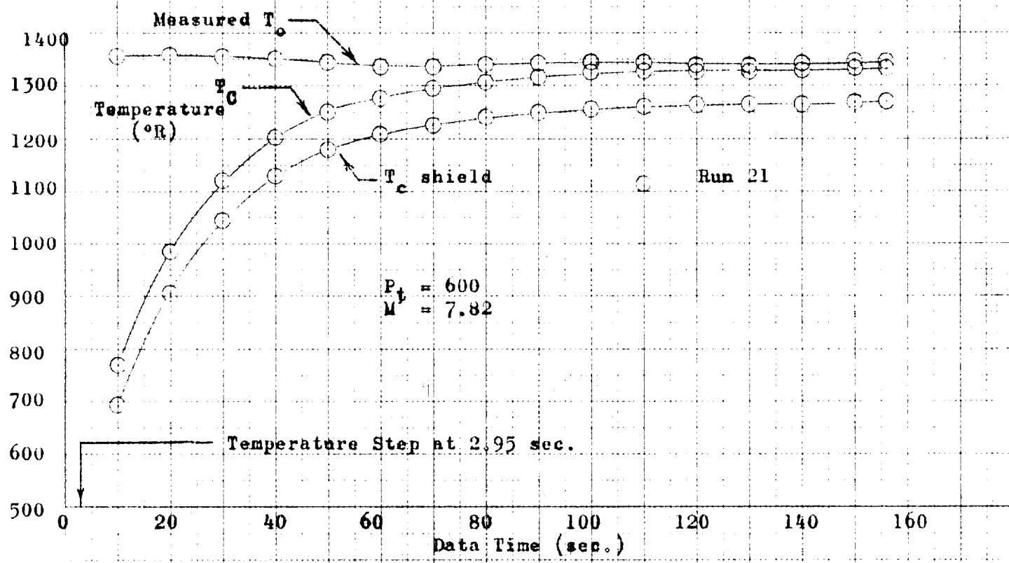
Figure 4b: Comparison of Shield Surface Temperatures with Element Temperatures and Measured T_0 for Sensor C, Mach 8 Wind Tunnel Runs.
