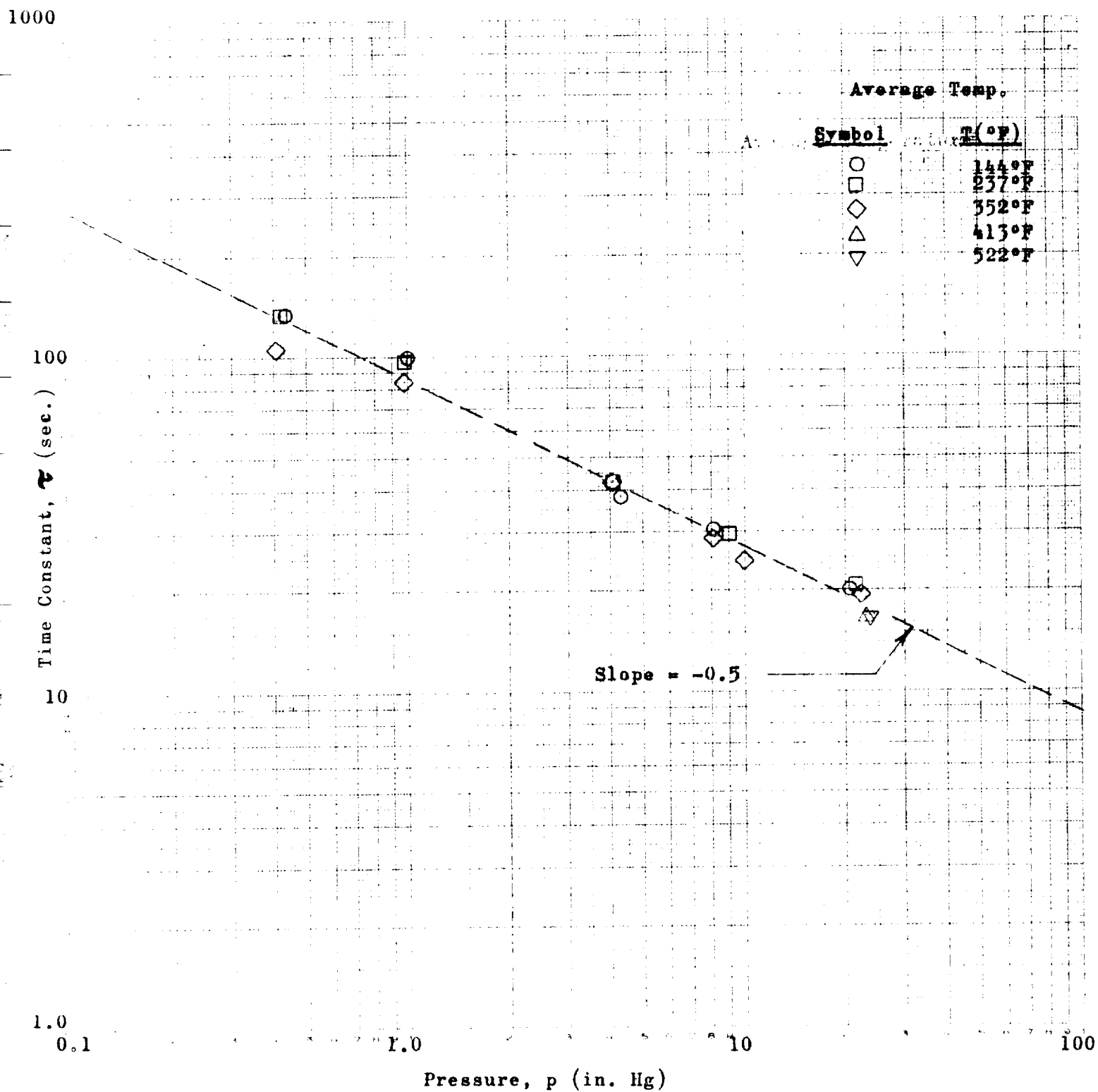
FIGURE 2Q Time Constant vs. Pressure for Type C Sensing Element
