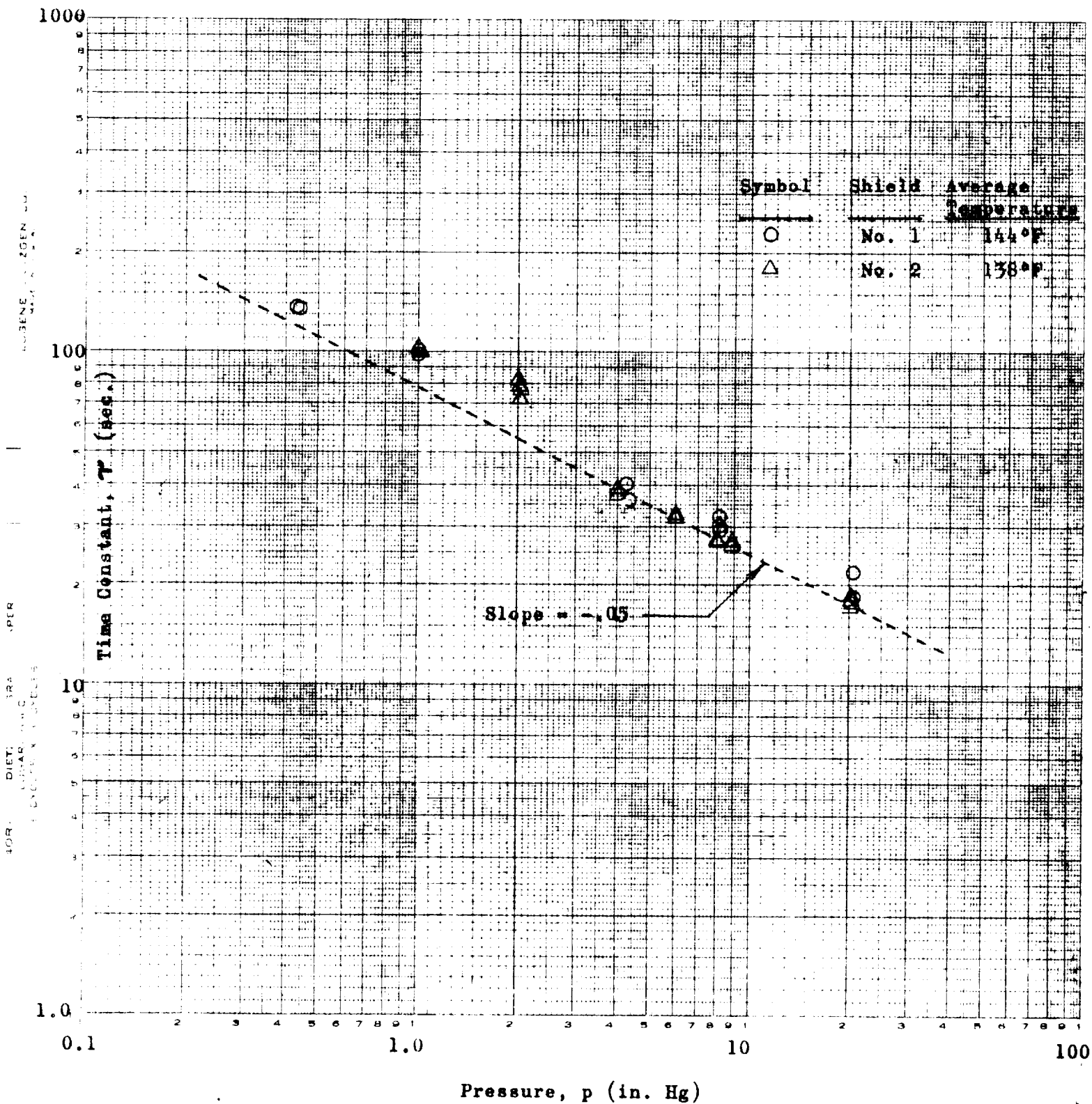
FIGURE 21: Time Constant vs. Pressure for Type C Sensing Element Installed in Two Radiation Shields
