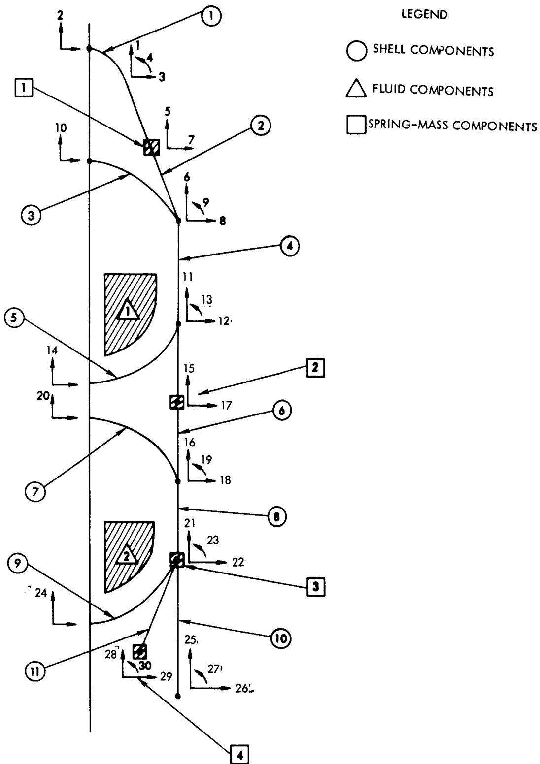
Figure F.2. System Components and Coordinates
