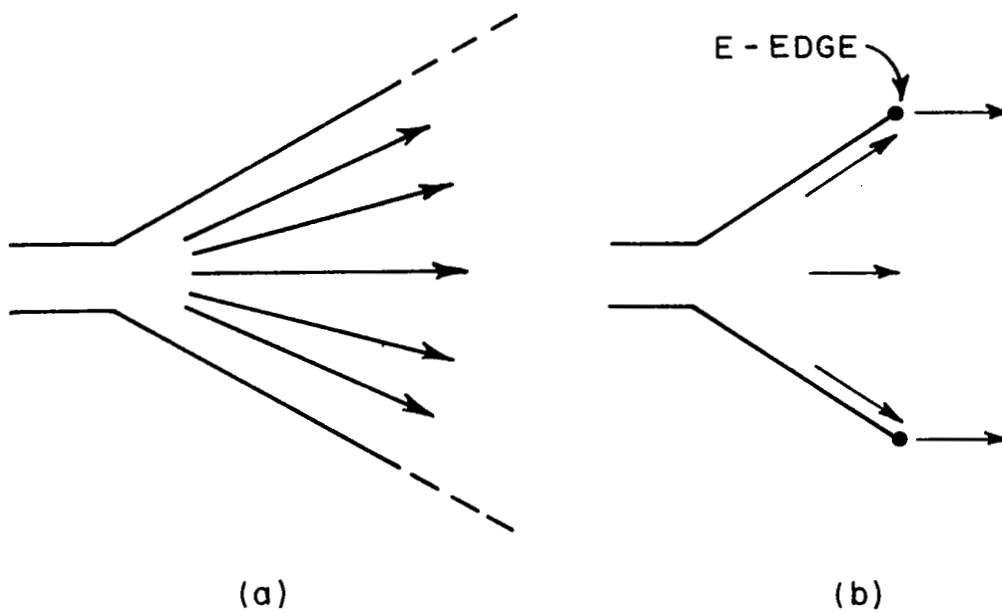
Fig. 17. E-plane cross section of horn.
