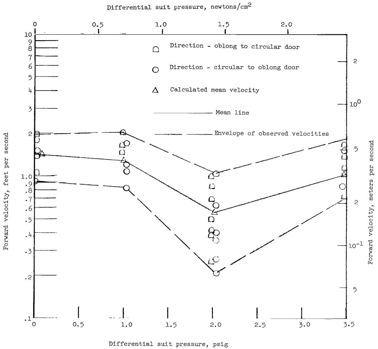
Figure 8.- Variation of observed forward velocity during ingress-egress maneuvers in water-immersion simulation with suit pressure.
