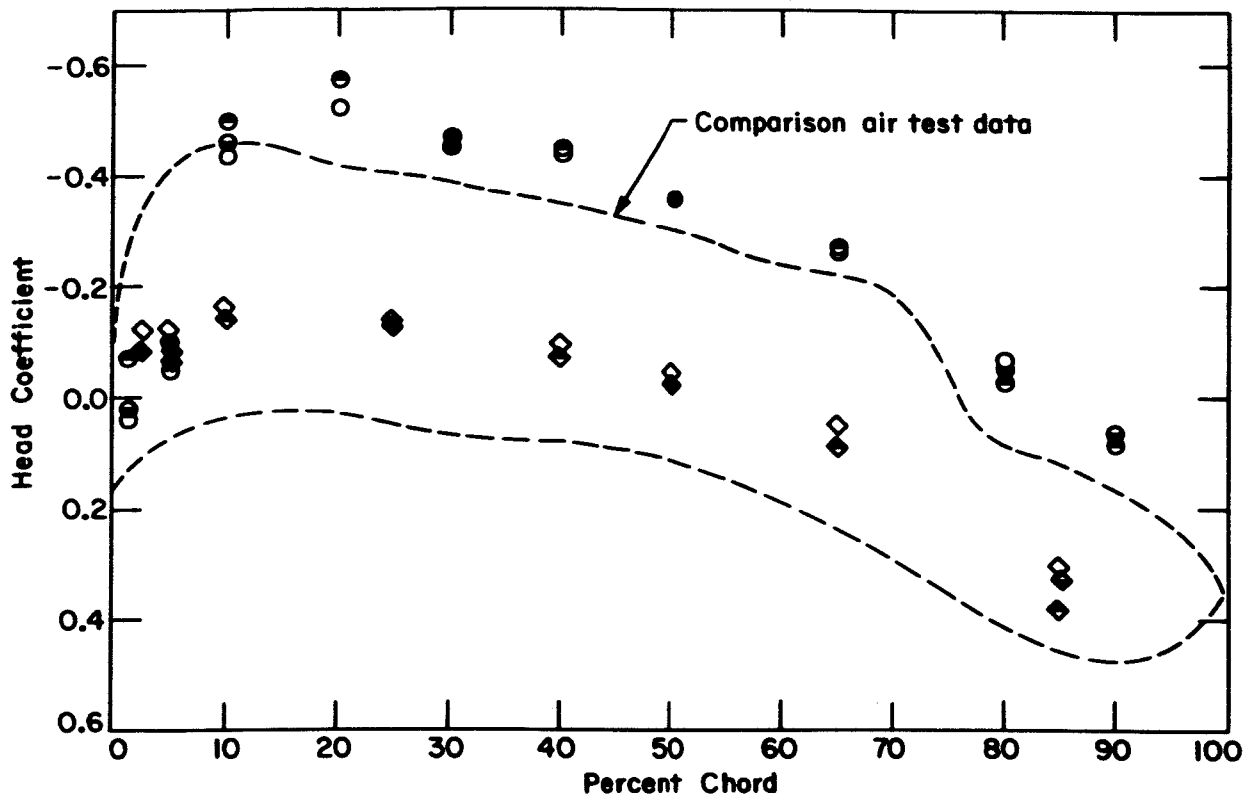
Figure 26. Experimental profile head coefficient distribution for \gamma = 33.2 degrees. \beta_1' = 45 degrees, \sigma = 1.5 . NACA 65(A 10 )-810 blade profile.
