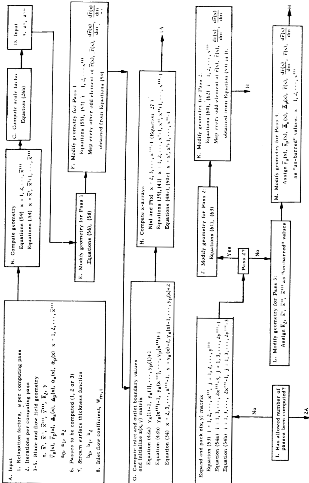
Computer program flow diagram. Main program.
