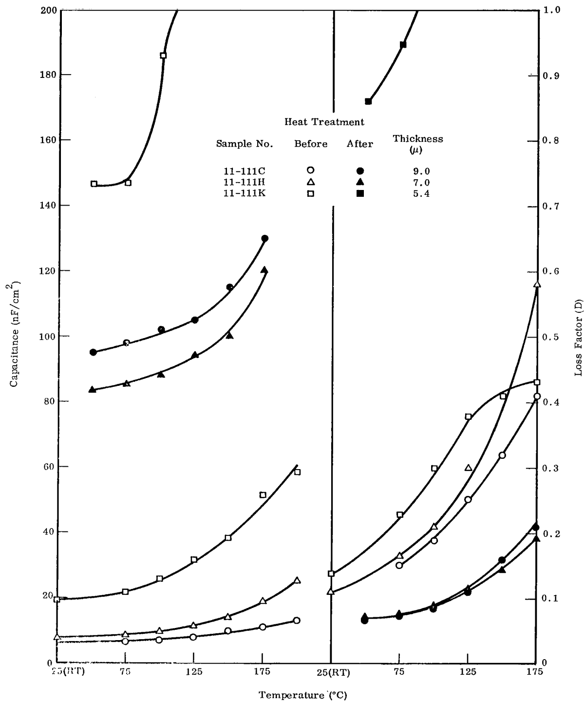
Fig. 3 Capacitance-Temperature Characteristics for Ti-Based Films
