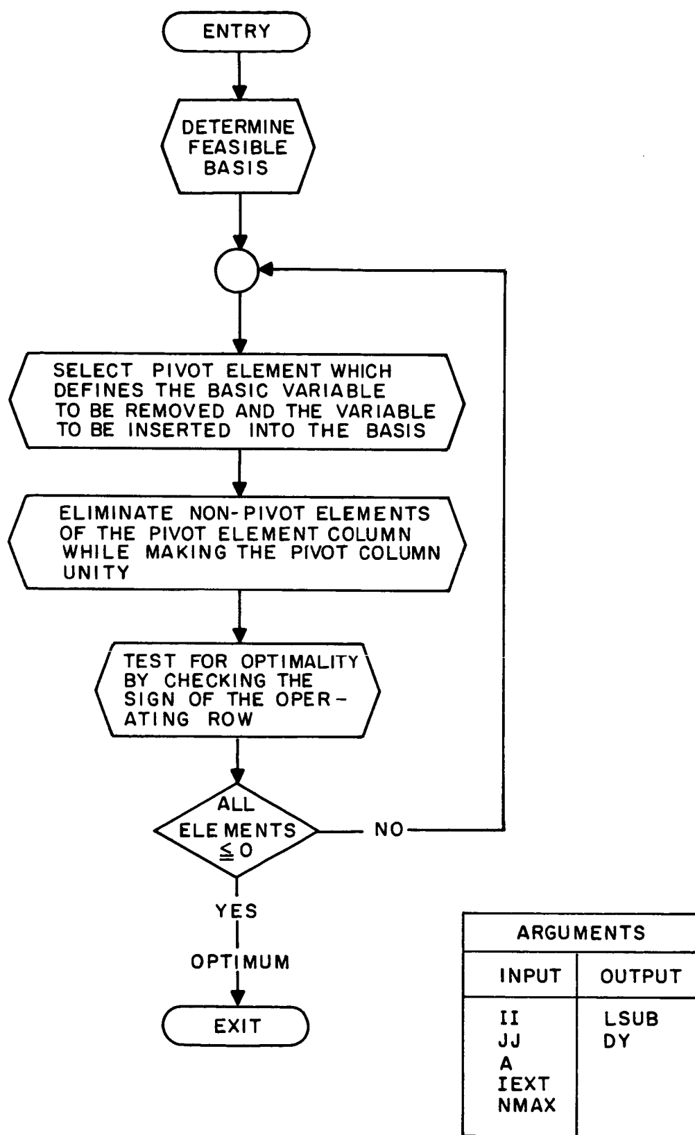
Linear Programming (LPSUB) Subroutine
