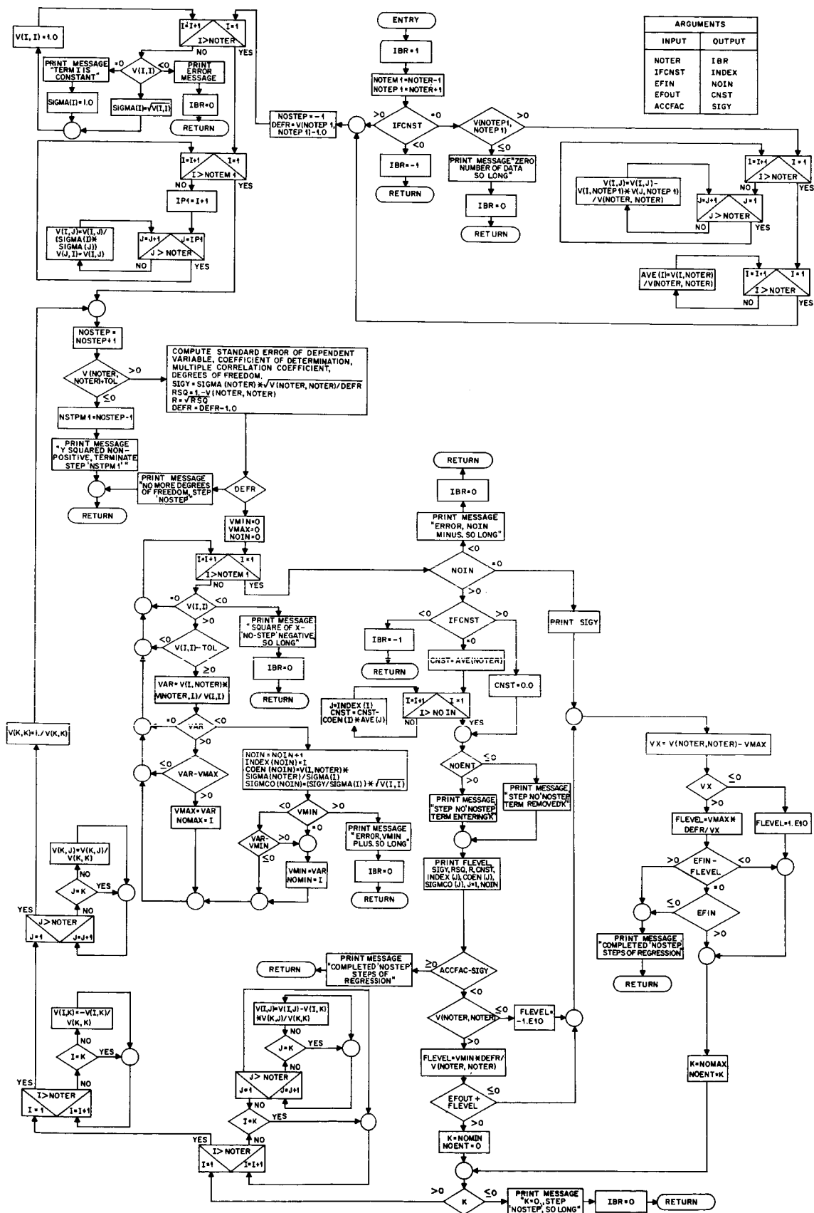
Figure E-28. SCORE-8 Subprogram -- Logic Flow Diagram
