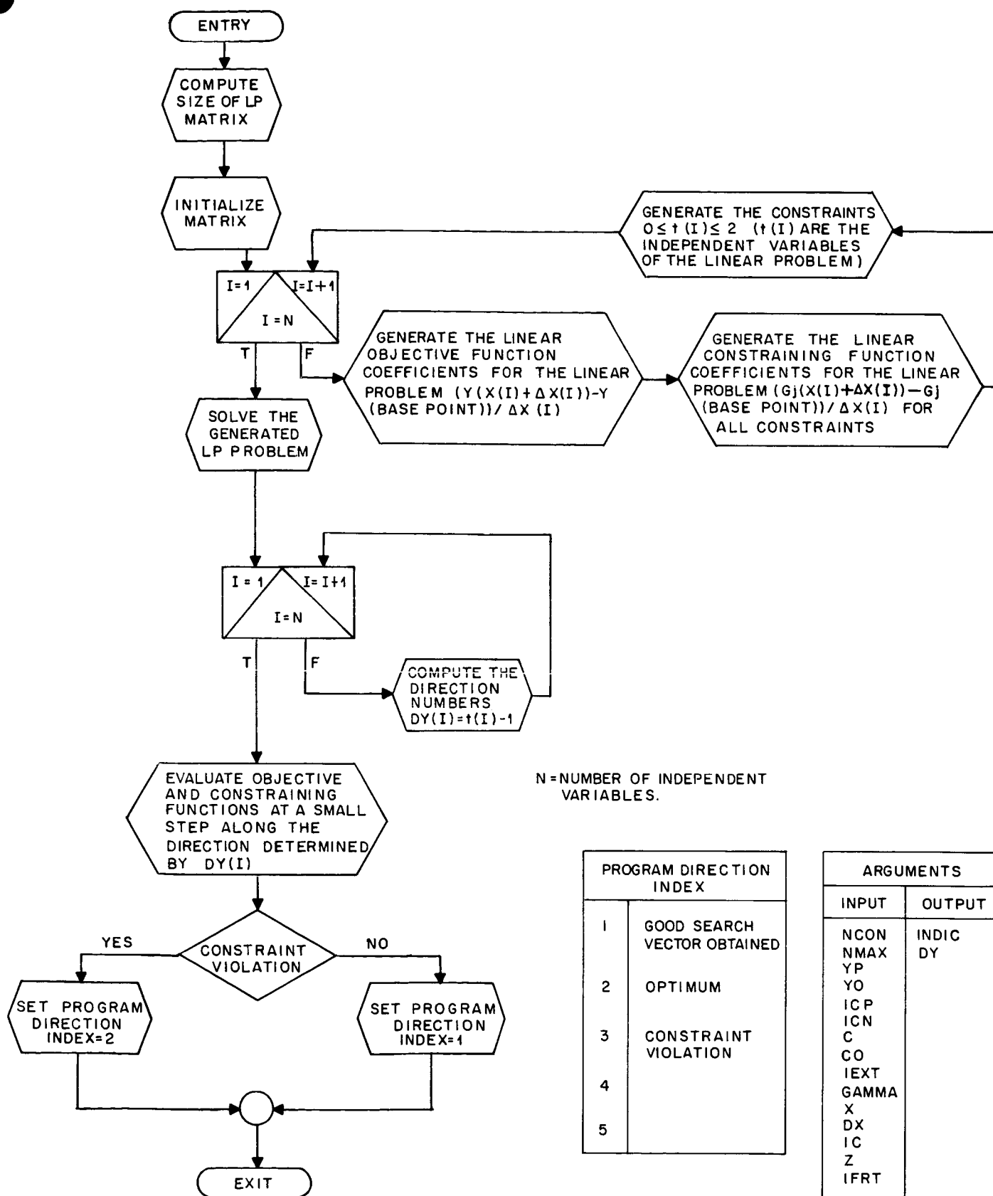
Type 3 Search (TANHYP) Subroutine
