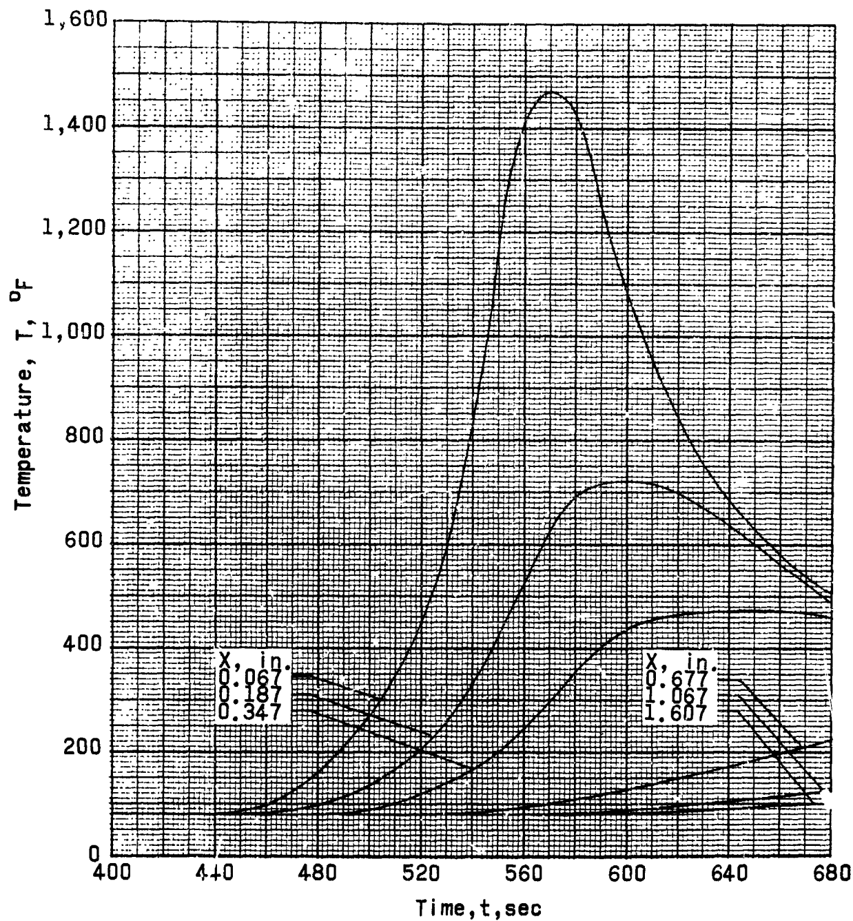
Figure 9.- Big Joe heat-shield faired temperature-time histories from a typical sensor, No. 1.
