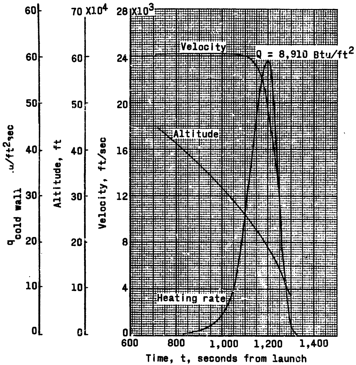
Figure 20.- Mercury nominal design entry trajectory (two retrorockets firing).
