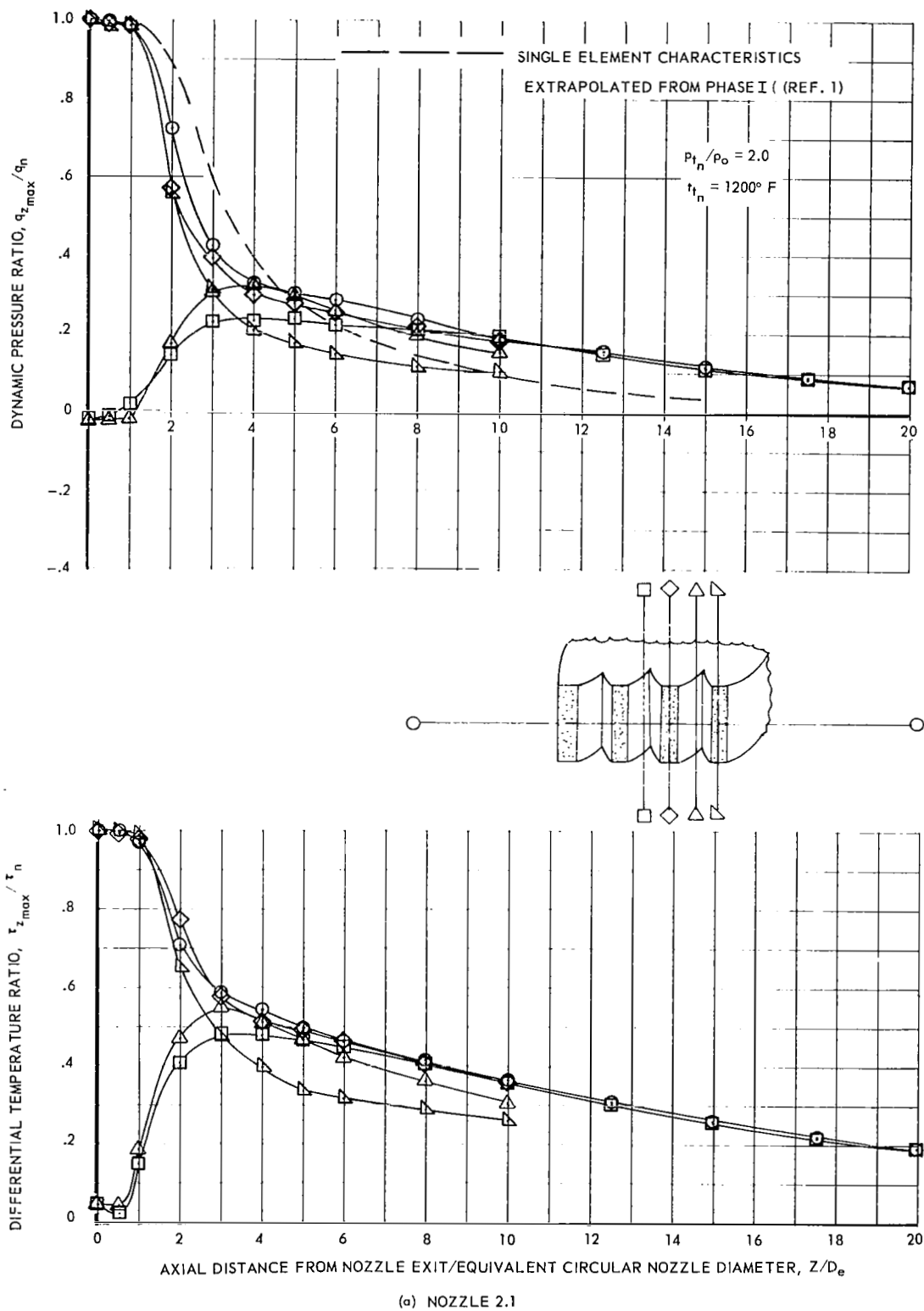
Figure 18 - Jet wake degradation characteristics for several basic nozzle configurations and survey planes
