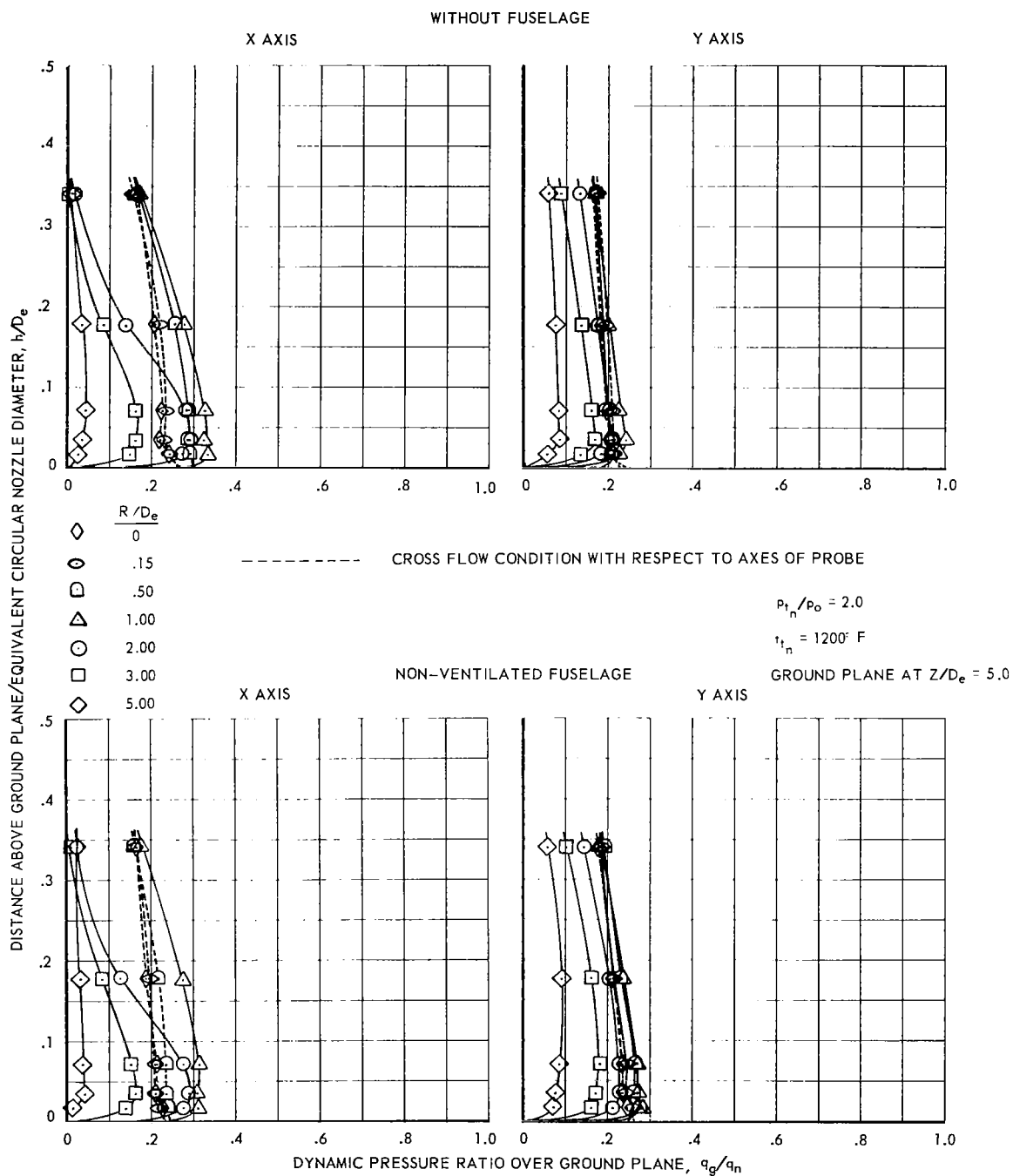
(b) SUPPRESSOR NOZZLE 2.1
