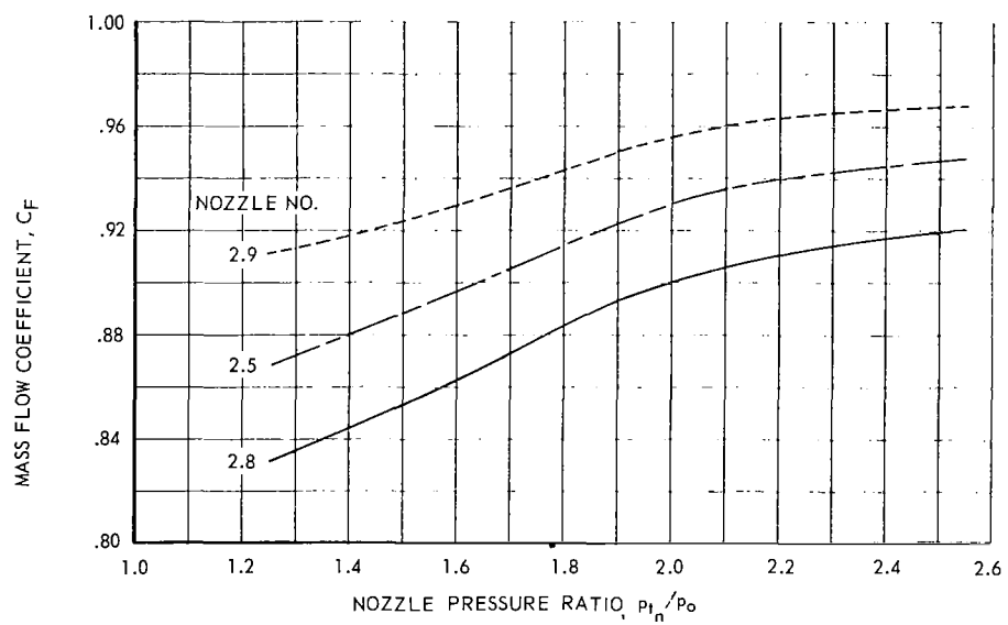
(c) PHASE II NOZZLES - VARIATION OF ASPECT RATIO, A
