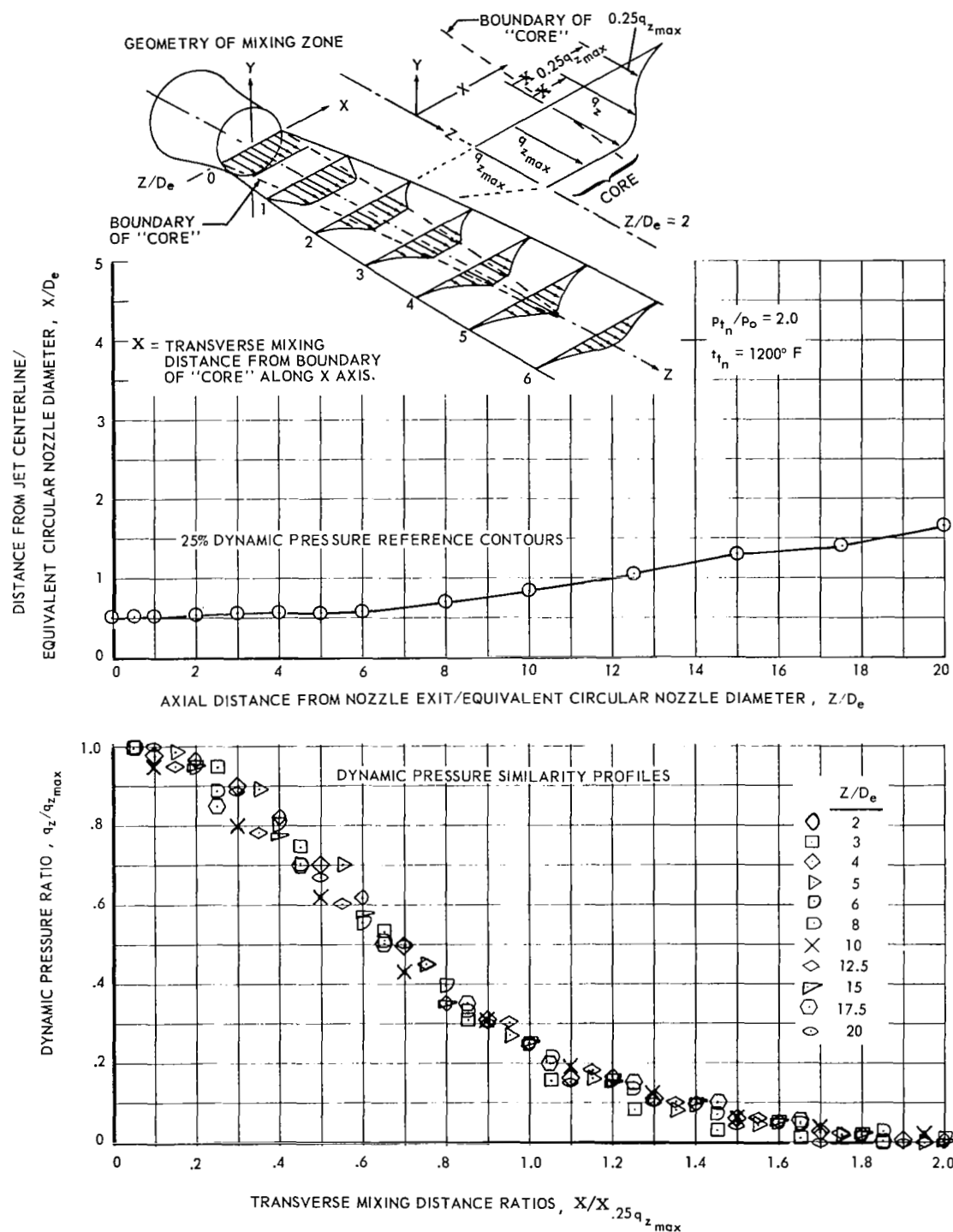
(a) CIRCULAR NOZZLE 1.1 - DYNAMIC PRESSURE RATIO
