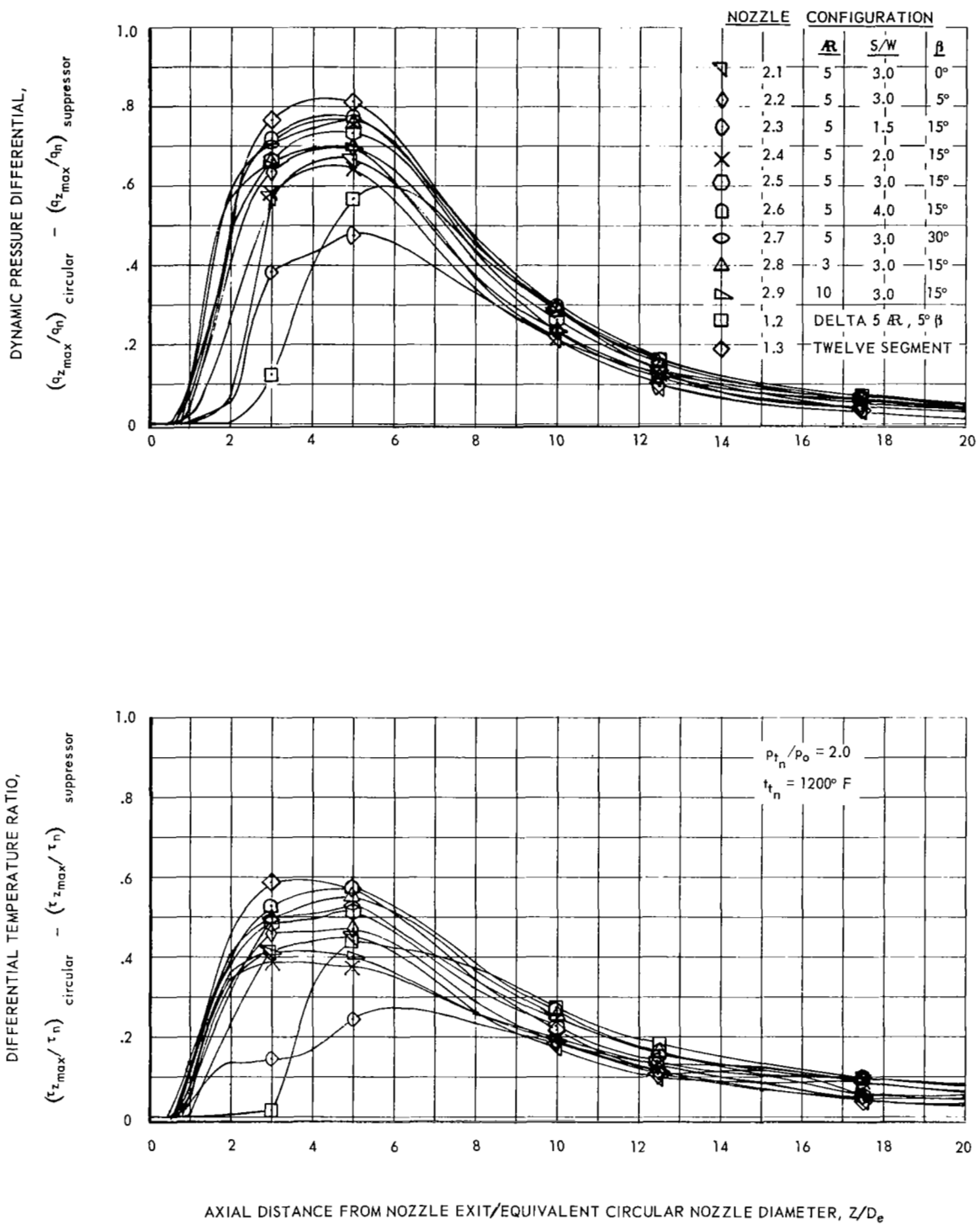
Figure 31 - Jet wake degradation characteristics of suppressor nozzles relative to the degradation characteristics of a circular nozzle for all basic nozzles out of ground effect
