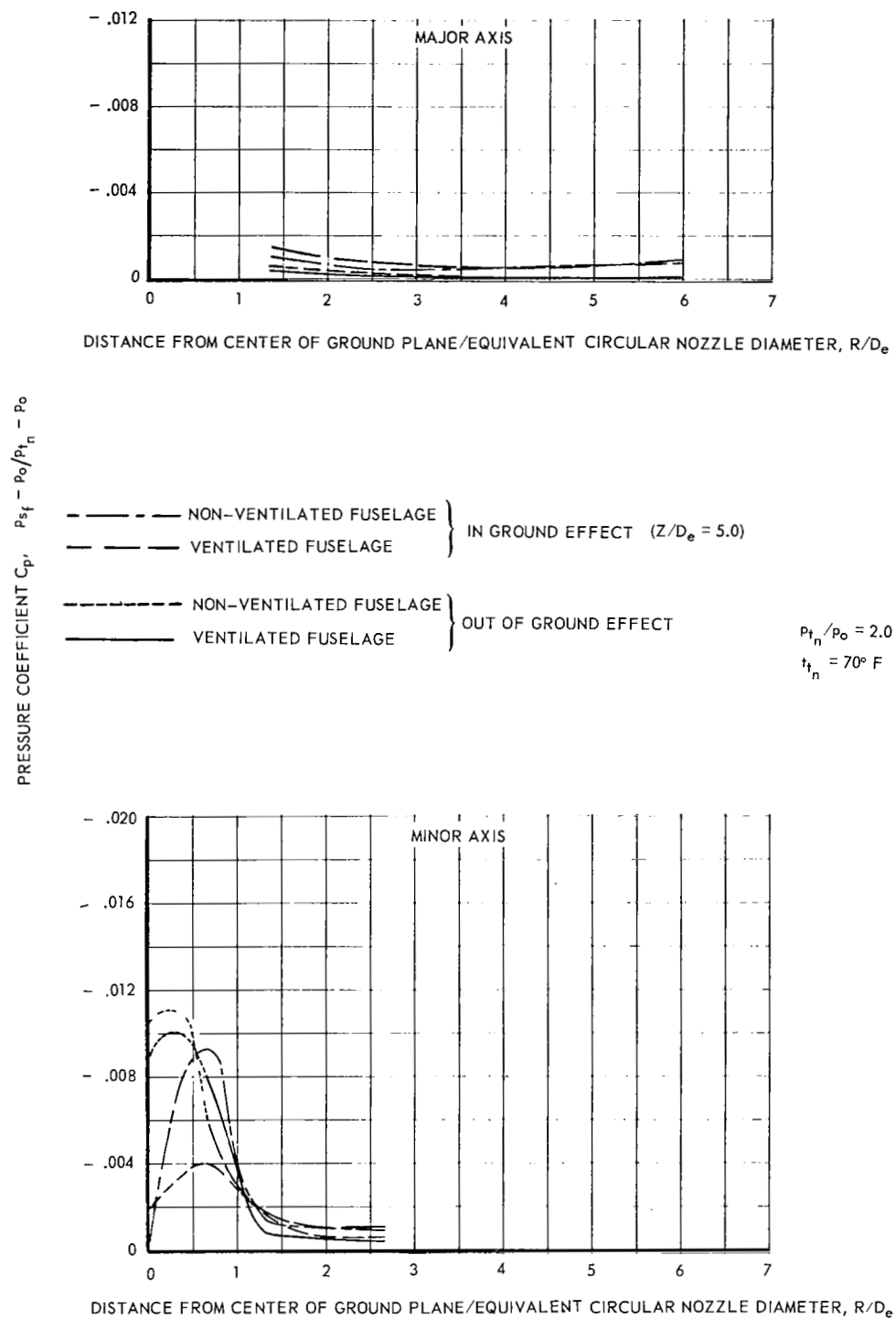
(b) SUPPRESSOR NOZZLE 2.1
