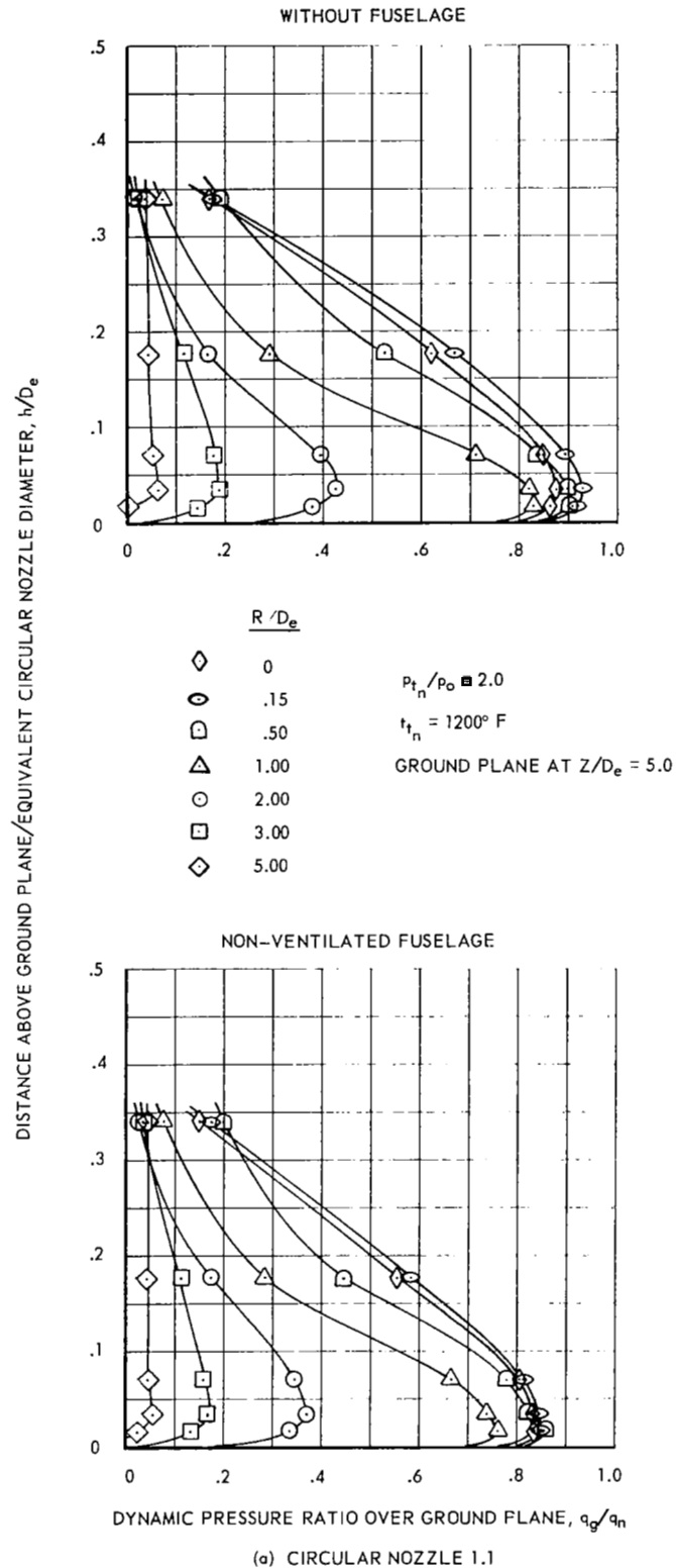
Figure 20 - Dynamic pressure distribution in the jet efflux adjacent to the ground plane
