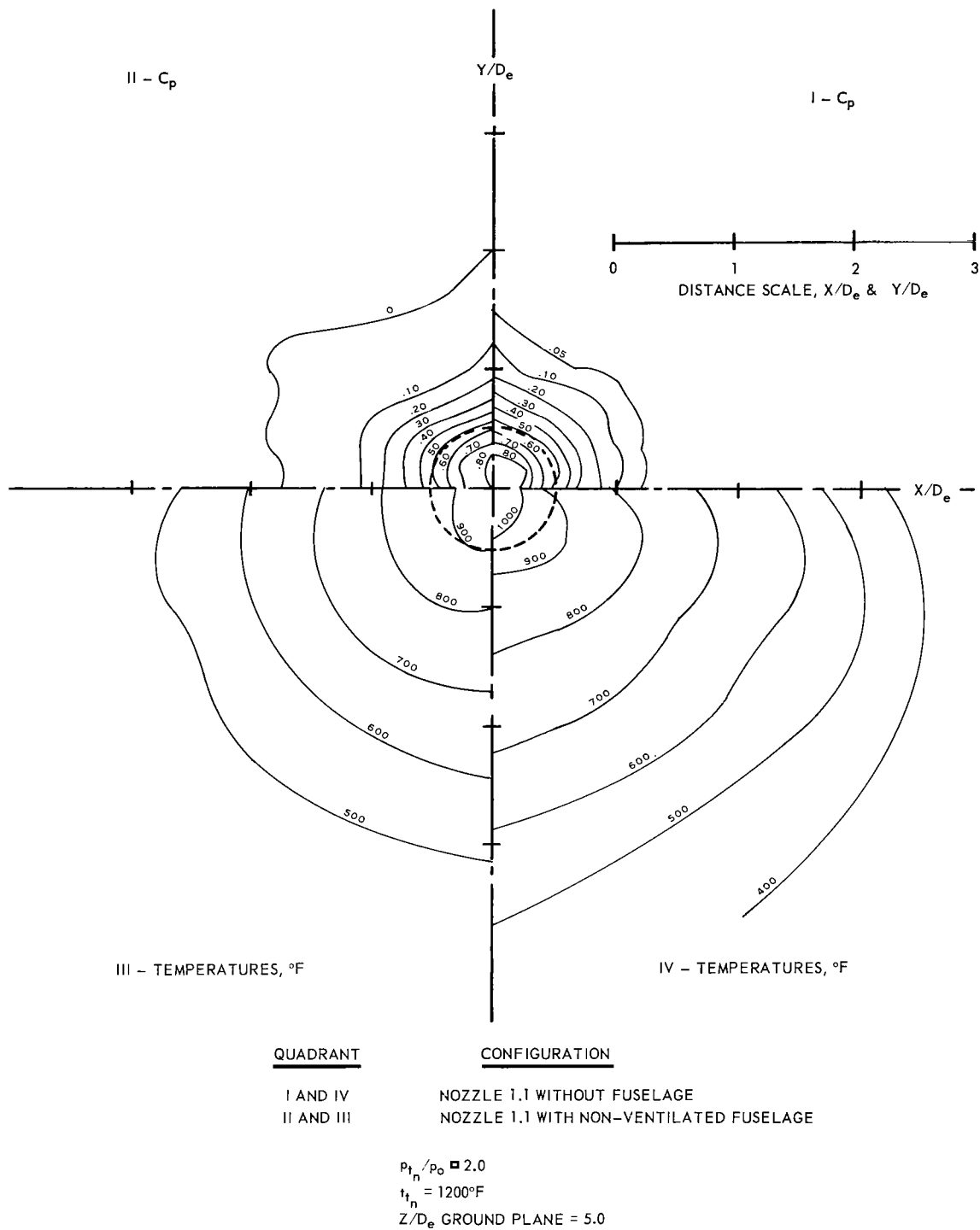
(a) CIRCULAR NOZZLE 1.1
