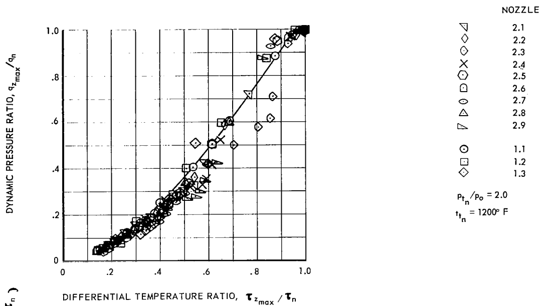
(a) DYNAMIC PRESSURE RATIO VERSUS DIFFERENTIAL TEMPERATURE RATIO
