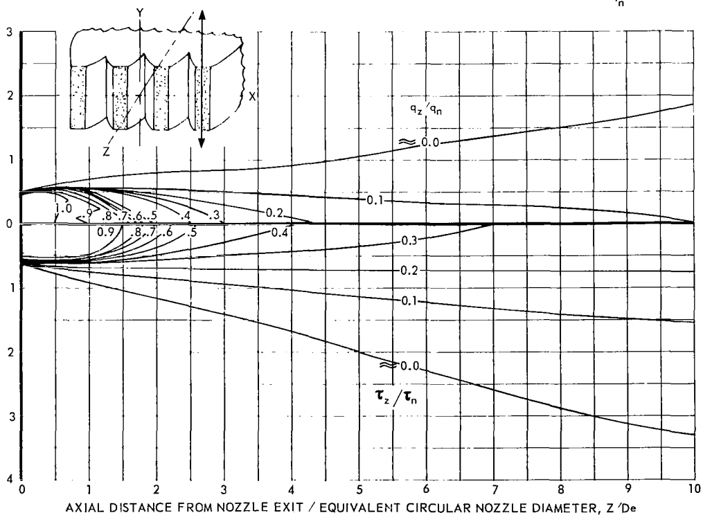
(e) SUPPRESSOR NOZZLE 2.1 ( X = 2.70 INCHES).
