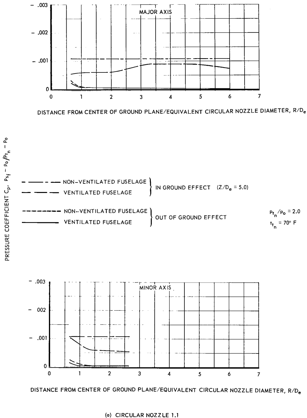
Figure 26 - Radial distribution of pressures induced on the lower surface of the fuselage by the jet
