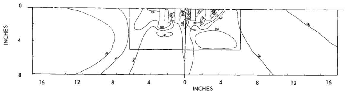
III - NOZZLE 2.5 IN GROUND EFFECT
