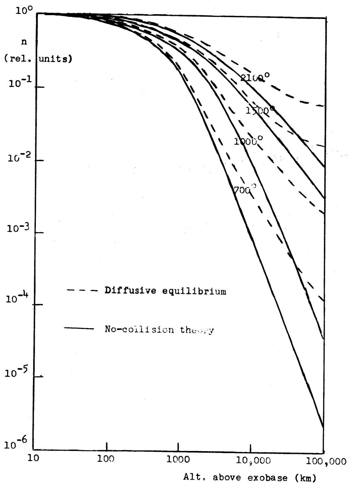
Figure 12. Diffusive equilibrium versus no-collision theory for hydrogen densities.
