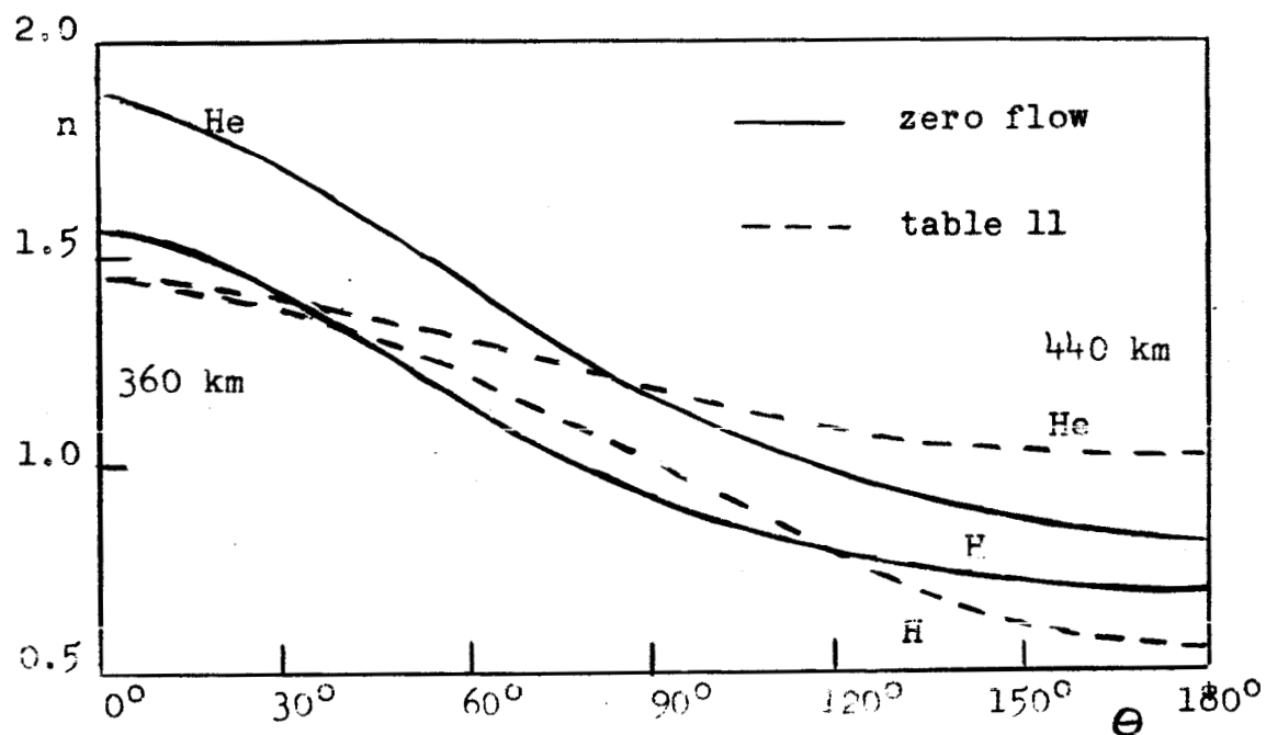
Figure 41. Hydrogen and helium densities in 10^4 and 10^6 \text{ cm}^{-3} respectively for zero flow and as in table 11, for a 700\text{-}1000^\circ sinusoidal temperature variation.
