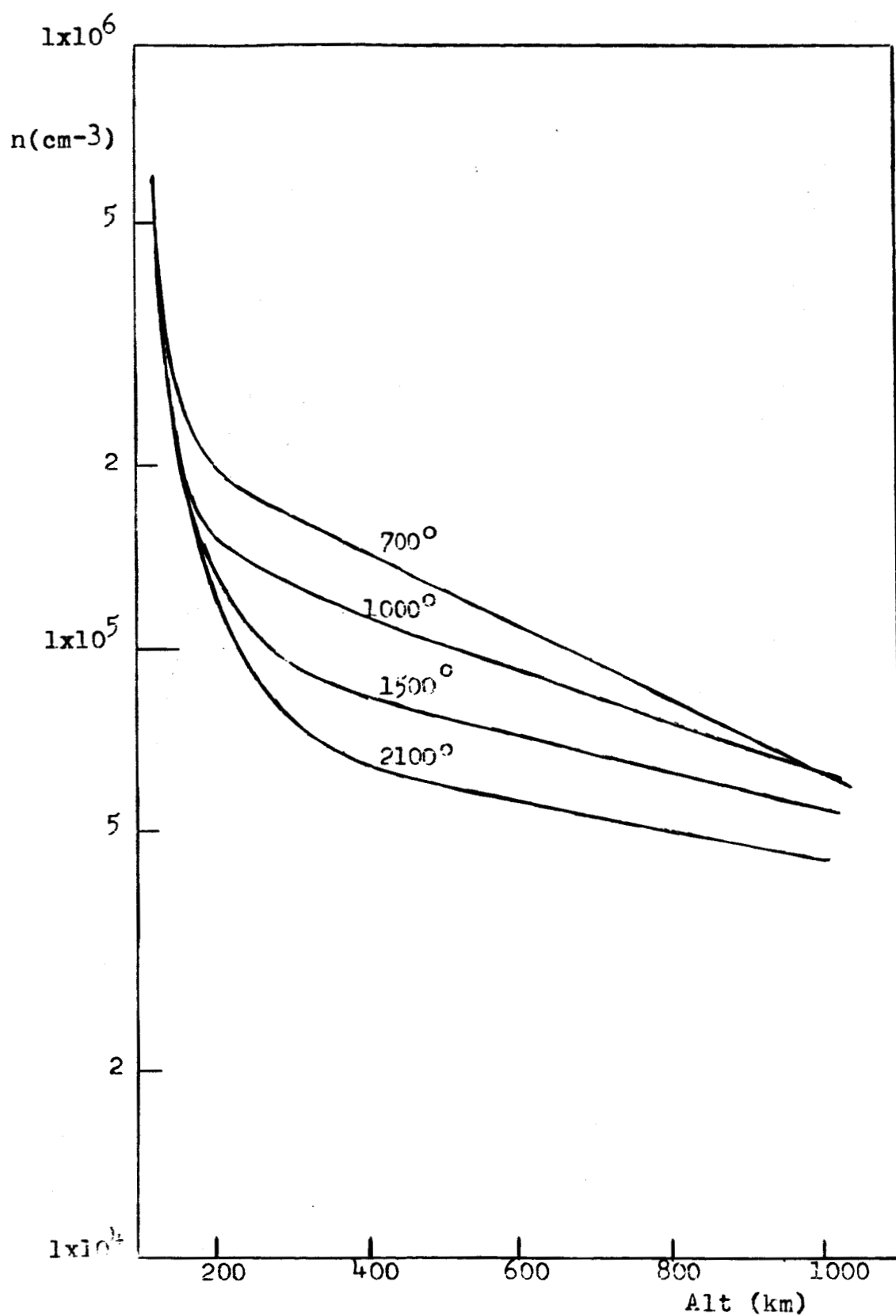
Figure 3. Hydrogen densities for diffusive equilibrium and temperature Model A.
