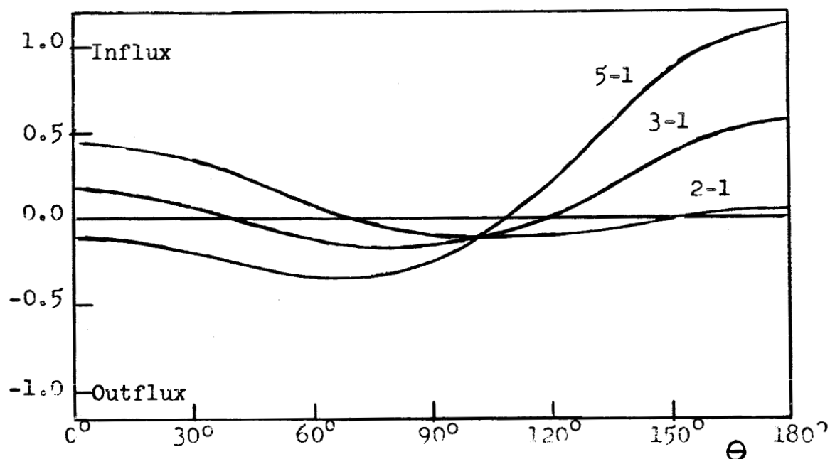
Figure 29. Hydrogen flux in 10^4 \text{ cm}^{-2} \text{ sec}^{-1} for 700-1000^\circ sinusoidal temperature variation and various sinusoidal density variations about unity. Density maximum at \theta = 0 , temperature maximum at \theta = 180^\circ .
