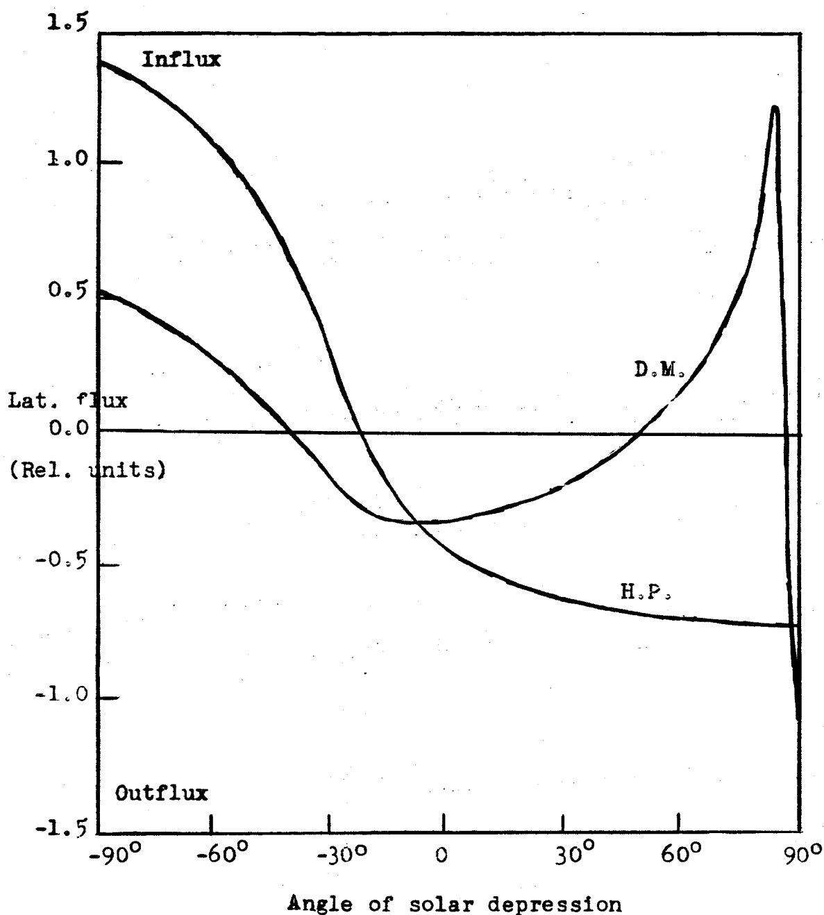
Figure 14. Lateral flux for a sinusoidal 1500-1000°, 2-1, case using the Hanson-Patterson approximations (H.P.) and the Donahue-McAfee approximation (D.M.).
