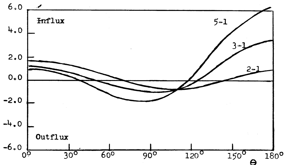
Figure 34. Oxygen flux in 10\text{cm}^{-2}\text{sec}^{-1} for 1500-2100° sinusoidal temperature variation and various sinusoidal density variations about unity. Density maximum at \Theta = 0 , temperature maximum at \Theta = 180^\circ .
