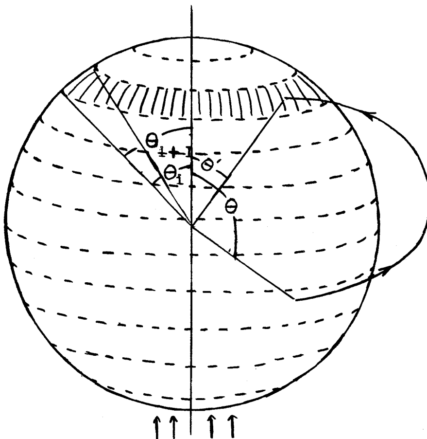
Figure 16. Geometry for spherical model with particle originating at \Theta and ending at \Theta' between \Theta_i and \Theta_{i+1} .
