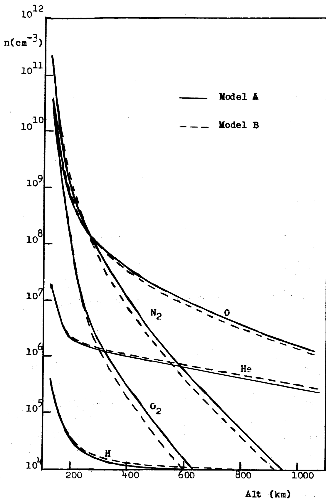
Figure 10. Comparison of diffusive equilibrium densities for temperature Models A and B.
