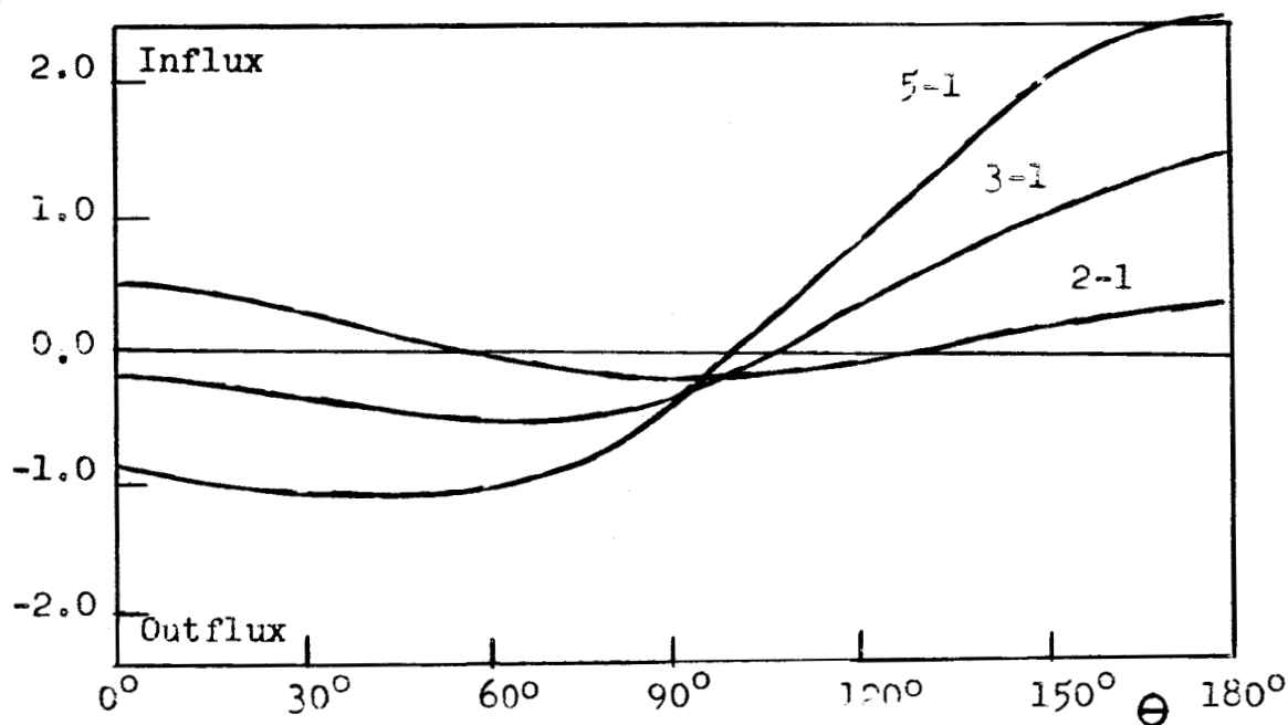
Figure 30. Hydrogen flux in 10^4 \text{ cm}^{-2} \text{ sec}^{-1} for 1000-1500^\circ sinusoidal temperature variation and various sinusoidal density variations about unity. Density maximum at \theta = 0 , temperature maximum at \theta = 180^\circ .
