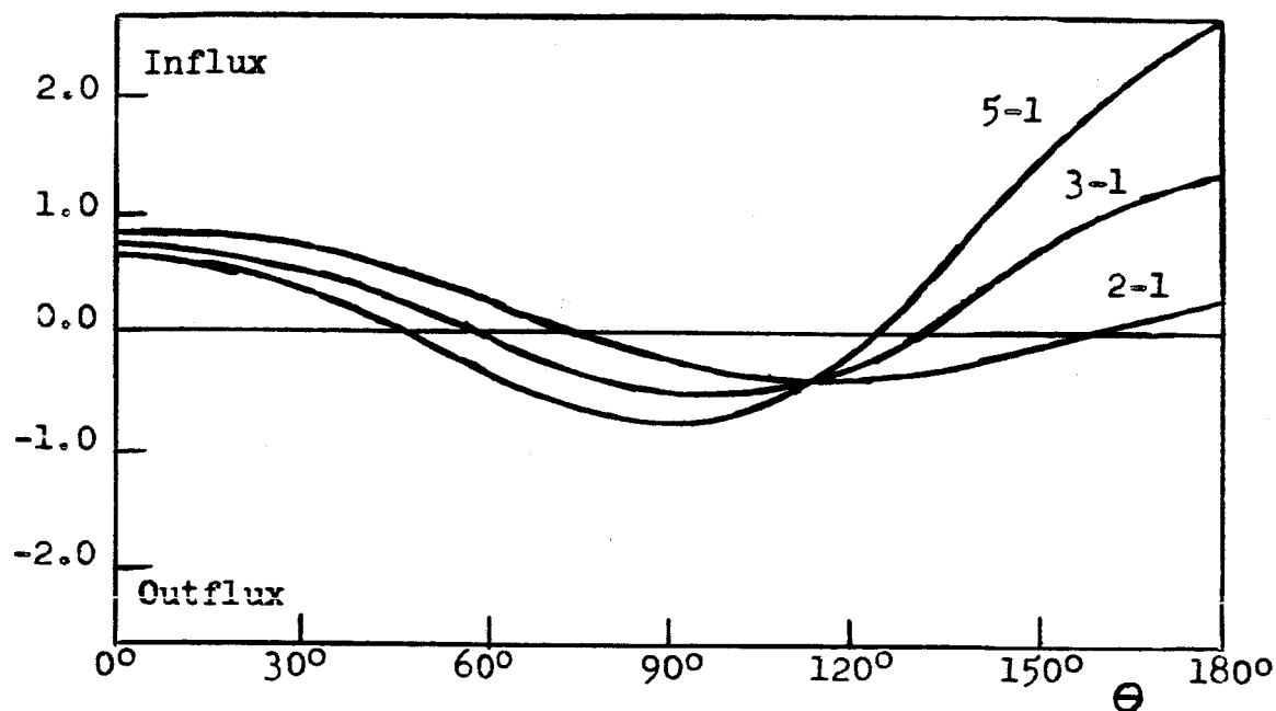
Figure 33. Oxygen flux in 10\text{cm}^{-2}\text{sec}^{-1} for 1000-1500° sinusoidal temperature variation and various sinusoidal density variations about unity. Density maximum at \Theta = 0 , temperature maximum at \Theta = 180^\circ .
