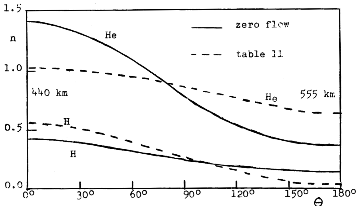
Figure 42. Hydrogen and helium densities in 10^5 and 10^6 \text{ cm}^{-3} respectively for zero flow and as in table 11, for a 1000\text{-}1500^\circ sinusoidal temperature variation.
