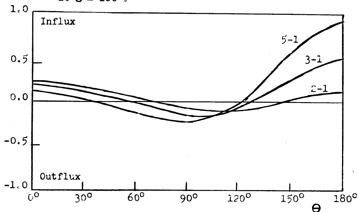
Figure 32. Oxygen flux in 10 \text{ cm}^{-2} \text{ sec}^{-1} for 700\text{--}1000^\circ sinusoidal temperature variation and various sinusoidal density variations about unity. Density maximum at \theta = 0 , temperature maximum at \theta = 180^\circ .
