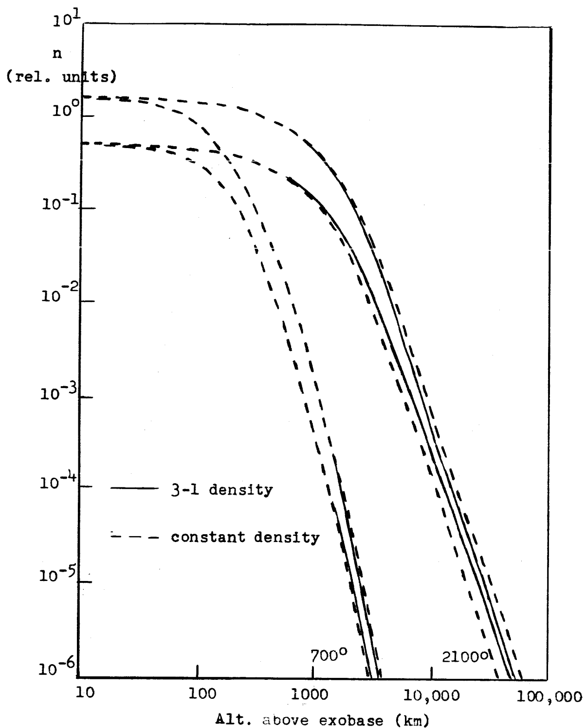
Figure 46. Exospheric helium densities for constant and sinusoidal 3-l density exobases and 700^\circ and 2100^\circ exospheric temperatures.
