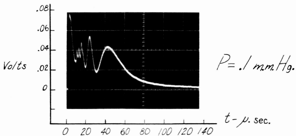
Fig. 12. Detector output for varying neutral gas pressures.
