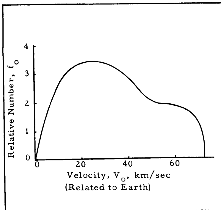
Figure 6 Meteoroid Velocity Distribution Relative to the Earth
