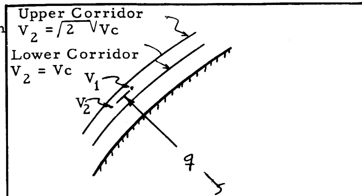
Figure 3. Corridor Boundaries (at perigee)
