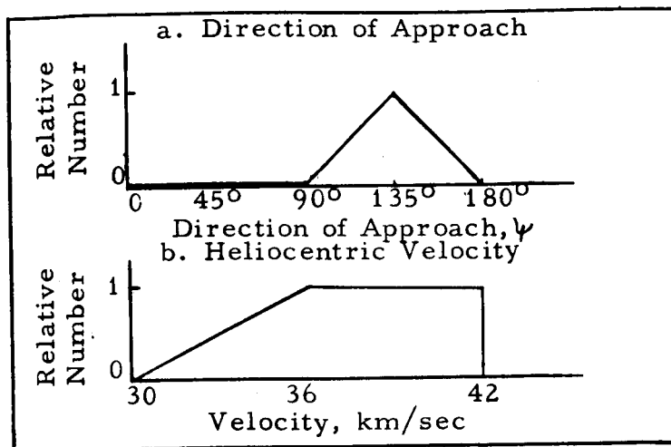
Figure 5 Velocity & Direction of Approach of Meteors
