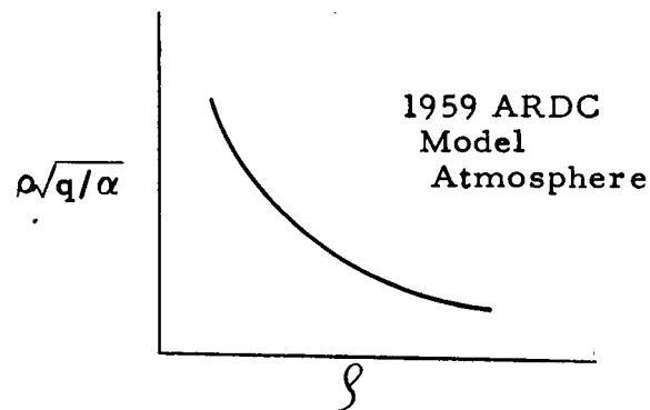
Figure 4. Corridor Functions vs Altitude
