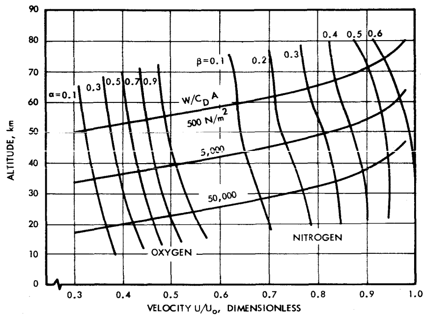
FIG. 9. DEGREE OF OXYGEN AND NITROGEN DISSOCIATION FOR SIMPLIFIED AIR-MODEL AT STAGNATION POINT. ALSO RE-ENTRY TRAJECTORIES FOR VARIOUS BALLISTIC VEHICLES. CIRCULAR VELOCITY U_0 = 7,910 m/s.
