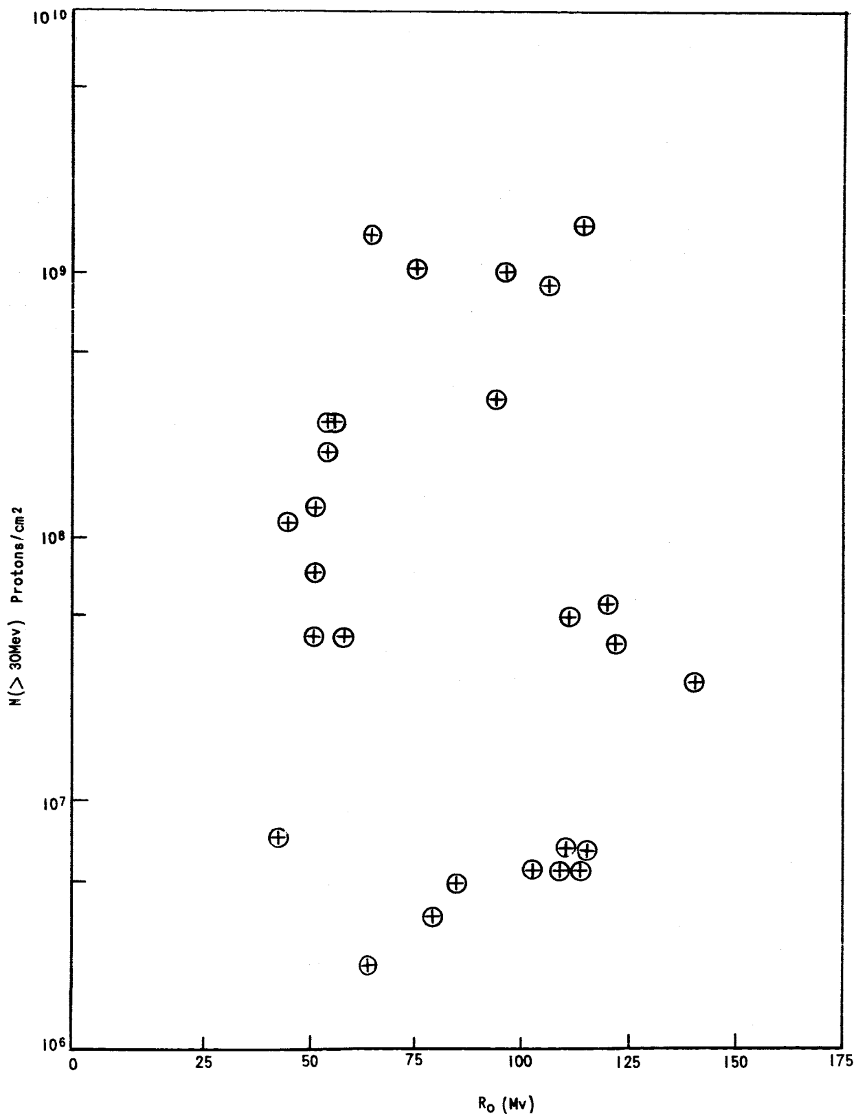
FIGURE 5 CORRELATIONS BETWEEN EVENT SIZE AND R_0
