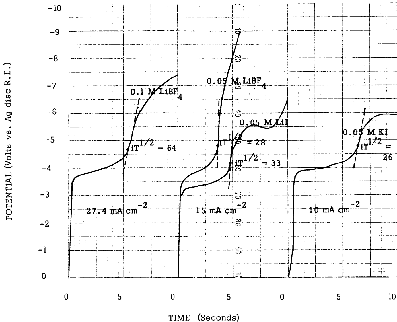
Figure 24: CATHODIC CHRONOPOTENTIOMETRY IN ACETONITRILE
