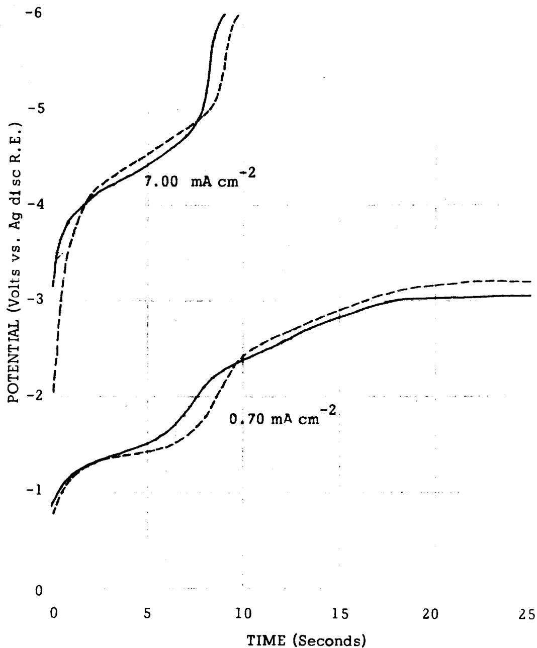
Figure 17: Cathodic Chronopotentiometry in Propylene Carbonate -- 0.1 M \text{LiBF}_4 Chronopotentiograms obtained on polished platinum electrodes at current indicated. Solid lines are for the freshly prepared solution. Dashed lines are for the solution which had stood overnight.
