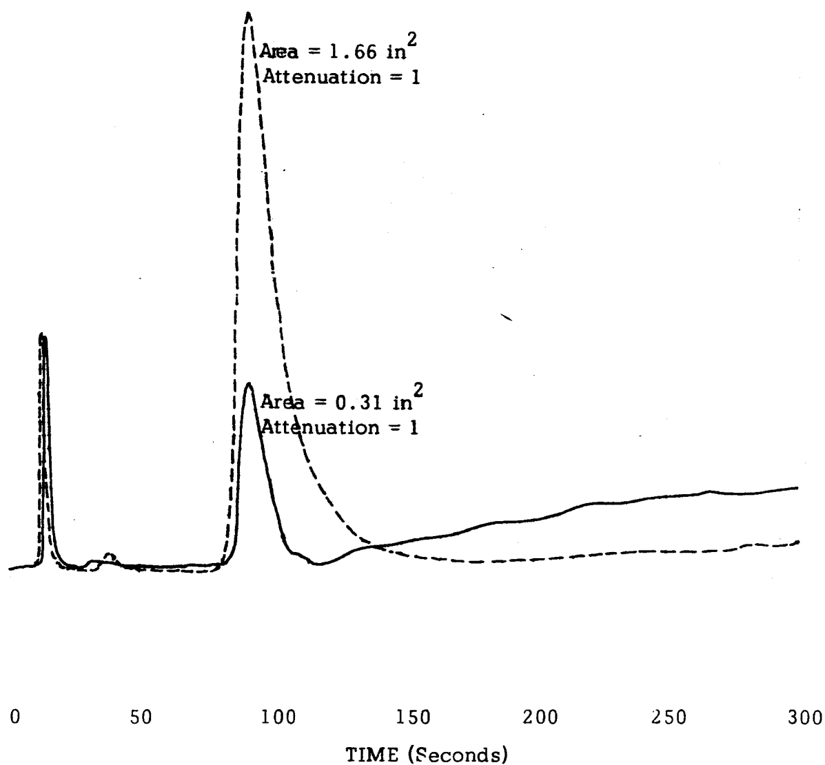
Figure 16: Vapor Phase Chromatograms of Propylene Carbonate Performed with 4 microliter samples, with temperature programming (see text).
