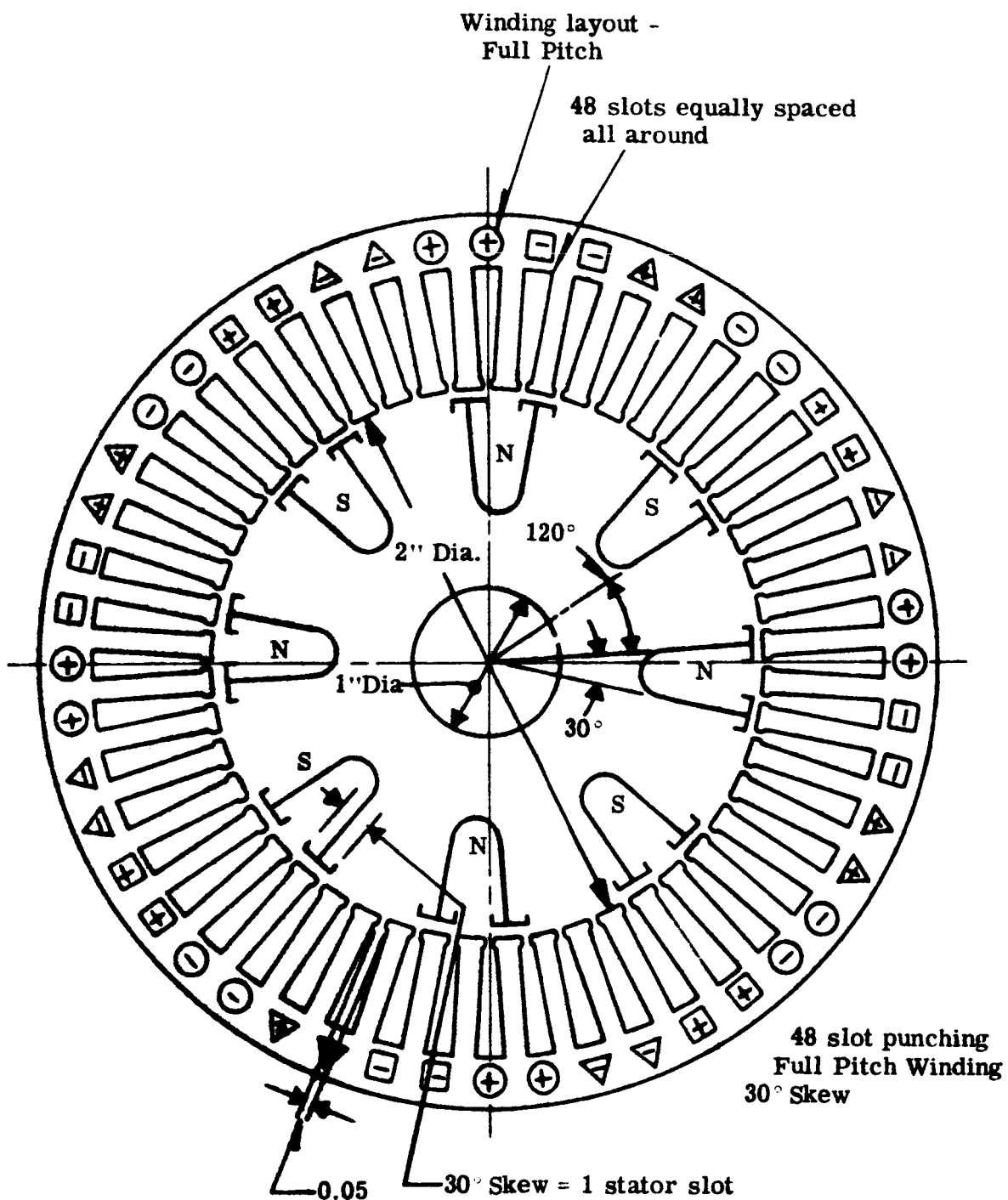
FIGURE 4. Layout for Ripple Determination
