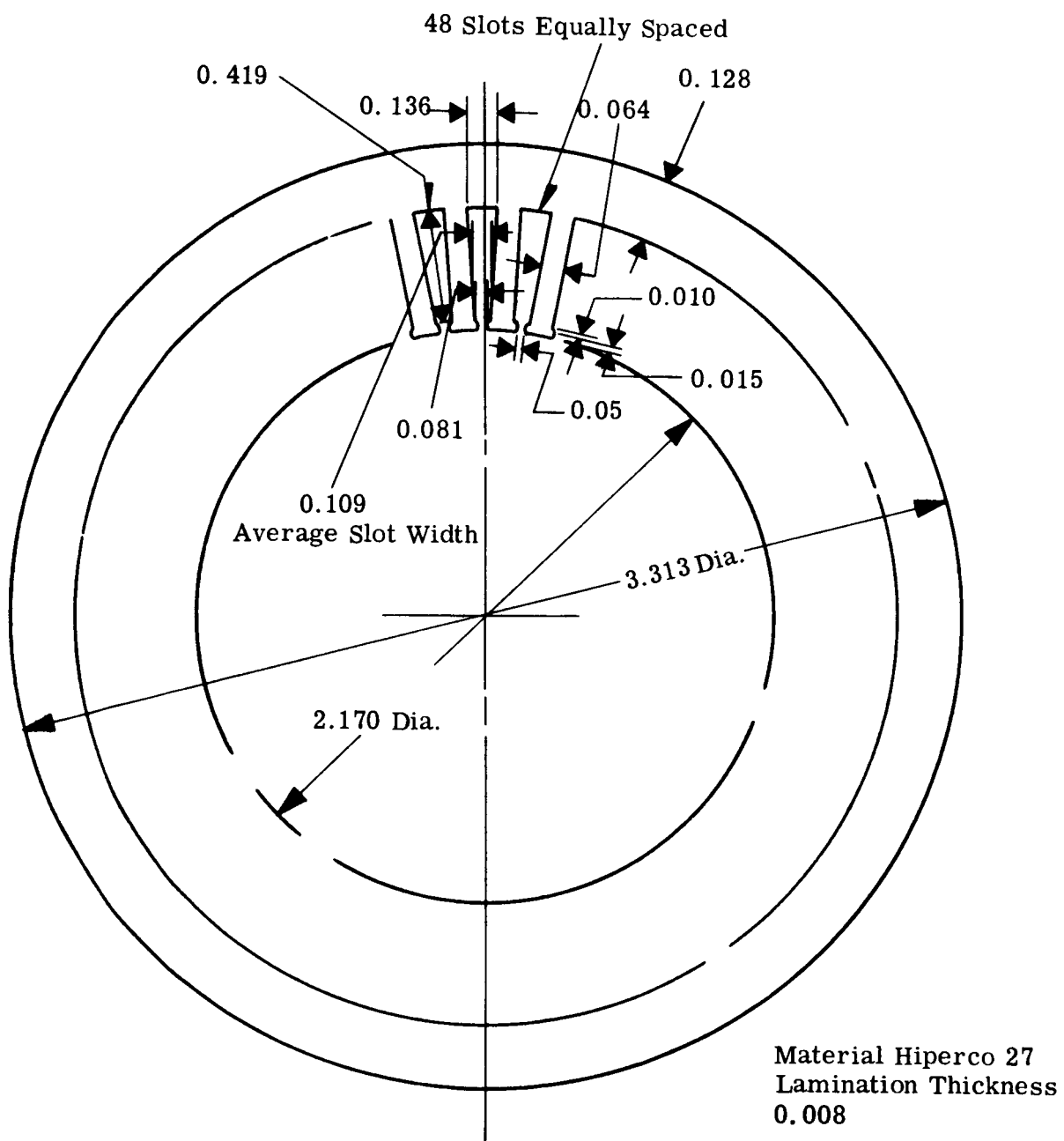
FIGURE 10. Armature Punching
