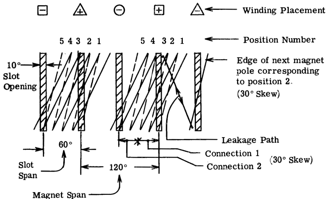
FIGURE 3. Layout for Illustration of Skew Effect
