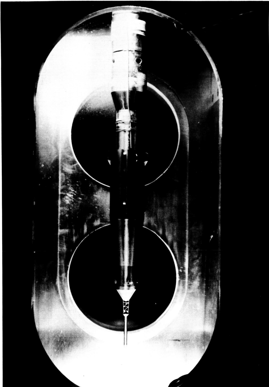
Figure 2. SATURN IB Upper Stage Test Configuration A_4^{8037} S_1C_1T_1t_3 Sting - Mounted in the AEDC von Karman Facility Hypersonic Tunnel E.
