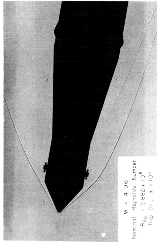
Figure 10. High Altitude Configuration (concluded)
