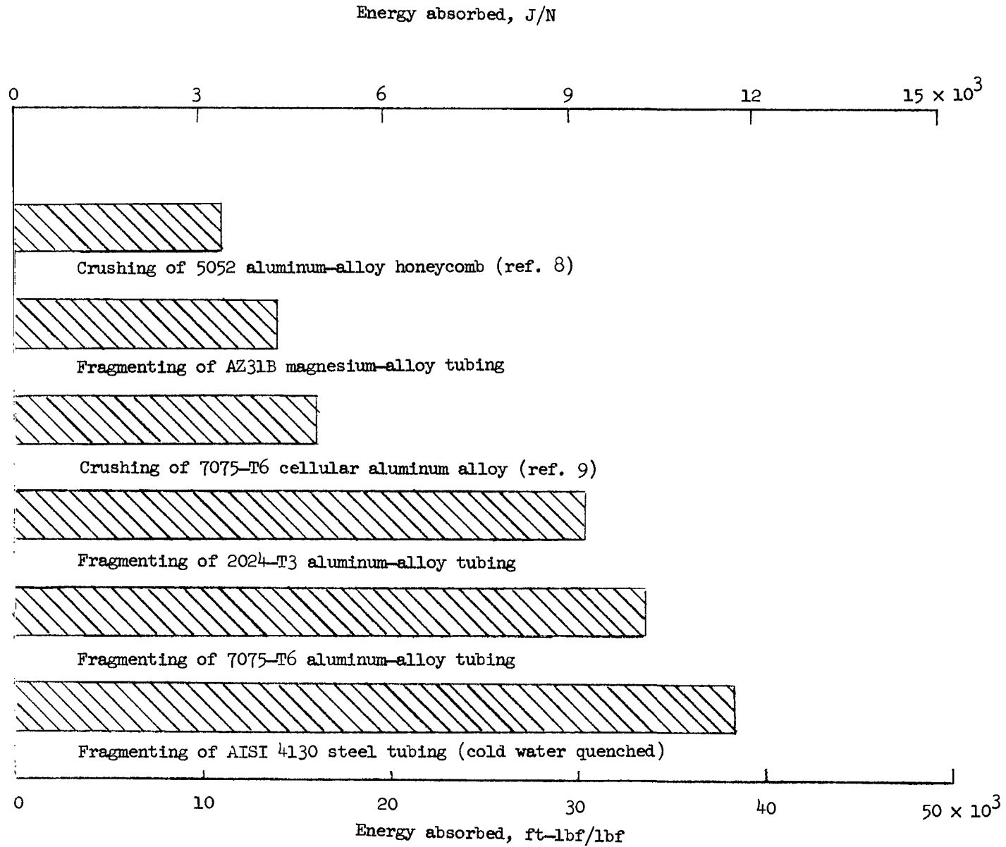
Figure 13.- Energy-absorption capabilities of various materials and processes.
