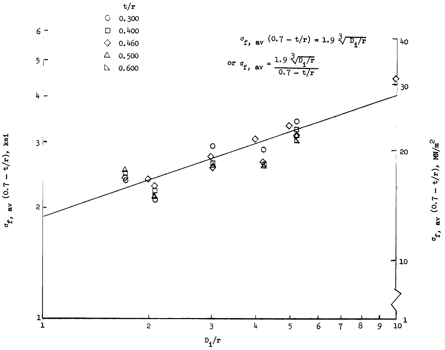
Figure 9.- Variation of product of average fragmenting stress and function of tube-wall-thickness—die-radius ratio with tube-inside-diameter—die-radius ratio for 2024-T3 aluminum alloy.
