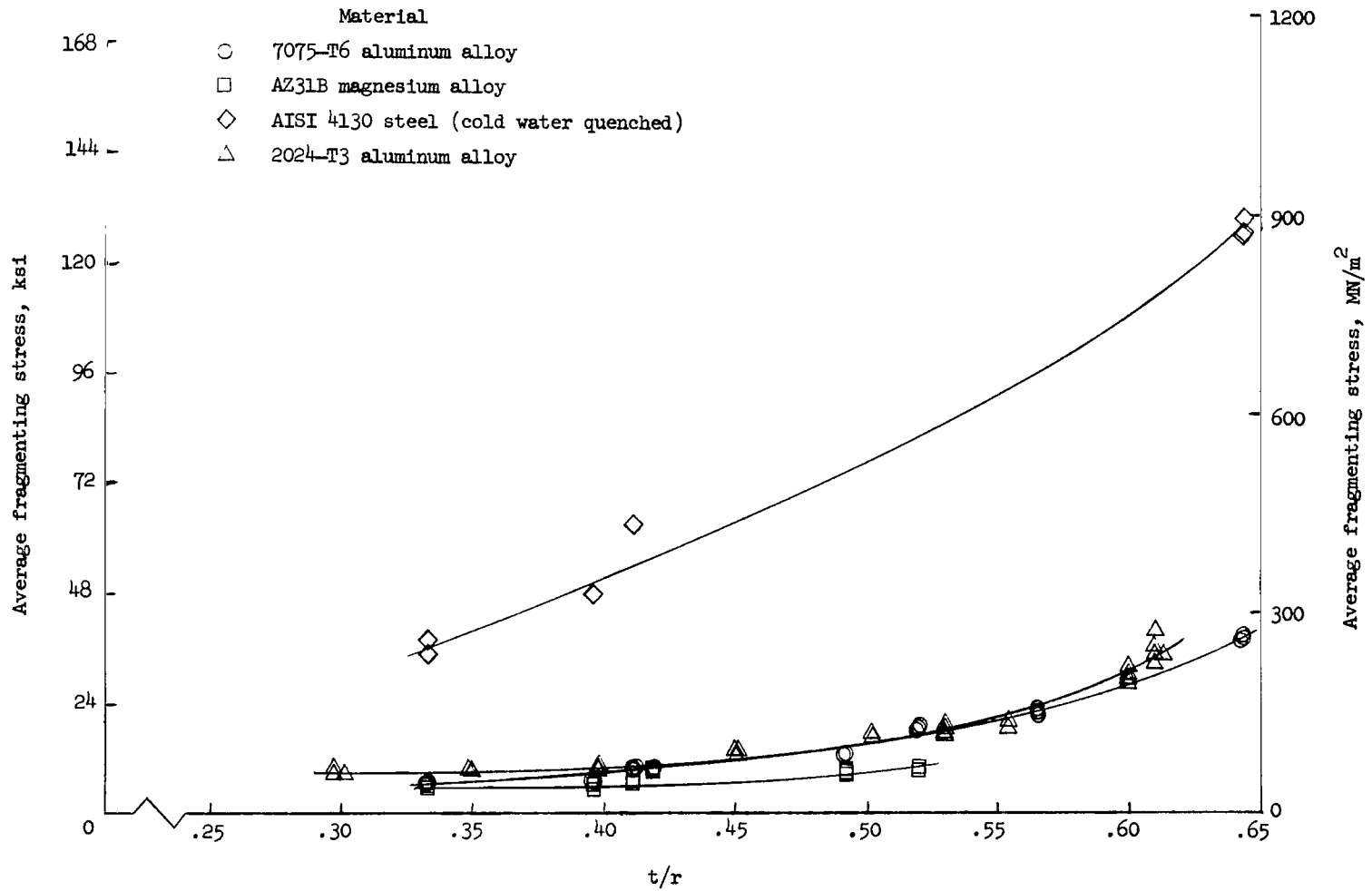
Figure 12.- Variation of average fragmenting stress with tube-wall-thickness—die-radius ratio for four materials. Range of D_i/r from 4.461 to 8.614.
