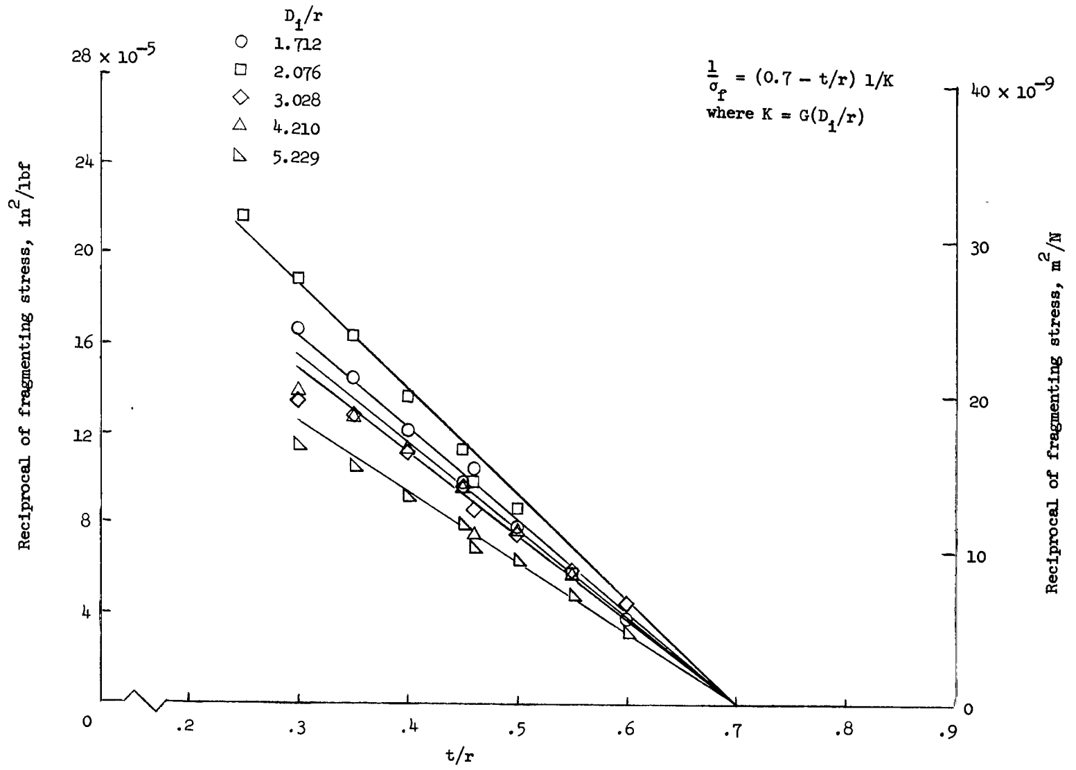
Figure 8.- Reciprocal of the average fragmenting stress as a function of tube-wall-thickness—die-radius ratio for 2024-T3 aluminum alloy.
