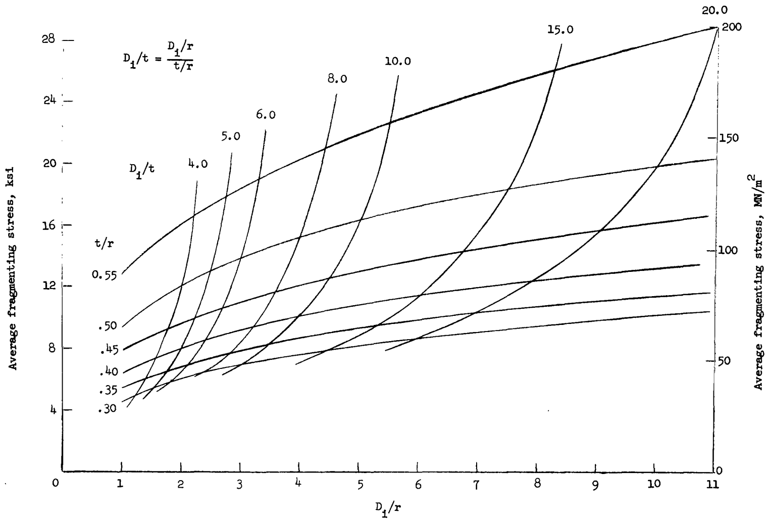
(b) Design chart.
