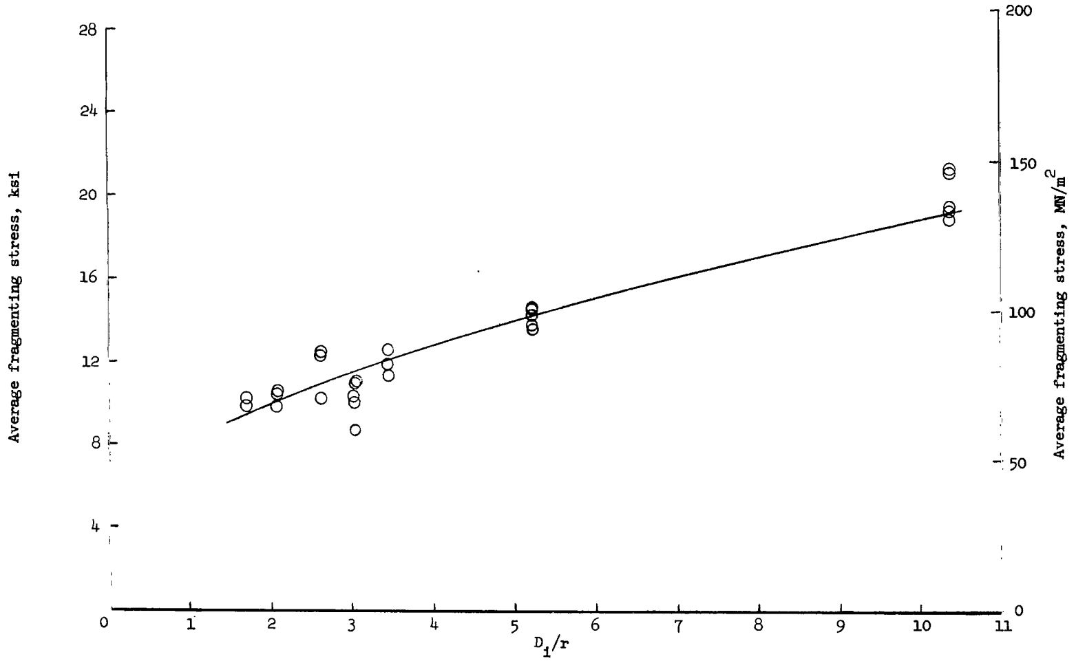
Figure 6.- Variation of average fragmenting stress with tube-inside-diameter—die-radius ratio for 2024-T3 aluminum alloy. Nominal t/r = 0.460 .
