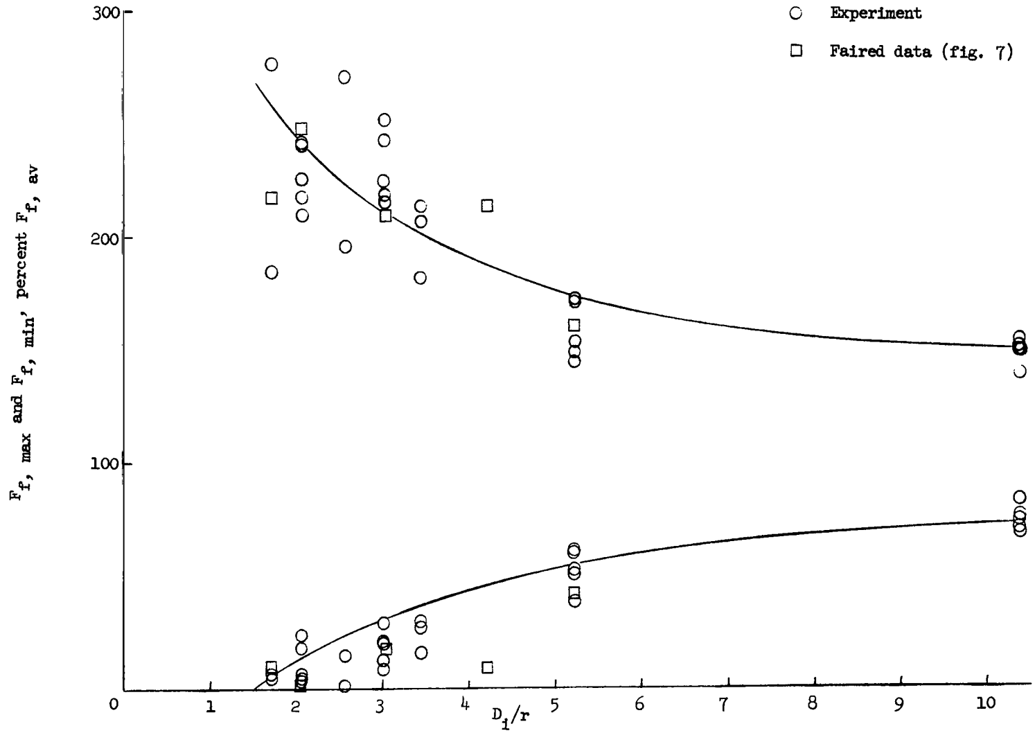
Figure 5.- Variation of maximum and minimum fragmenting force fluctuations with tube-inside-diameter—die-radius ratio for 2024-T3 aluminum alloy. Nominal t/r = 0.460 .
