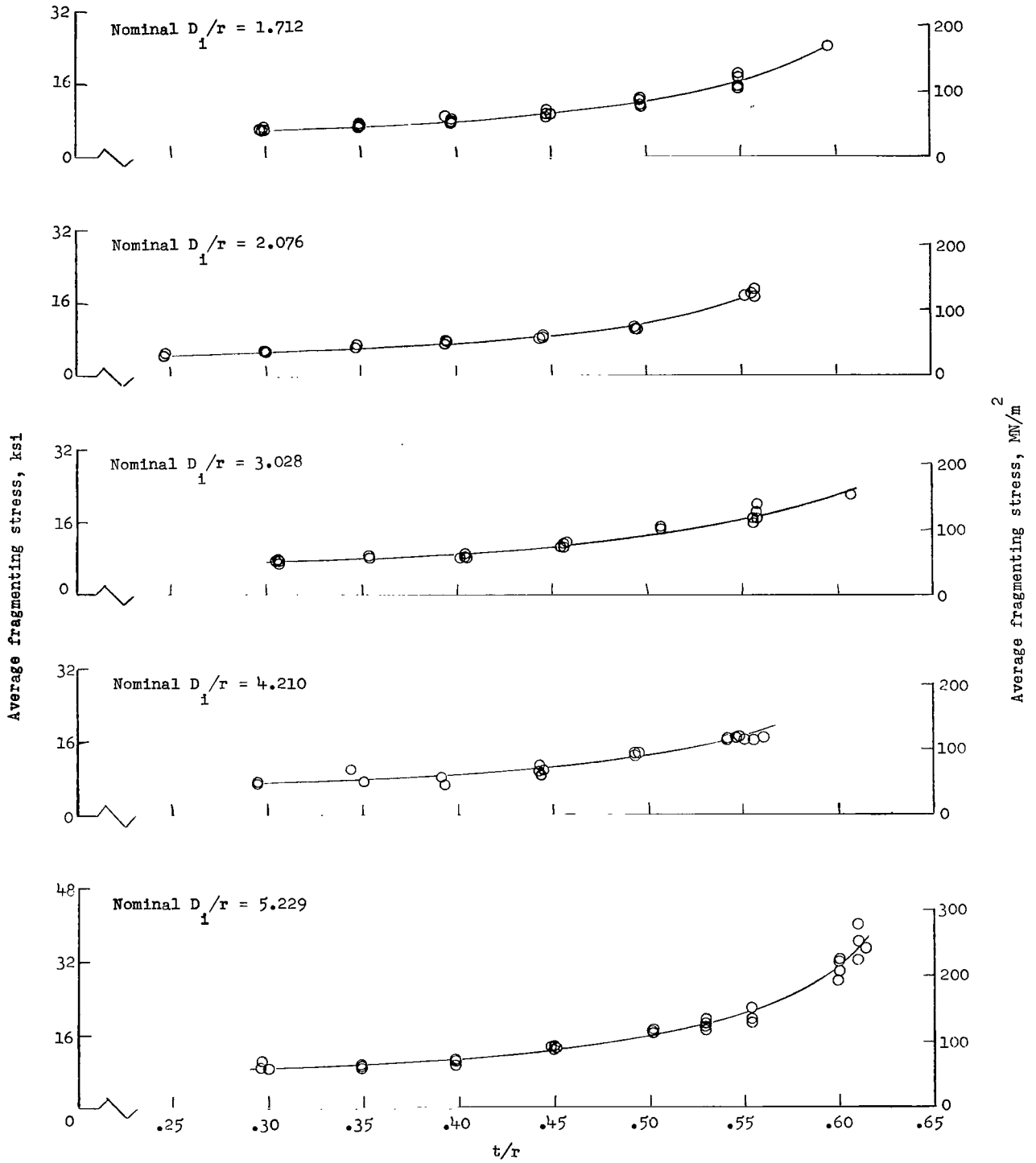
Figure 7.- Variation of average fragmenting stress with tube-wall-thickness—die-radius ratio for 2024-T3 aluminum alloy.
