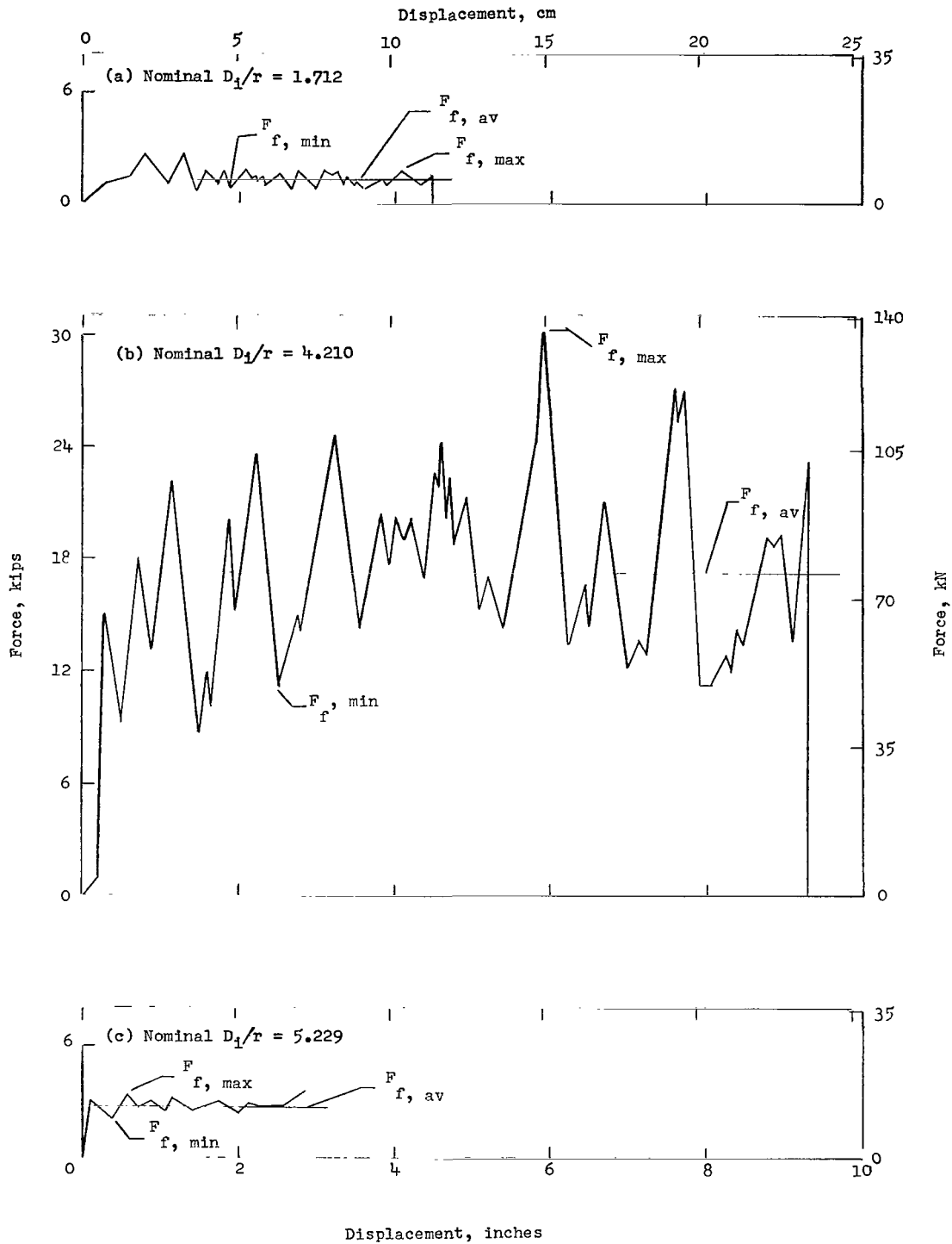
Figure 3.- Typical axial-force variations with displacement for 2024-T3 aluminum alloy. Nominal t/r = 0.300 .
