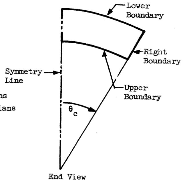
Fig. 6 Configurations of shells in the numerical examples
