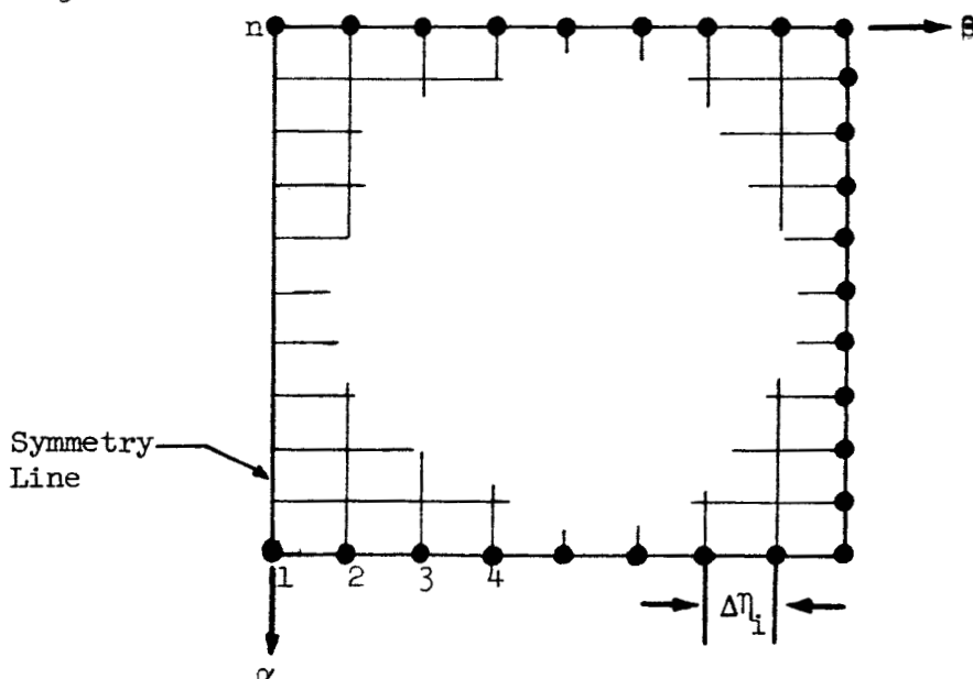
Fig. 5 Boundary of a Shell Segment for a Finite Difference Solution
