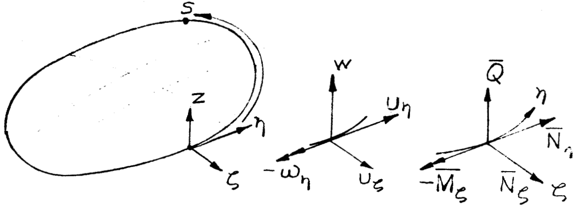
Fig. 3 Boundary Coordinates, Deformations, and Forces
