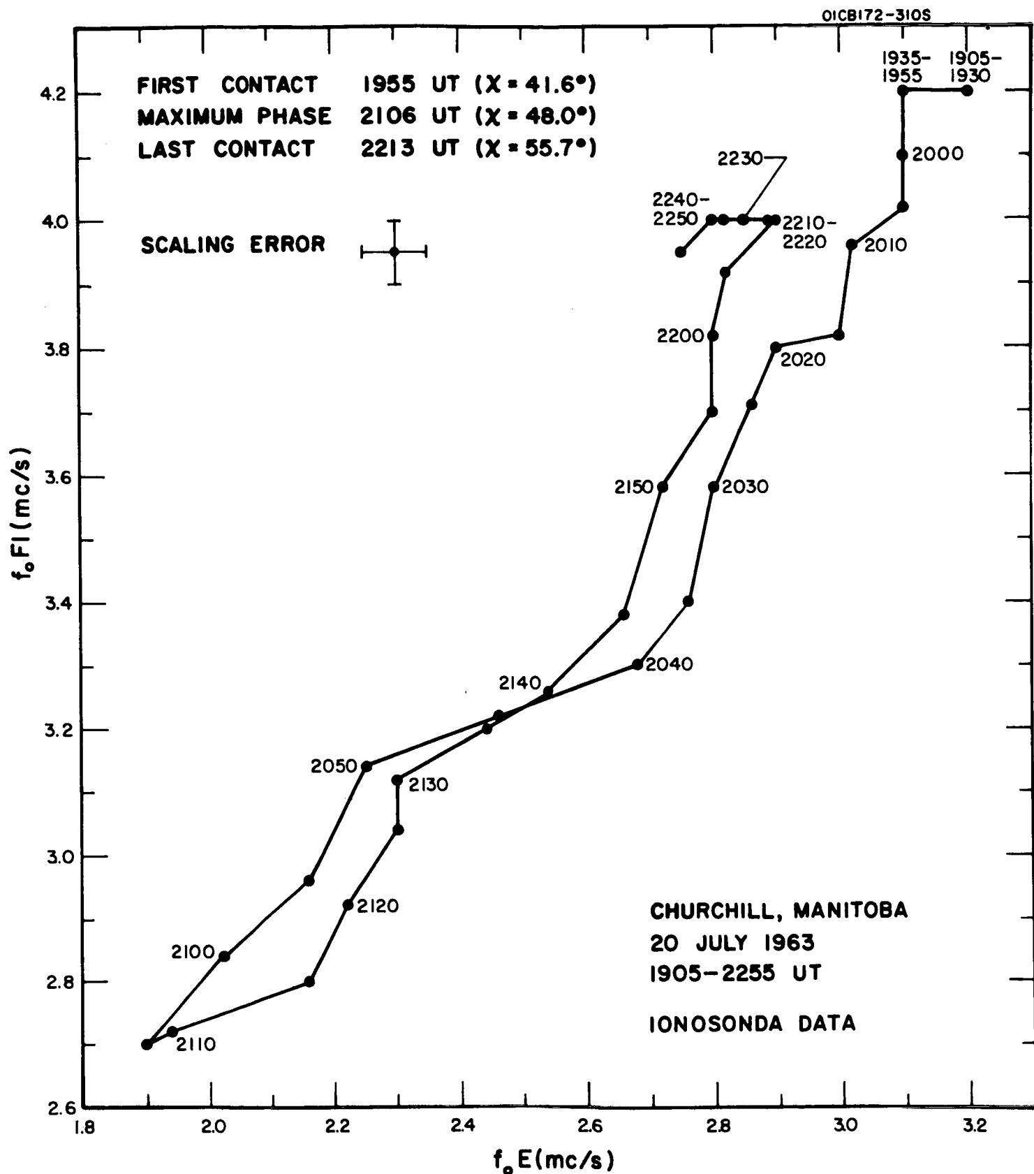
Figure 29. Variation of f_o E and f_o F_1 during the eclipse. Each point is the average of five readings taken at 1-minute intervals.
