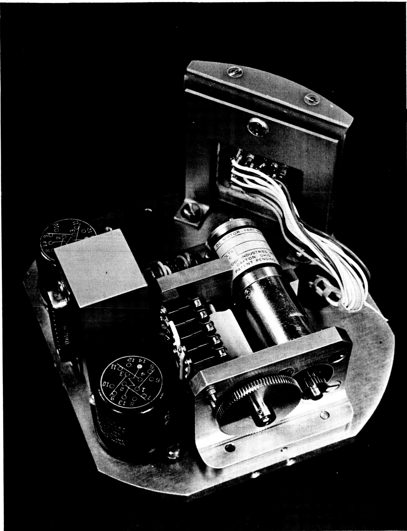
Figure 14. Transfer switch assembly.
