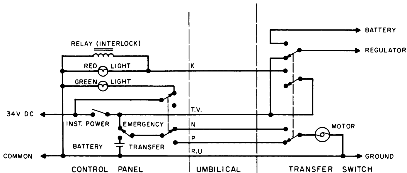
(a) POWER TRANSFER CIRCUIT
