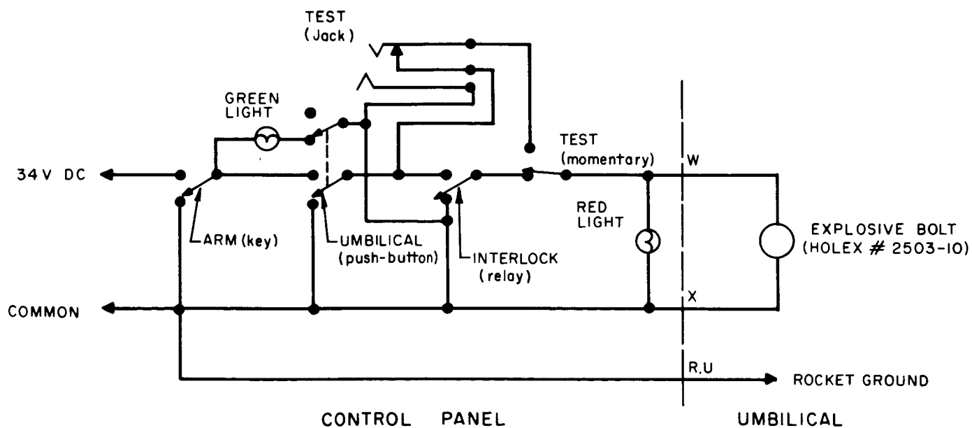
(b) UMBILICAL RELEASE CIRCUIT
