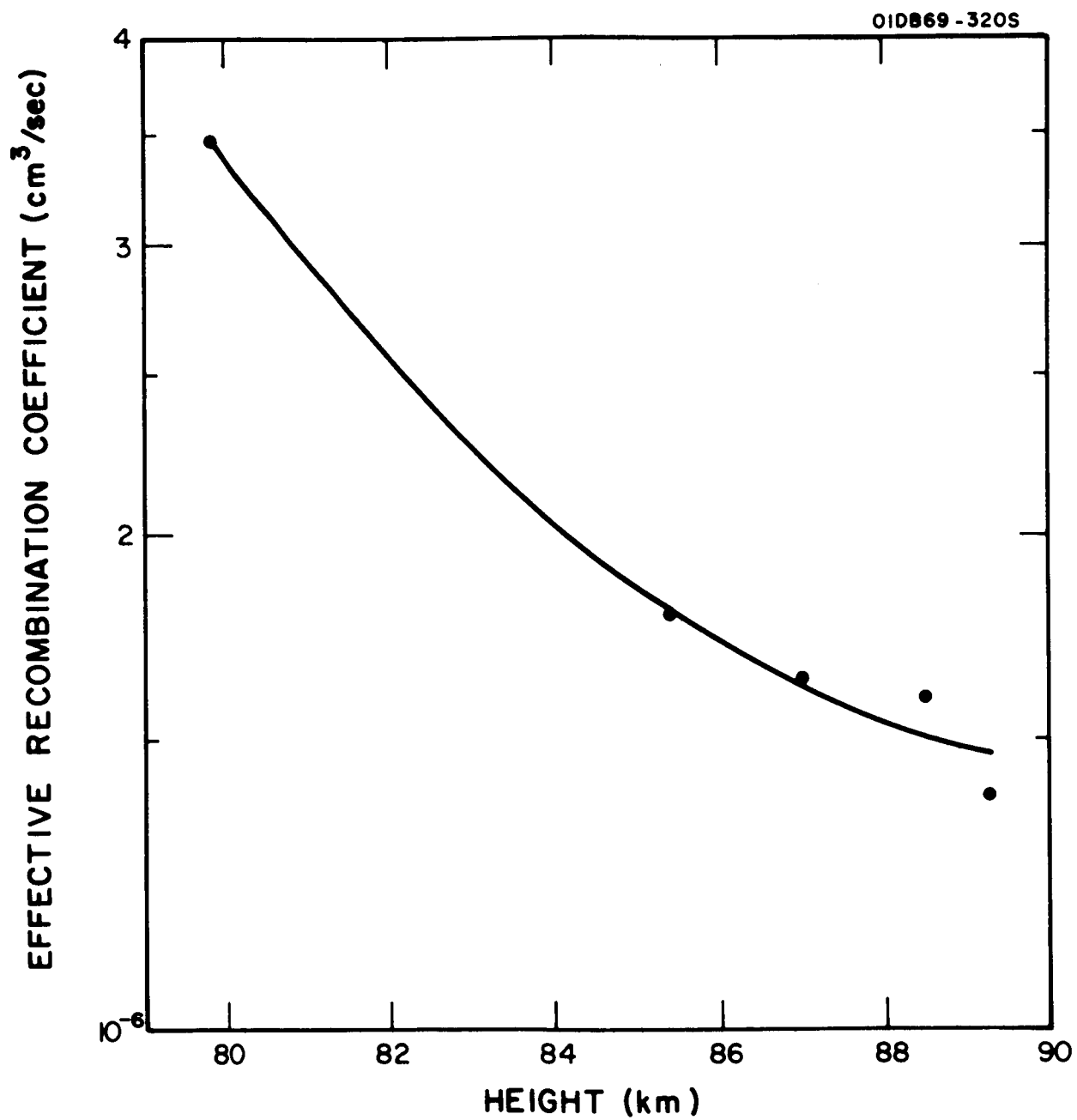
Figure 35. Effective recombination coefficient as a function of height.
