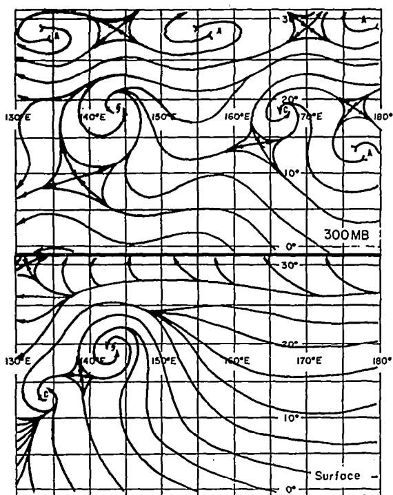
September 19, 1964 (1200 GMT)
