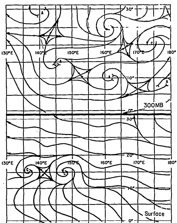
September 17, 1964 (1200 GMT)
