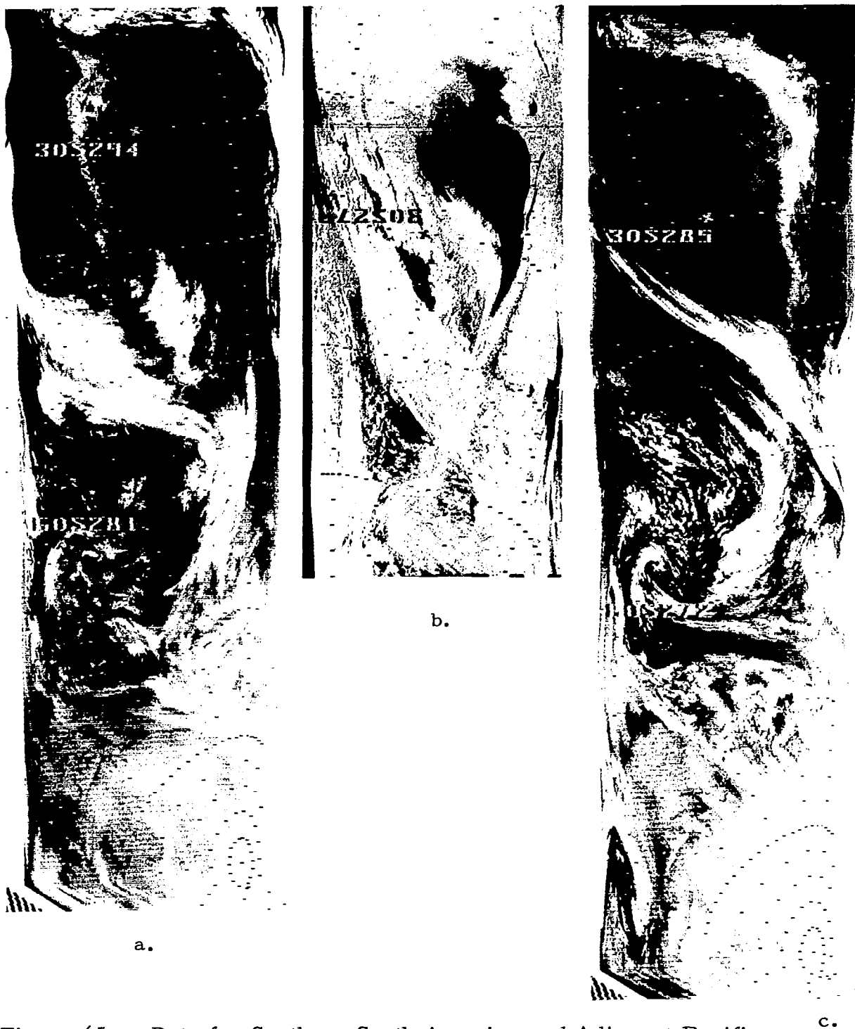
Figure 65. Data for Southern South America and Adjacent Pacific Ocean, 11-12 September 1964
