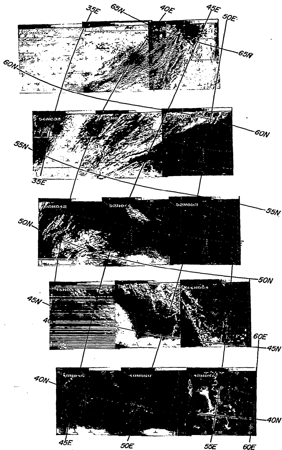
Figure 5-9 AVCS Montage for Part of Orbit 322, About 0745 GMT, 19 September 1964
