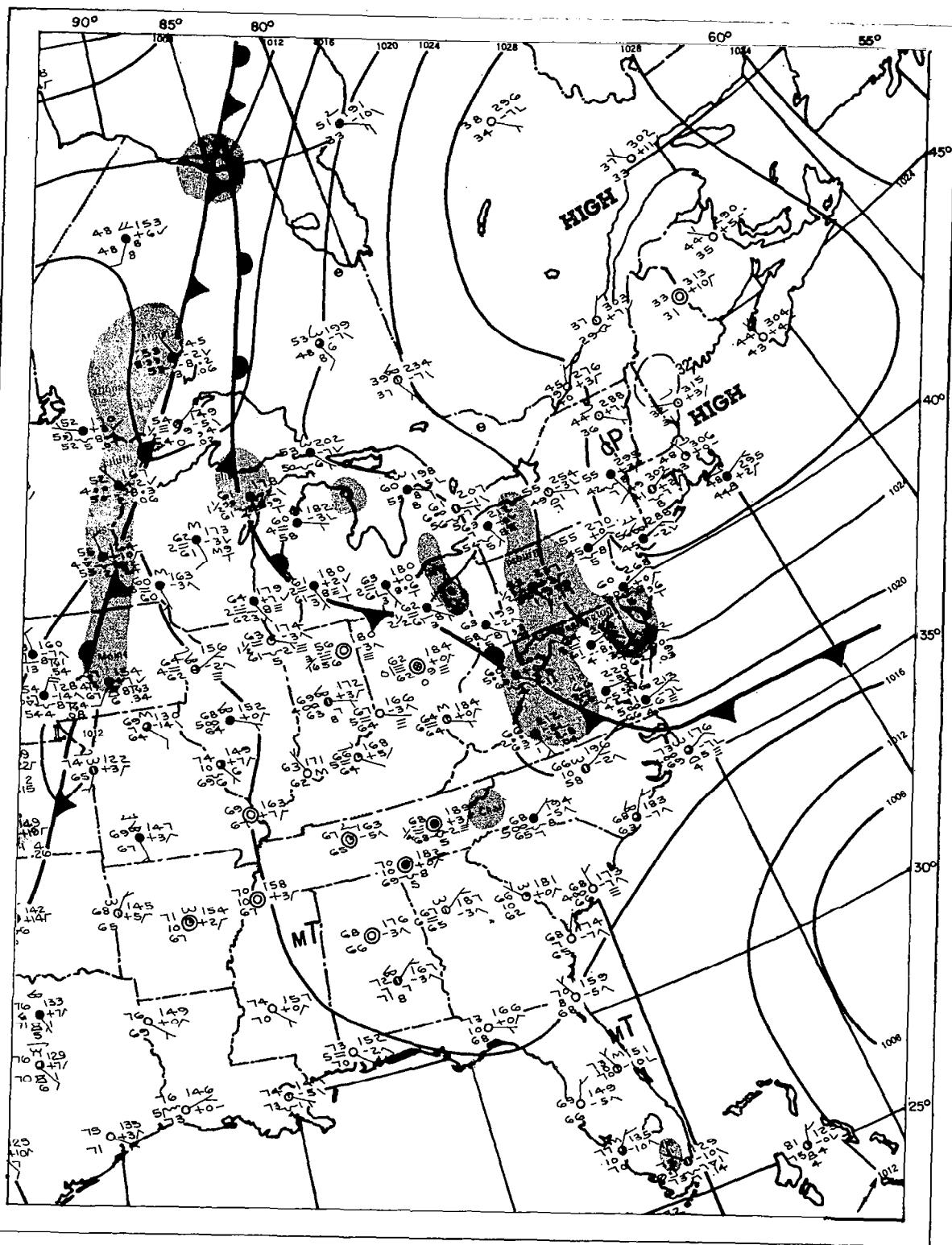
Figure 56. Surface Weather Map at 0600 UT, 20 September 1964
