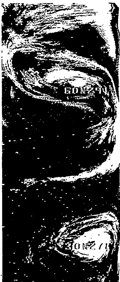
Figure 4-3 HRIR View of a Cloud Vortex, a Frontal Cloud Band, and a Hurricane
