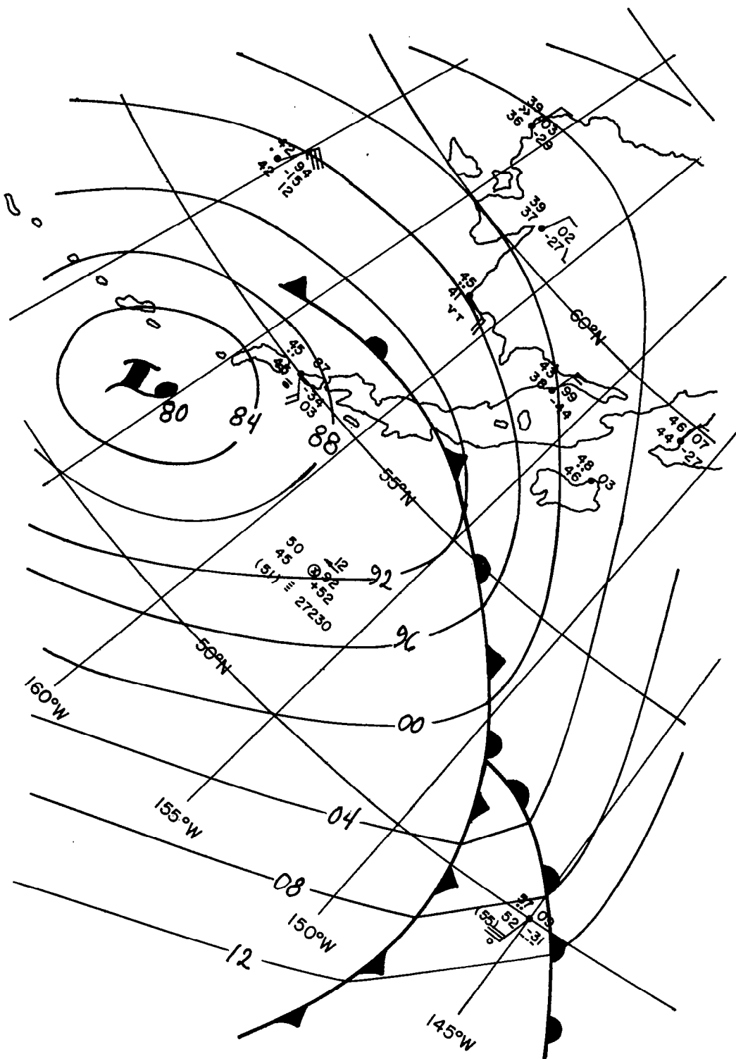
Figure 46. Northwest Portion of NMC North American Surface Analysis, 1200 UT, 20 September 1964
