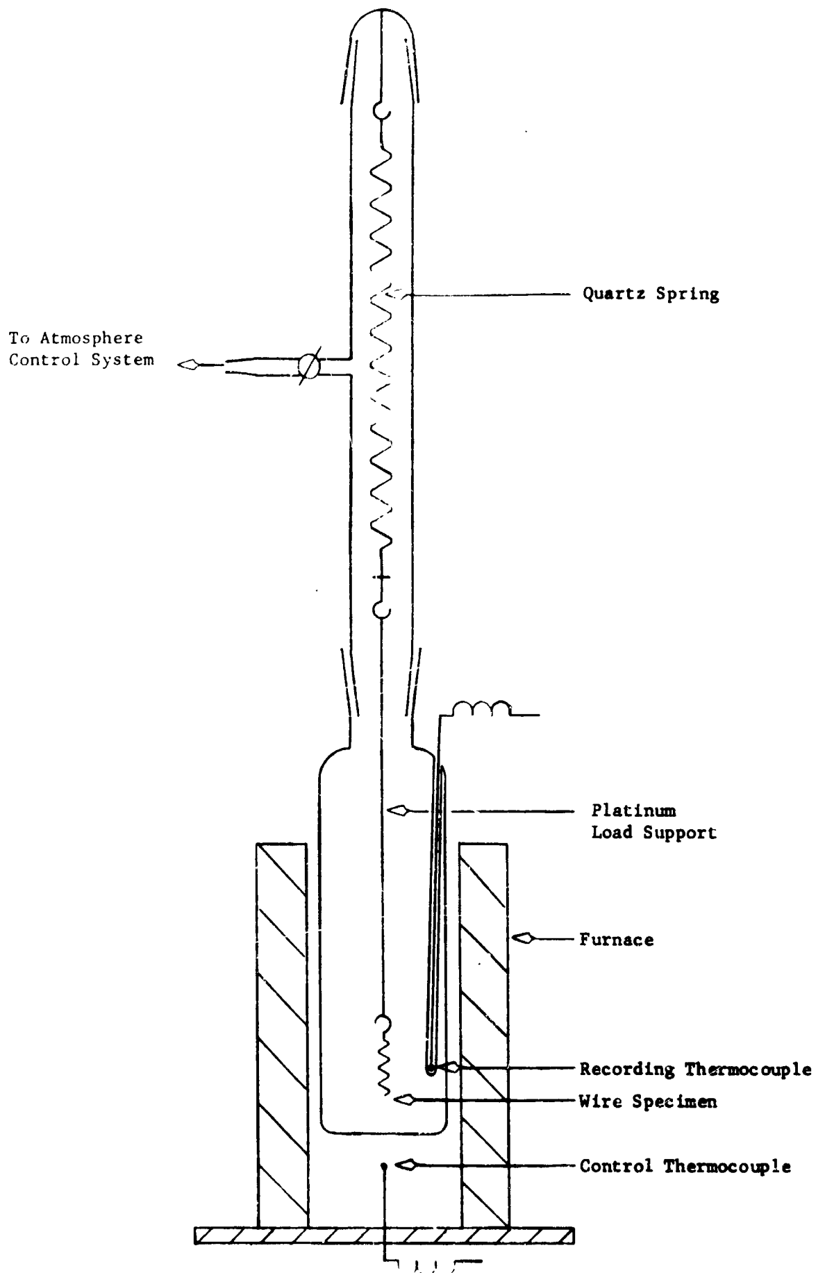
Figure 32: Schematic Diagram of Quartz Spring Balance
