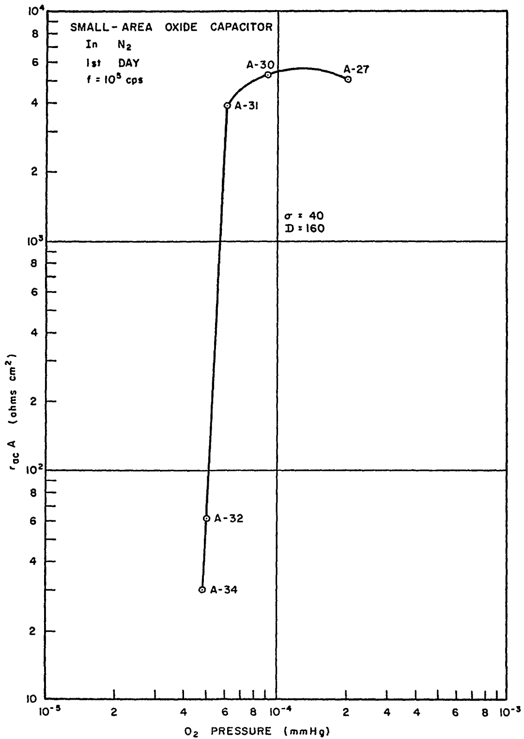
Figure 6. r_{ac} Versus O 2 Pressure
