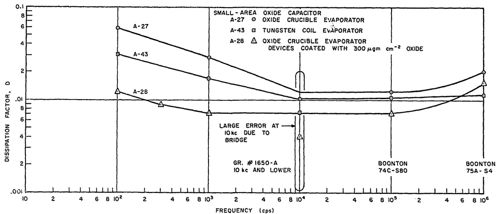
Figure 9. Dissipation Factor Versus Frequency
