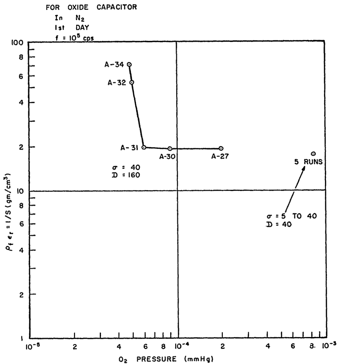
Figure 5. \rho_f \epsilon_r Versus O 2 Pressure
