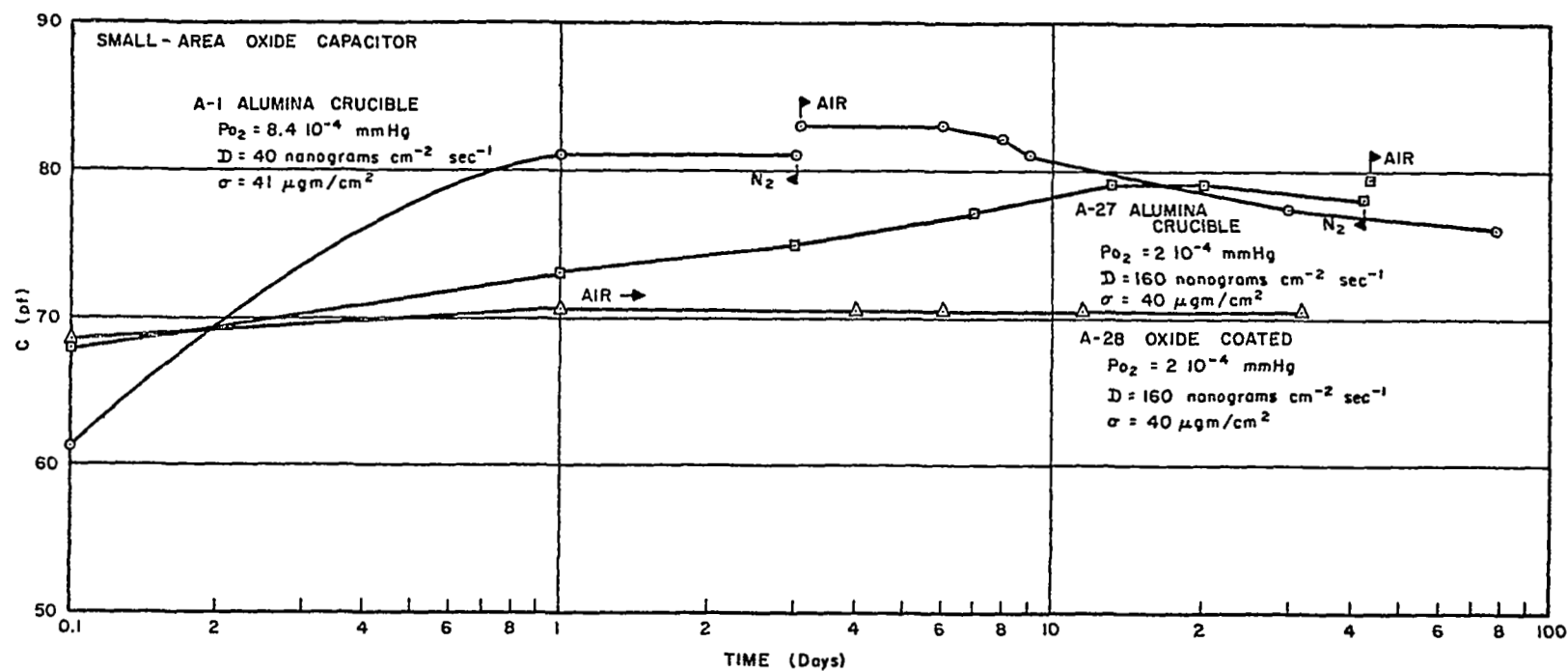
Figure 7. Capacity Versus Time
