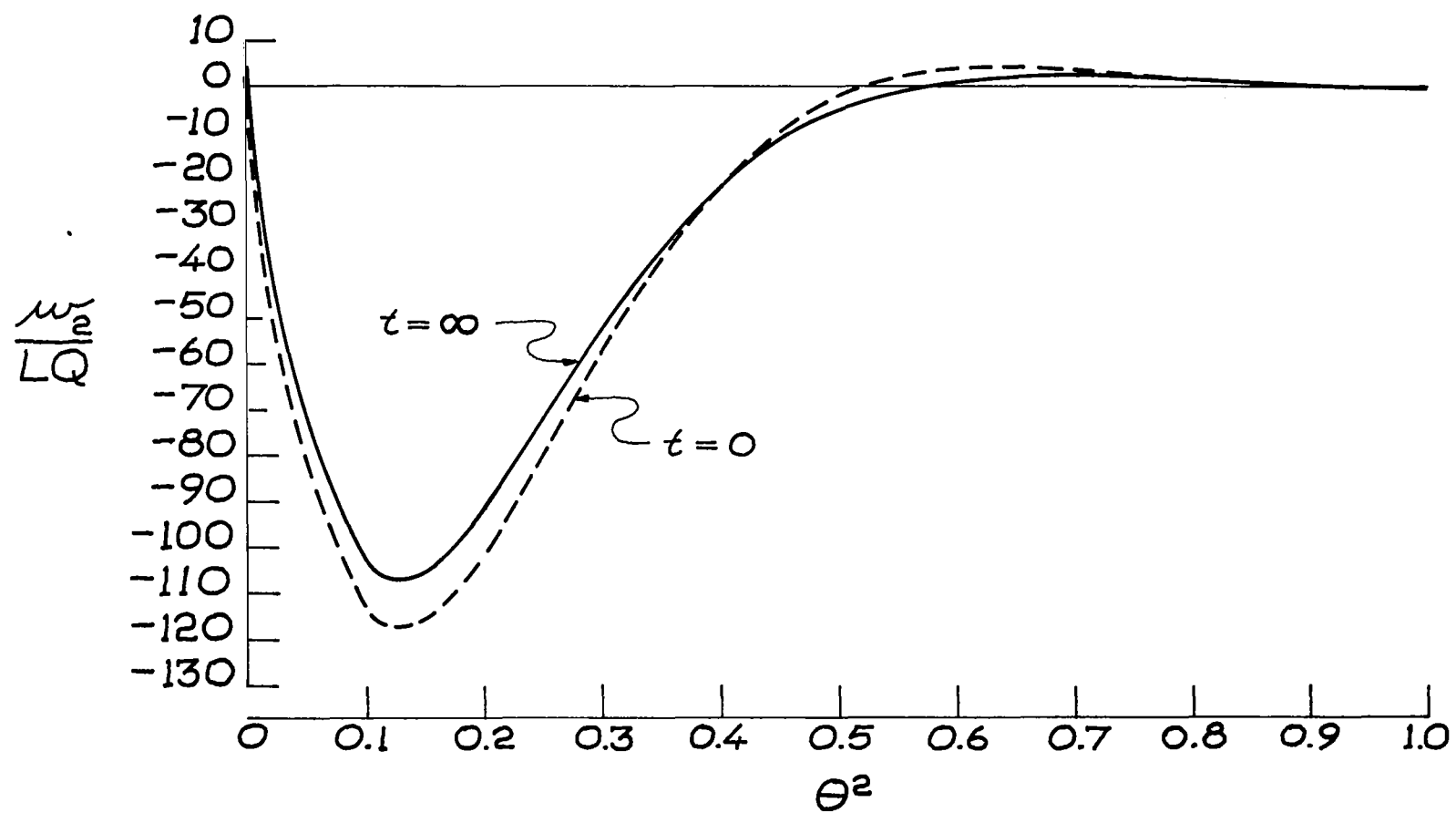
FIG.12, ROTATION
