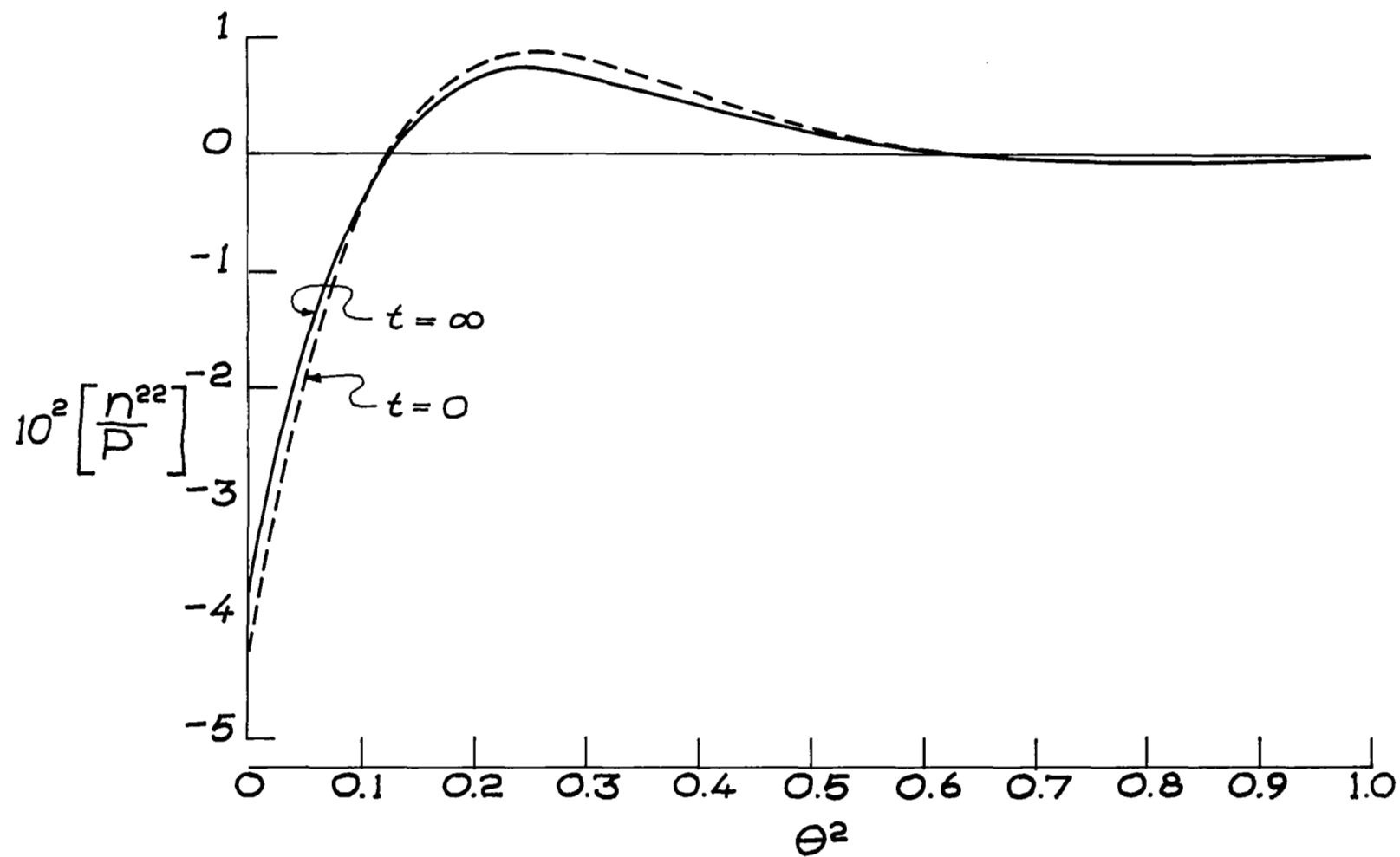
FIG. 14, BENDING MOMENT
