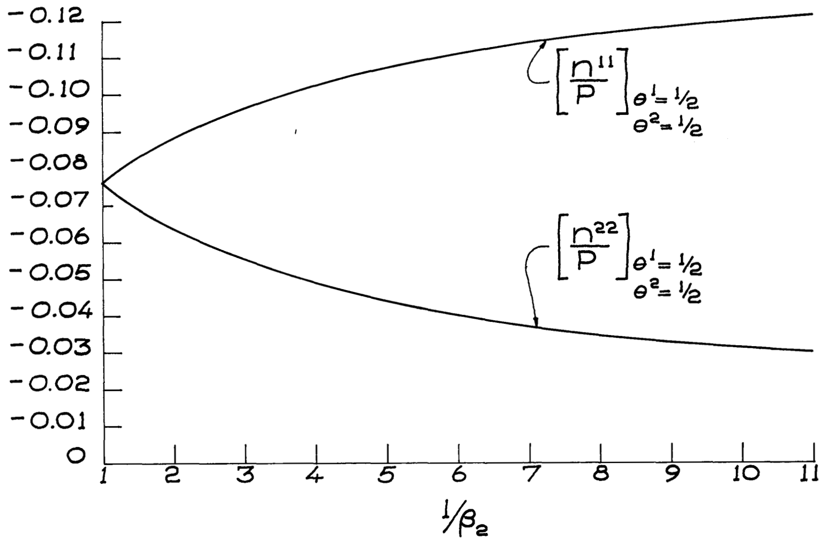
FIG. 7, BENDING MOMENTS
