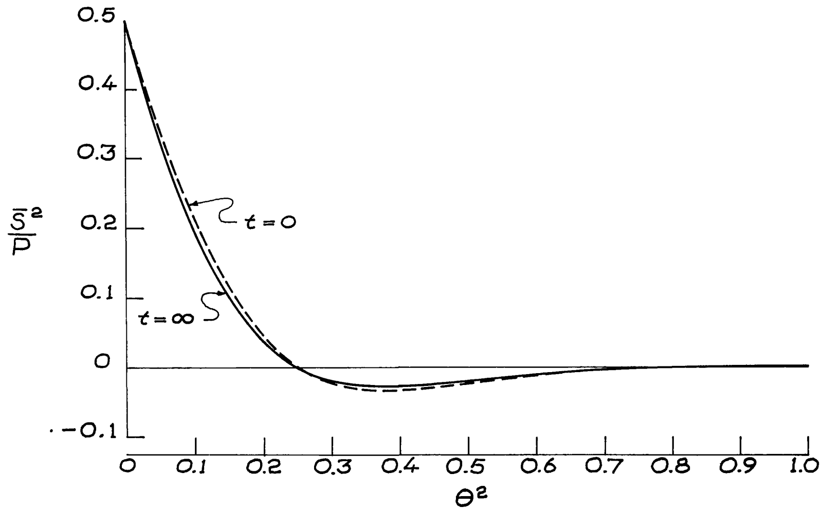
FIG. 13, SHEAR RESULTANT
