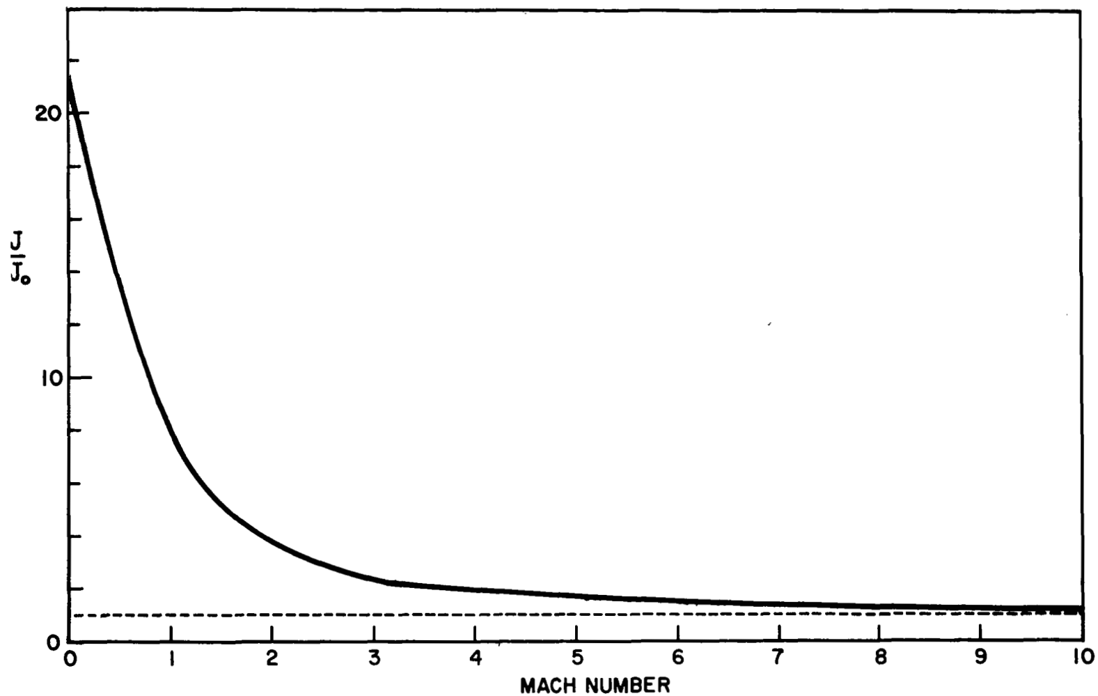
FIGURE 5. CURRENT vs MACH NUMBER POTENTIAL = -5.1 VOLTS
