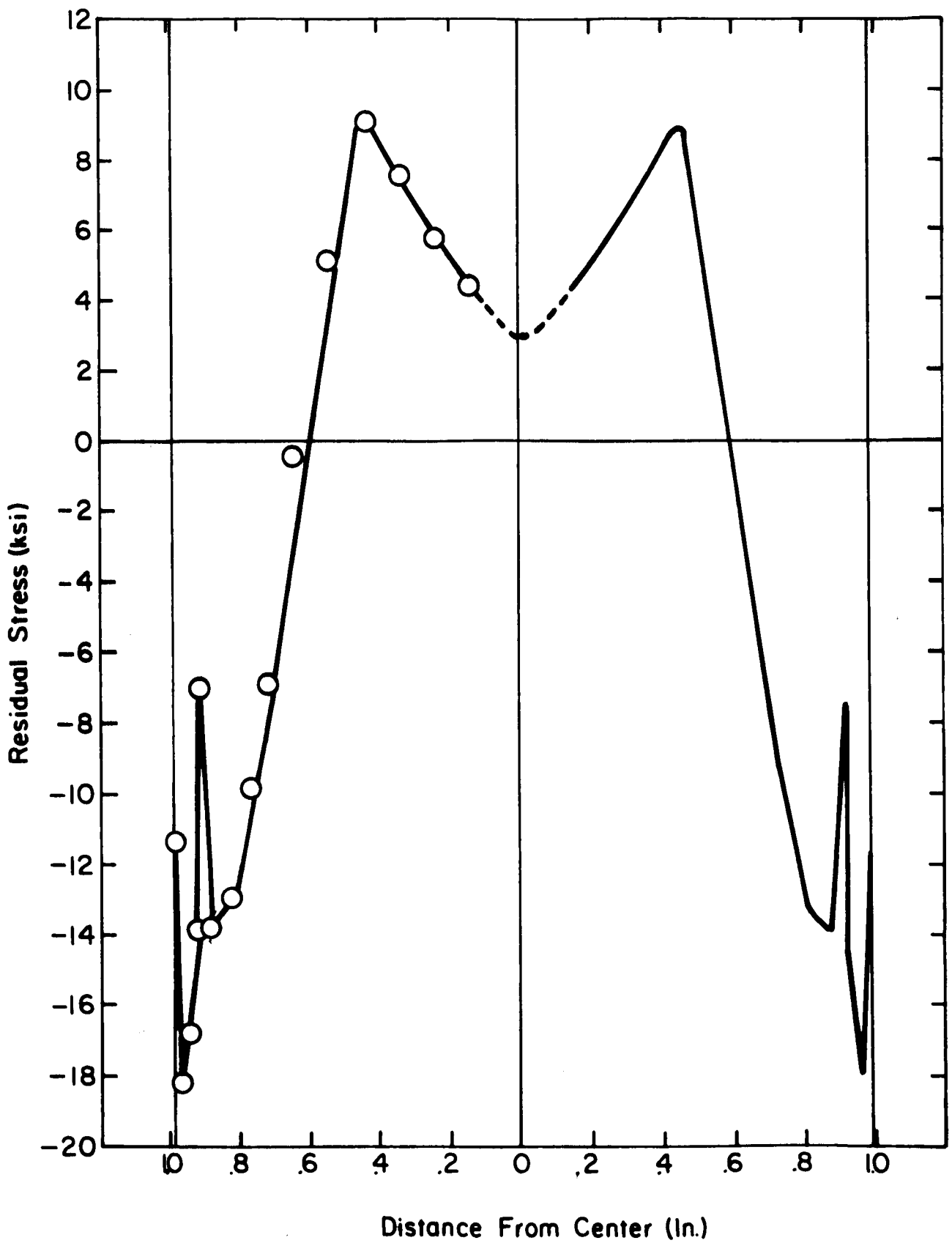
Figure 44. Residual Stress Distribution Through the Thickness in 2 inch Thick 2219-T6 Plate as Heat Treated.
