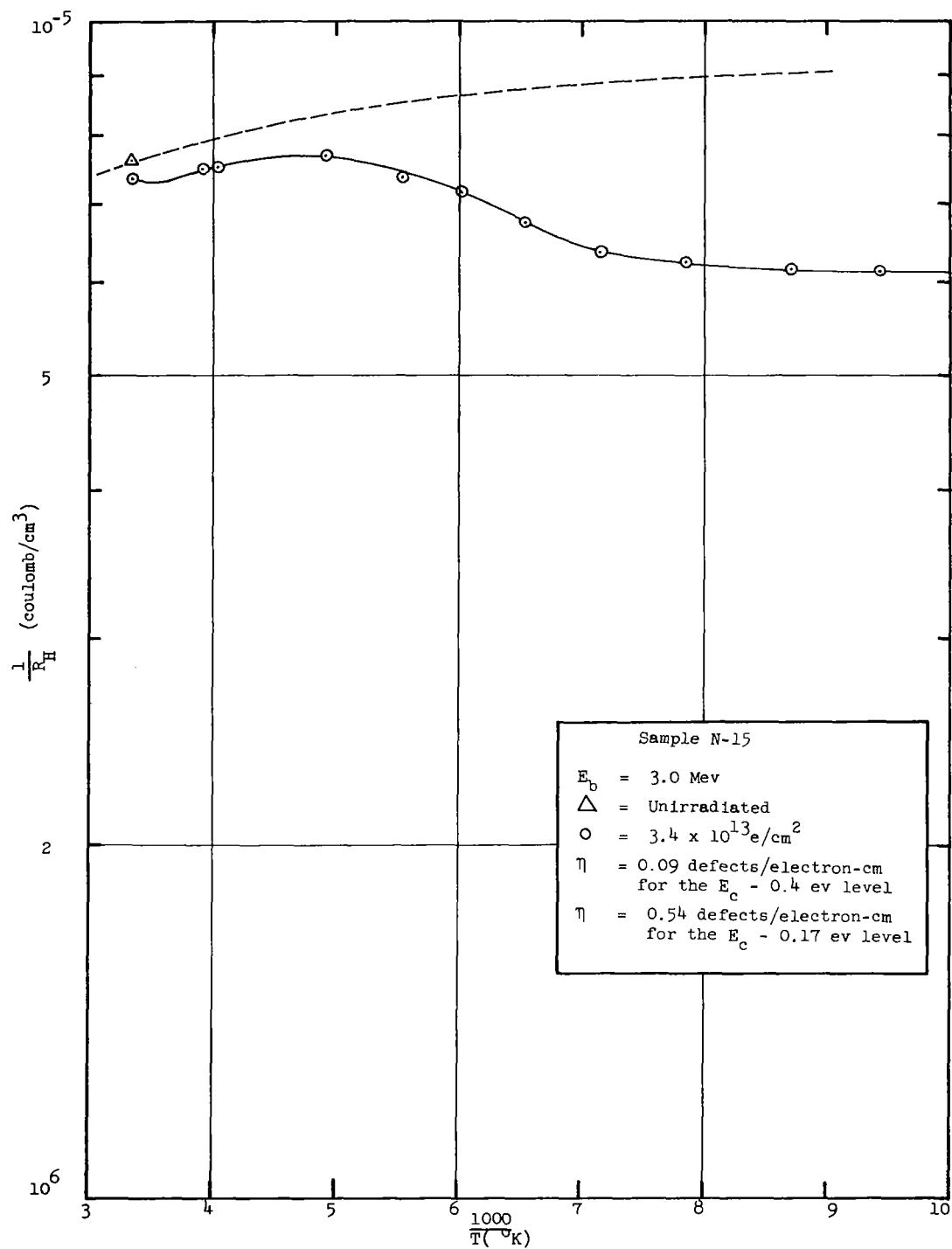
Figure 3. Temperature Variation of Reciprocal Hall Coefficient for 100 Ω-cm, n-type Silicon before and after Electron Irradiation (3.0 Mev)
