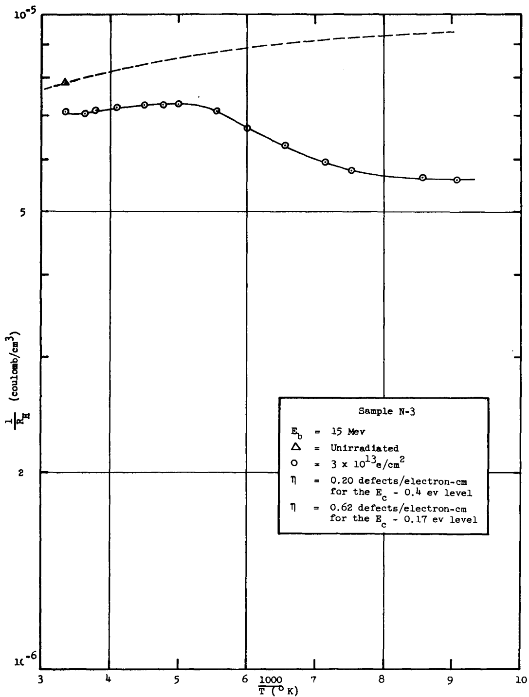
Figure 5. Temperature Variation of Reciprocal Hall Coefficient for 100 \Omega -cm, n-type Silicon before and after Electron Irradiation (15 Mev)
