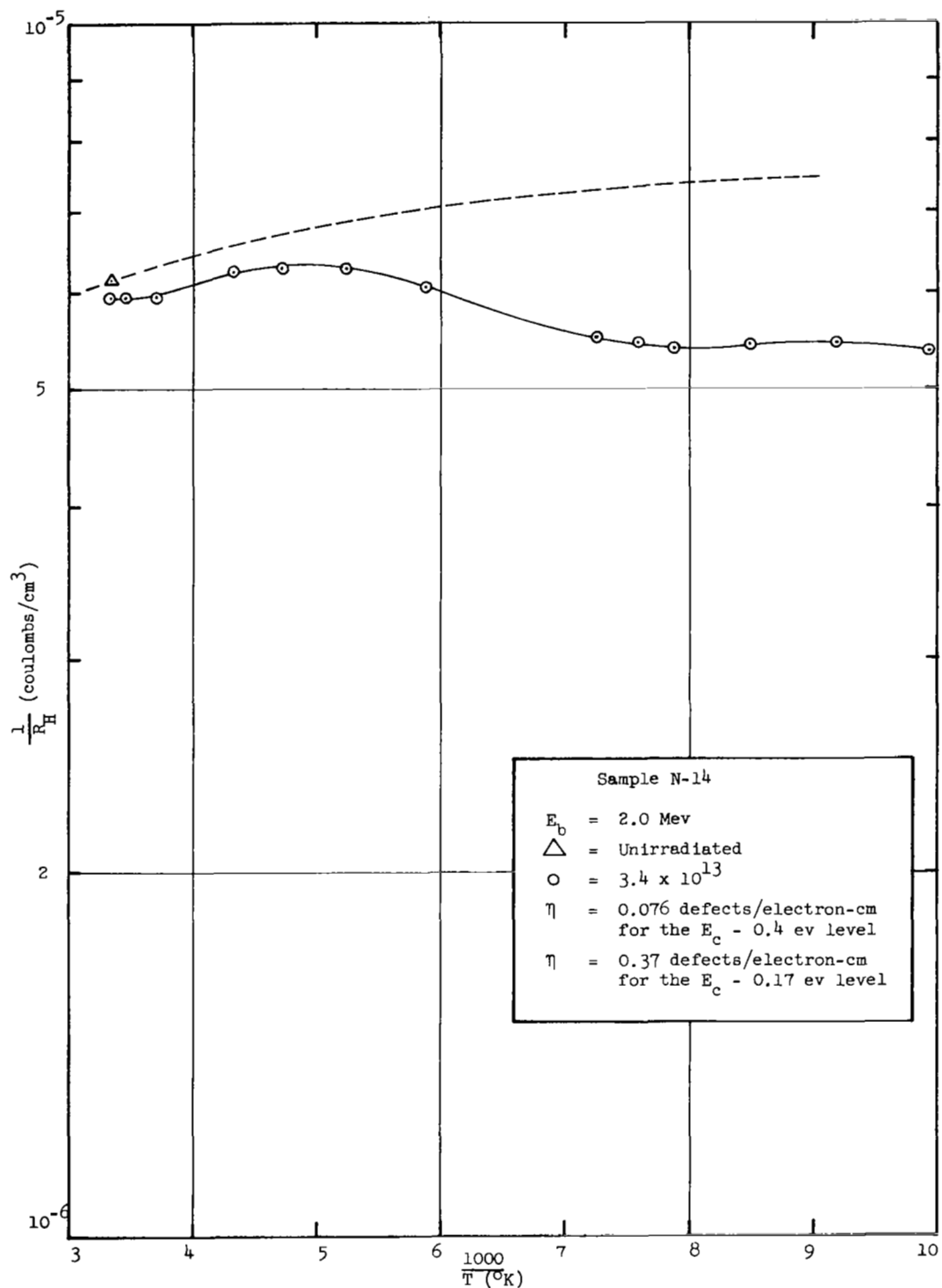
Figure 2. Temperature Variation of Reciprocal Hall Coefficient for 100 Ω -cm, n-type Silicon before and after Electron Irradiation (2.0 Mev)
