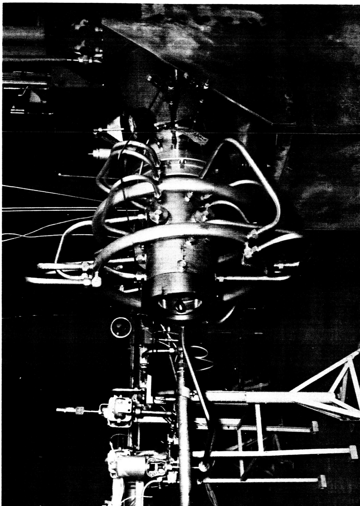
Figure 5 Test Stand, Motor-Driven Tester Page 9
