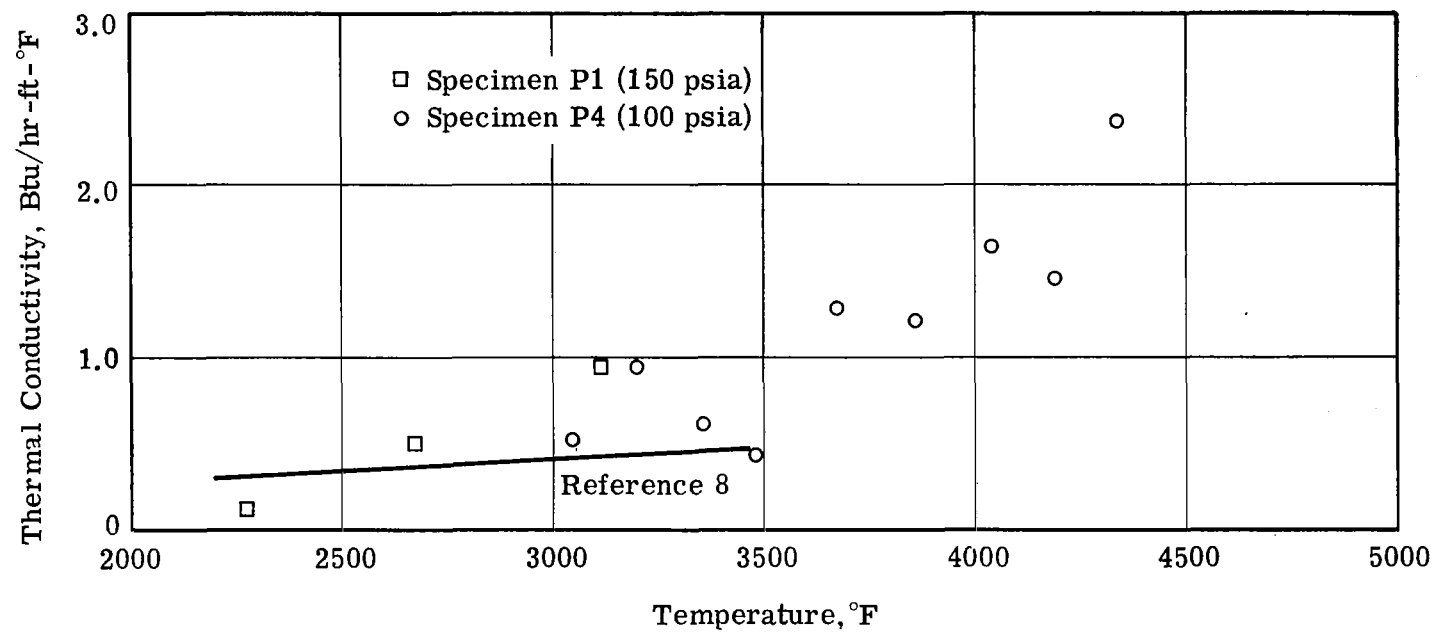
Fig. 18 — Helium Thermal Conductivity
