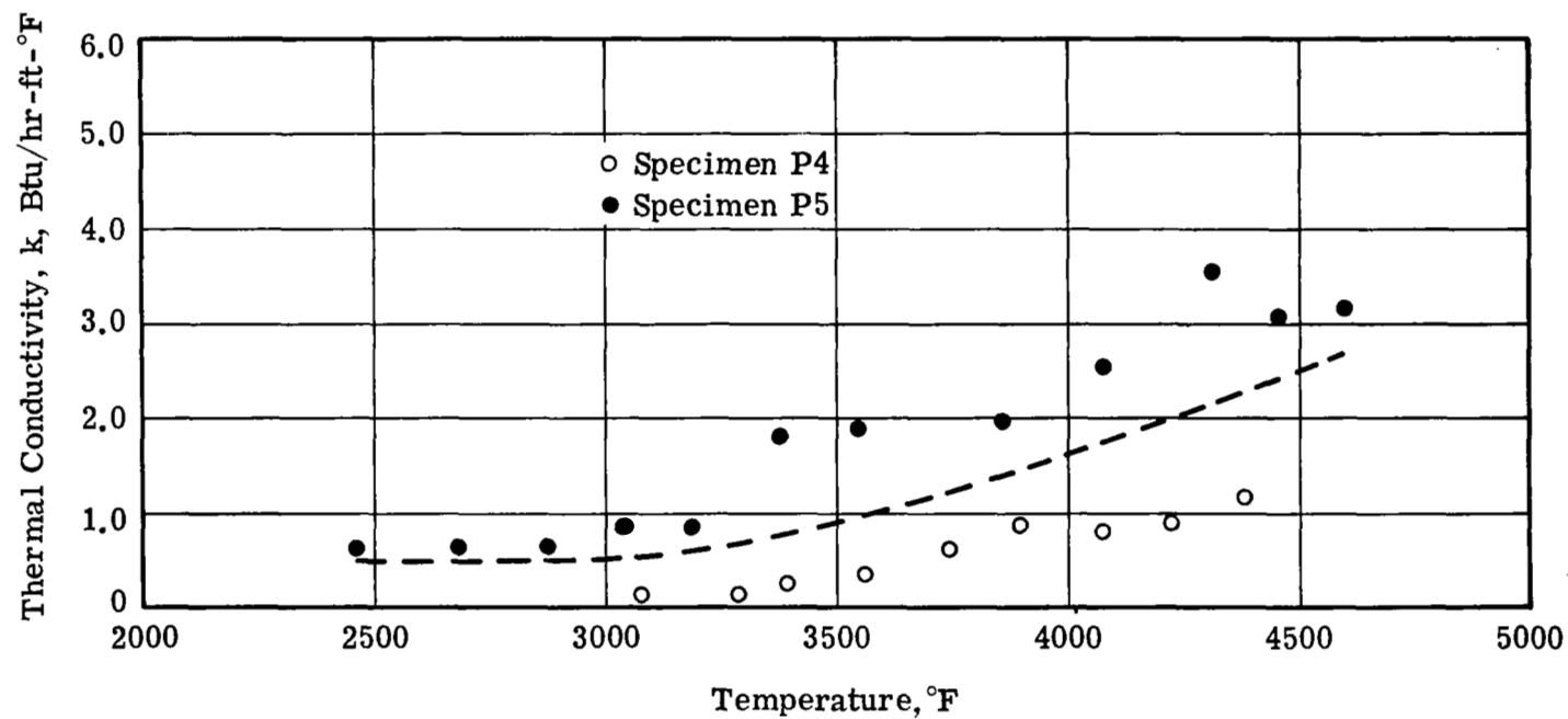
Fig. 10 — Hydrogen Thermal Conductivity, 100 psia
