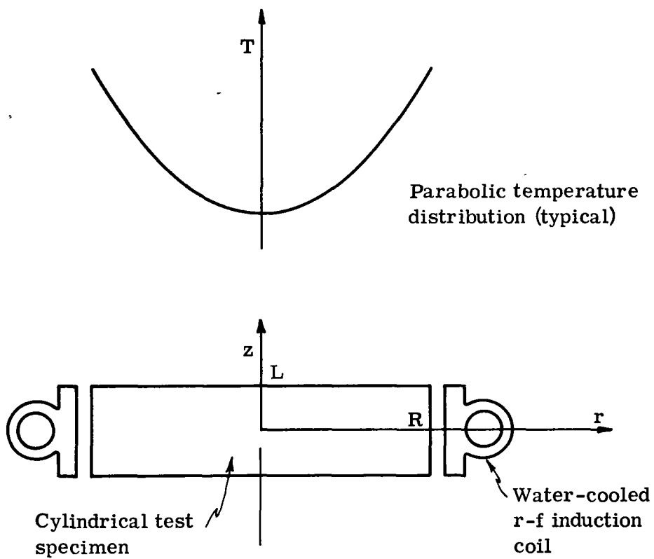
Fig. 5 — Specimen Arrangement
