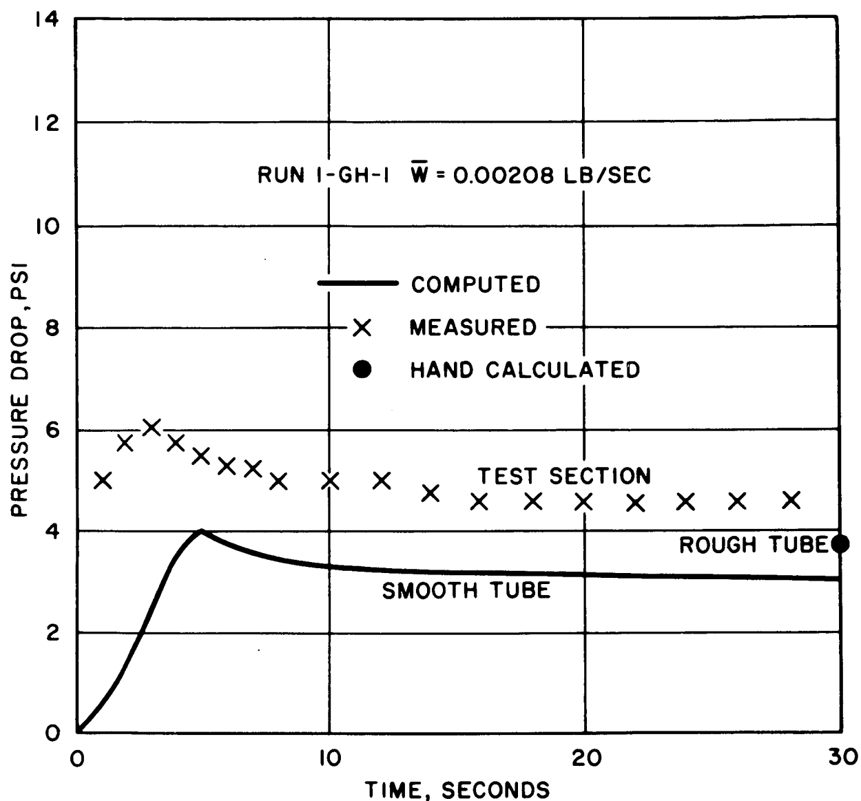
FIGURE II-COMPARISON OF CALCULATED AND MEASURED PRESSURE DROPS ACROSS THE TEST SECTION
