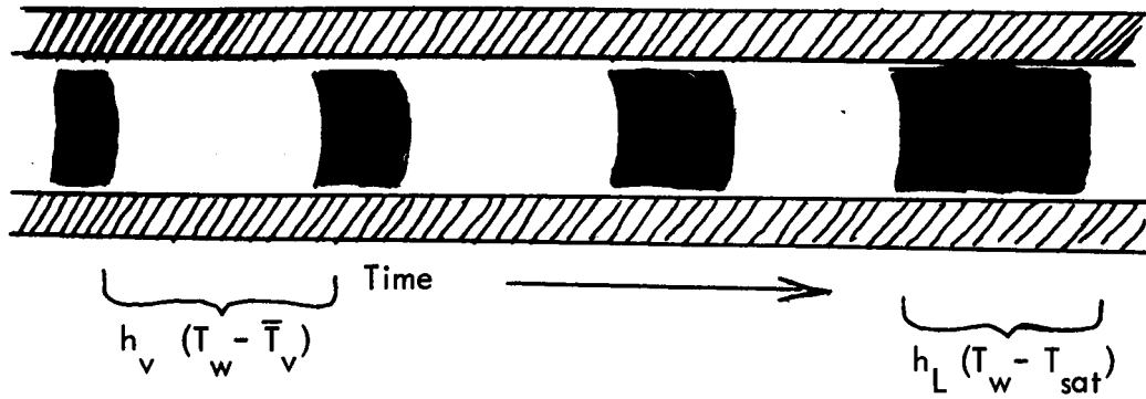
HEAT TRANSFER MODEL FOR THE FILM BOILING REGIME
