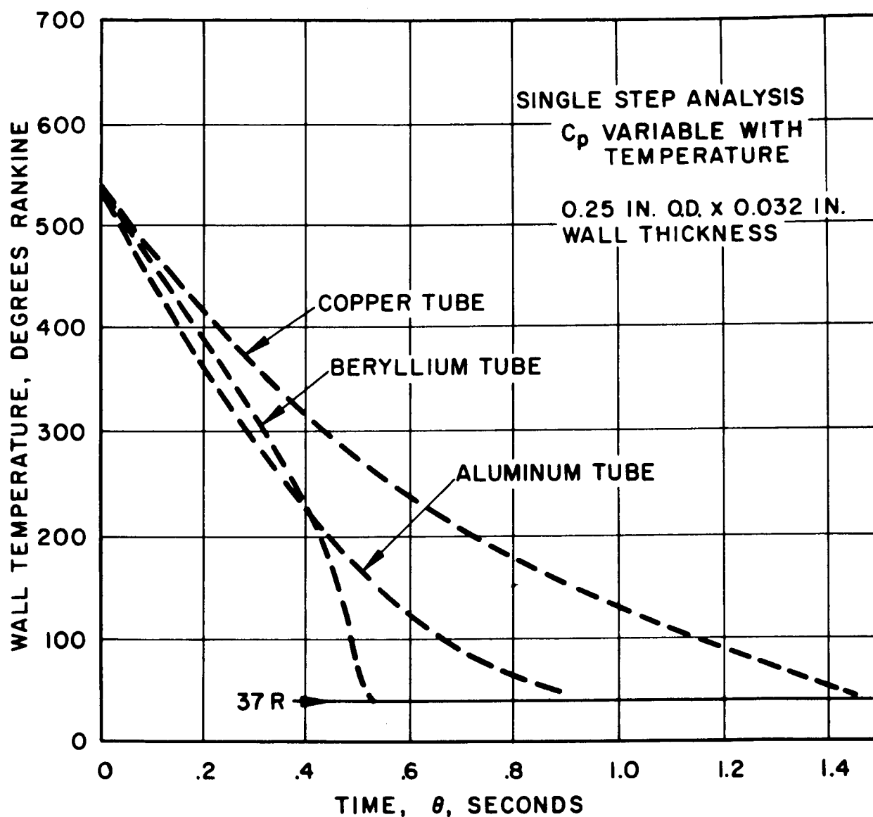
FIGURE 5 - RESULTS OF SINGLE STEP ANALYSIS OF TRANSIENT TEMPERATURE HISTORY WITH HYDROGEN FLOW IN A THIN WALLED TUBE
