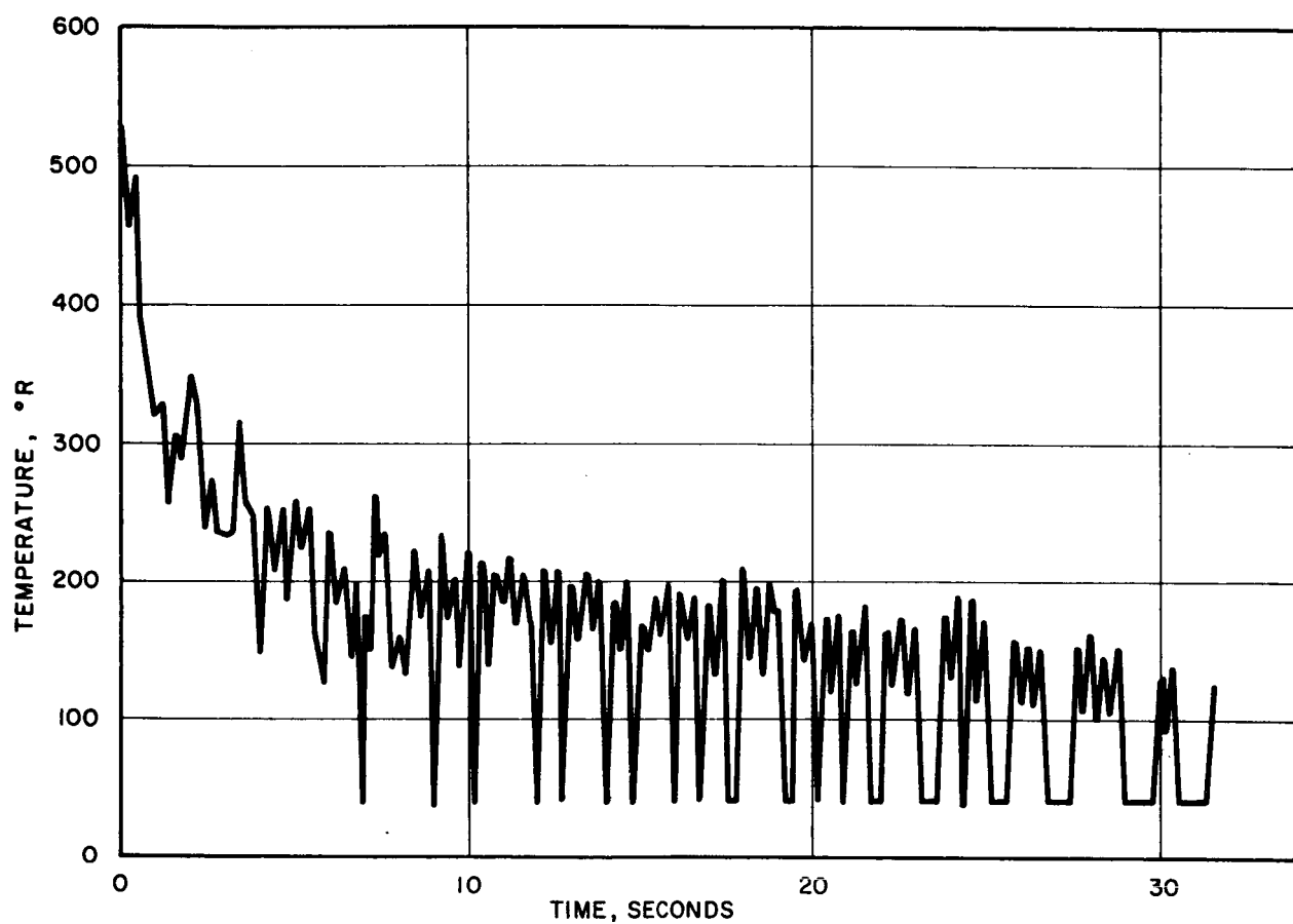
FIGURE 12- TYPICAL INLET STREAM TEMPERATURE HISTORY
