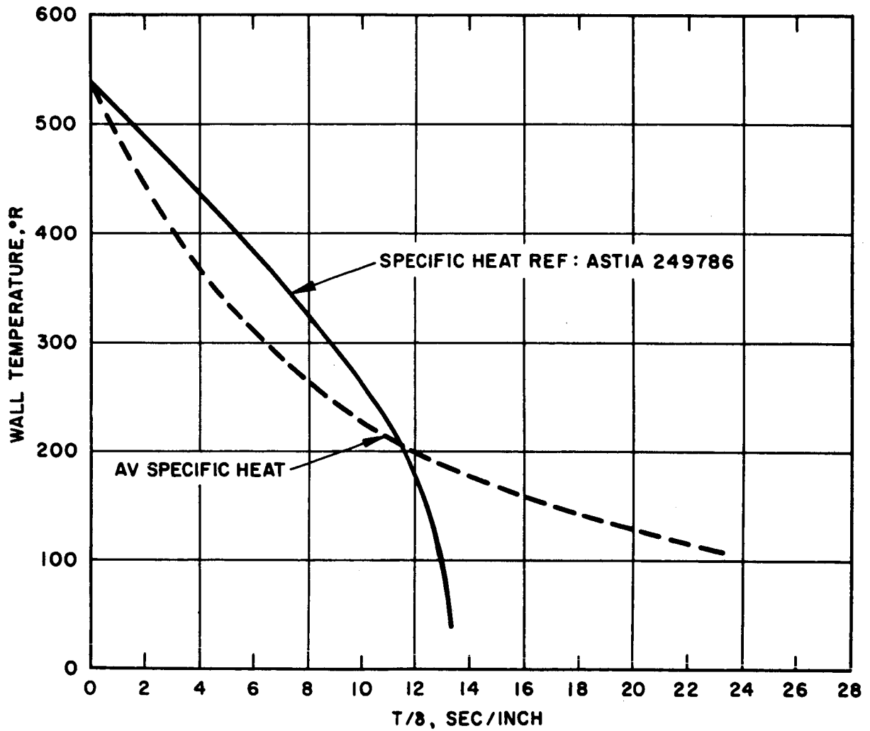
FIGURE 24 - TEMPERATURE HISTORY OF LUMPED PARAMETER SYSTEM BERYLLIUM TUBE (8 INCH WALL THICKNESS)
