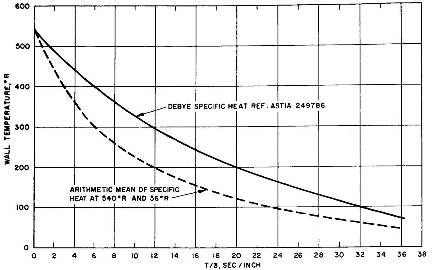
FIGURE 25. TEMPERATURE HISTORY OF LUMPED PARAMETER SYSTEM. COPPER TUBE ( \frac{3}{8} IN. WALL THICKNESS)
