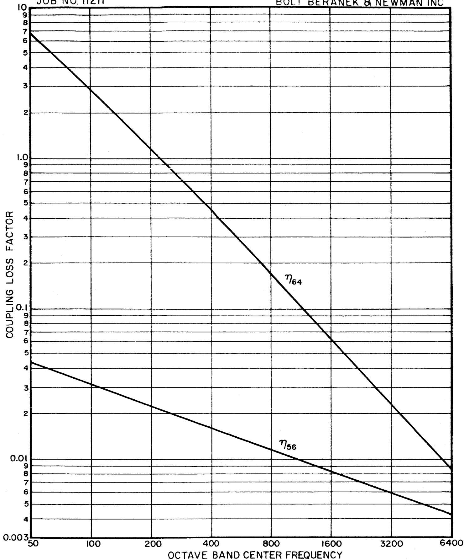
FIG. 7 COUPLING LOSS FACTORS FOR OGO MODEL
