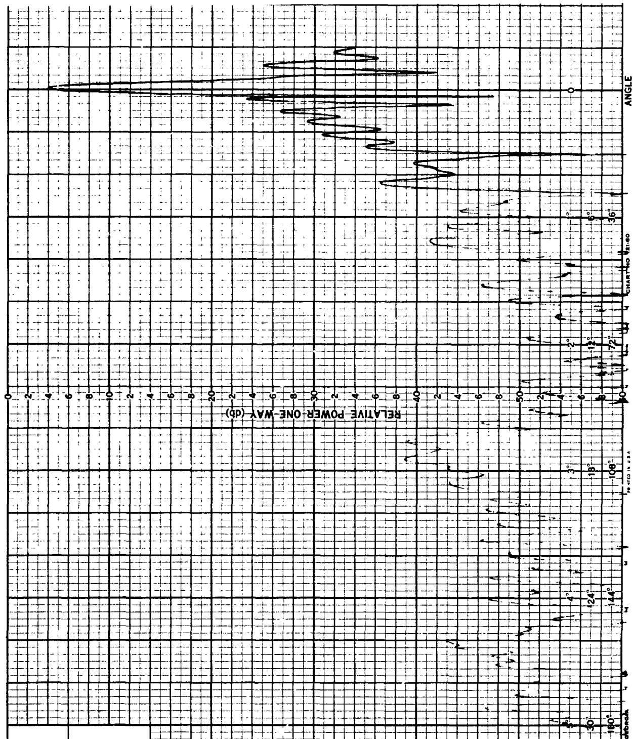
FIG. 82 - 1700 MC, E\theta , FEED TILTED DOWN
