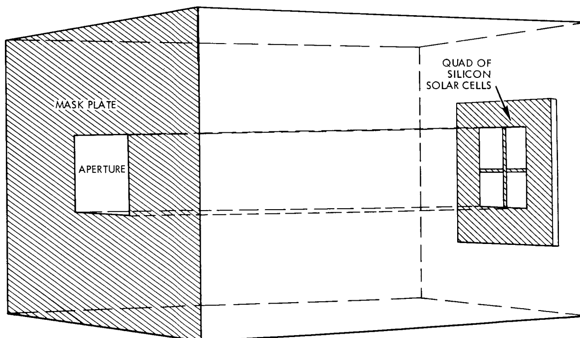
Figure 34. Fine Sun Sensors
