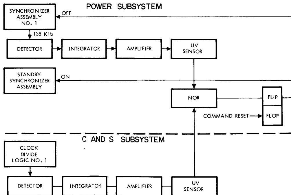
Figure 11. Switching Logic
