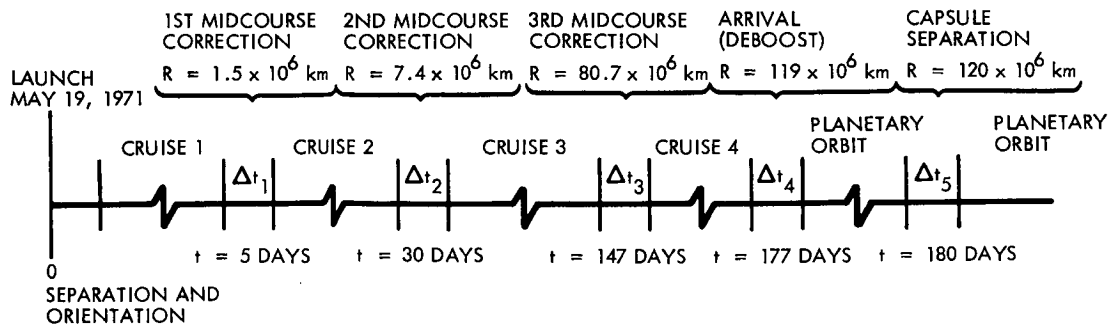
Figure 70. Typical Voyager Mission Maneuver Profile
