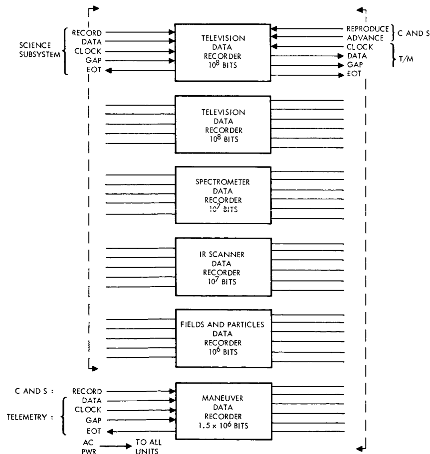
Figure 91. Data Storage Subsystem Block Diagram
