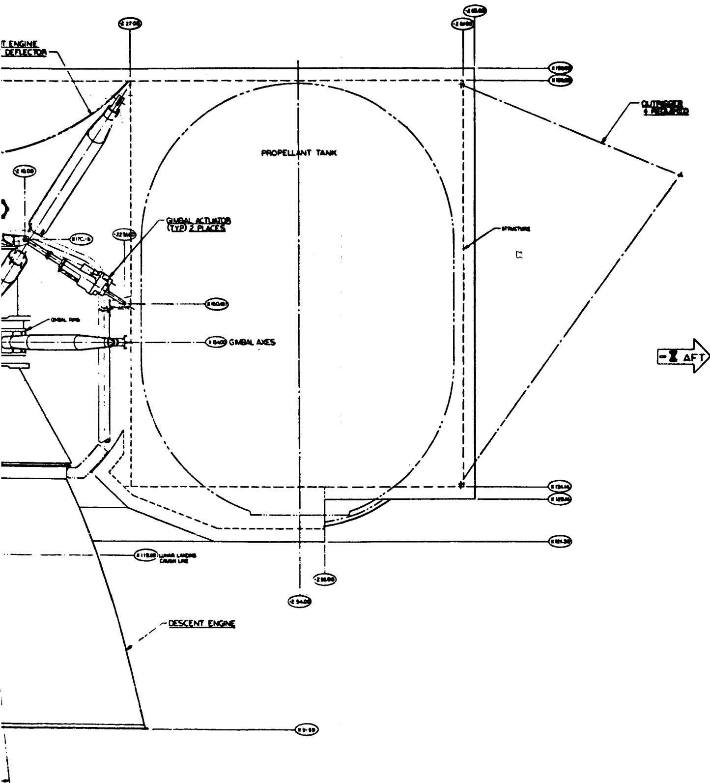
Figure 152. Descent Propulsion Engine Installation
