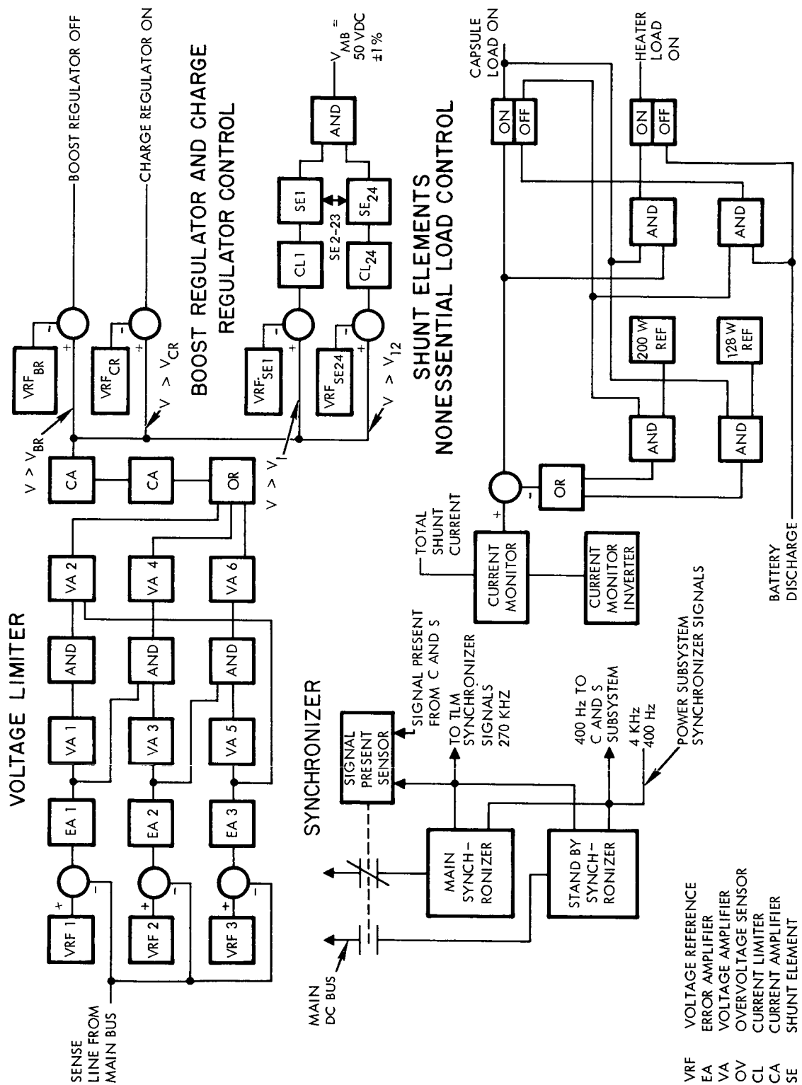
Figure 8. Power Control Unit Functional Block Diagram
