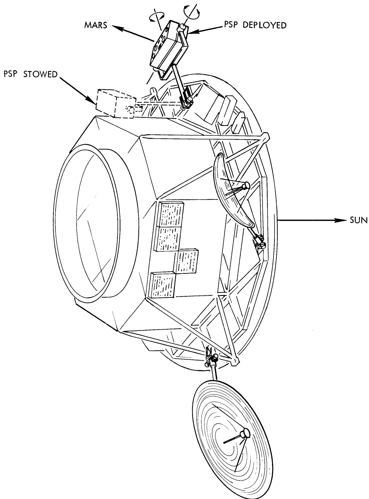
Figure 167. PSP Gimbal Assembly
