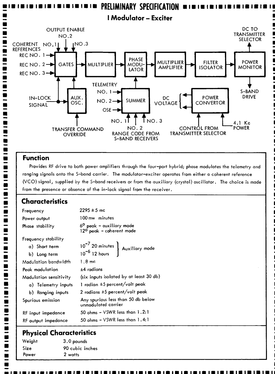
Figure 57. Preliminary Specification - Modulator-Exciter
