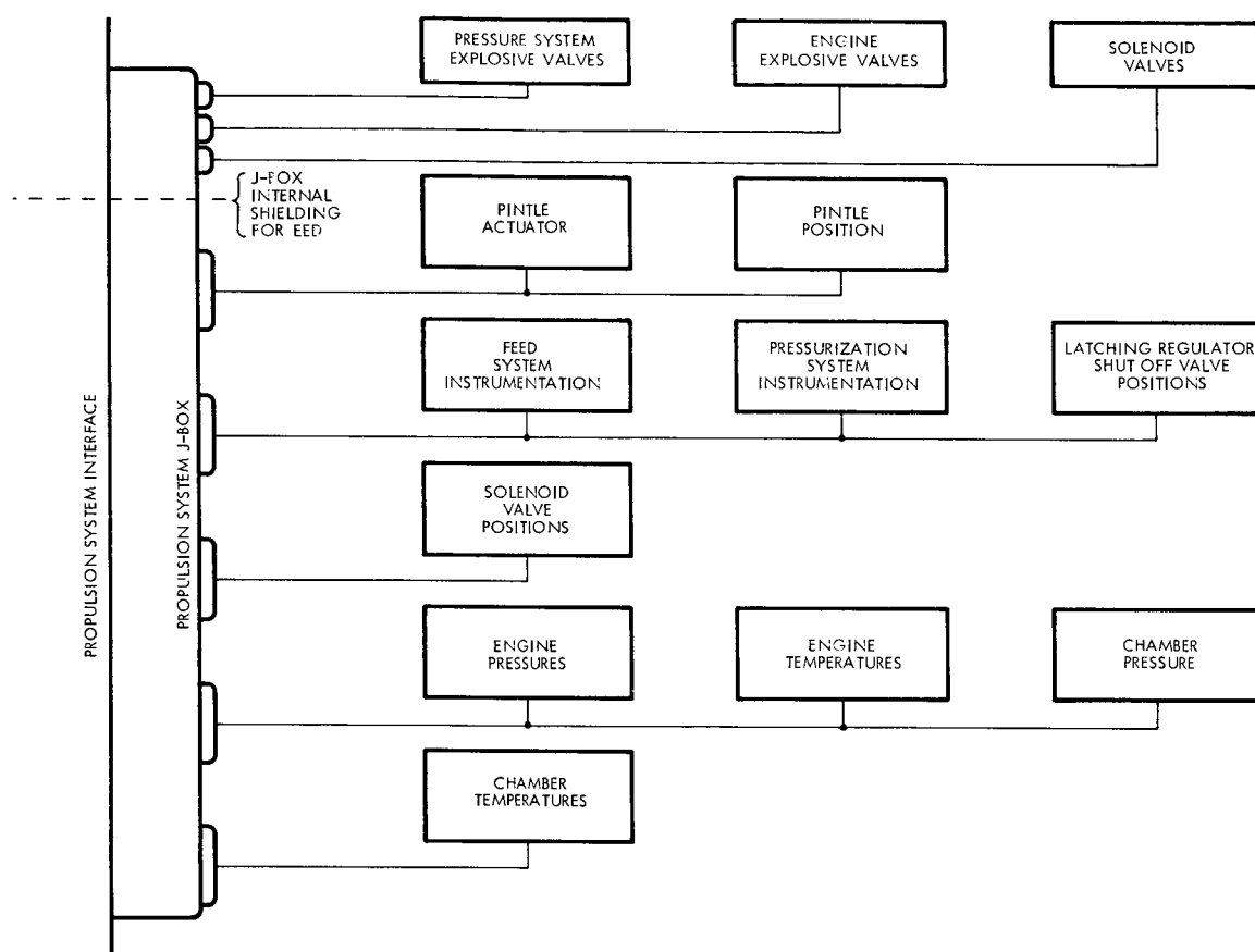
Figure 159. Propulsion Subsystem Electrical Block Diagram
