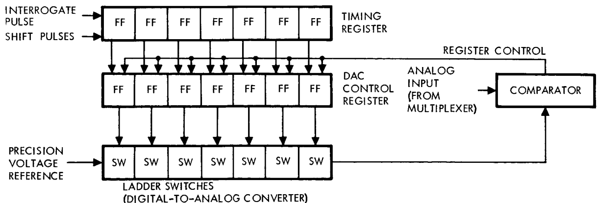
Figure 86. Analog-to-Digital Converter
