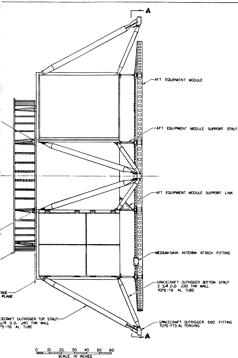
Figure 110. Structural Configuration—1971 Voyager Spacecraft
