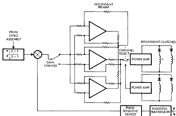
Figure 38. Thrust Vector Control Circuitry
