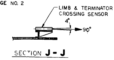
Figure 111. Sensor Geometry—1971 Voyager Spacecraft
