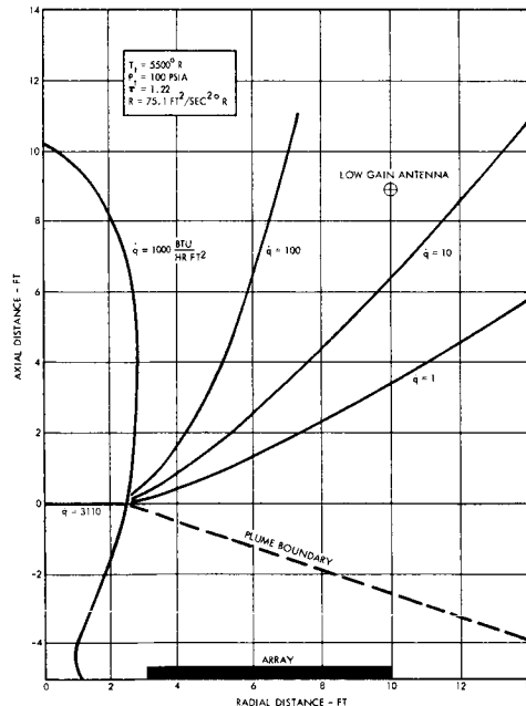
Figure 141. Plume Convective Heating Characteristics
