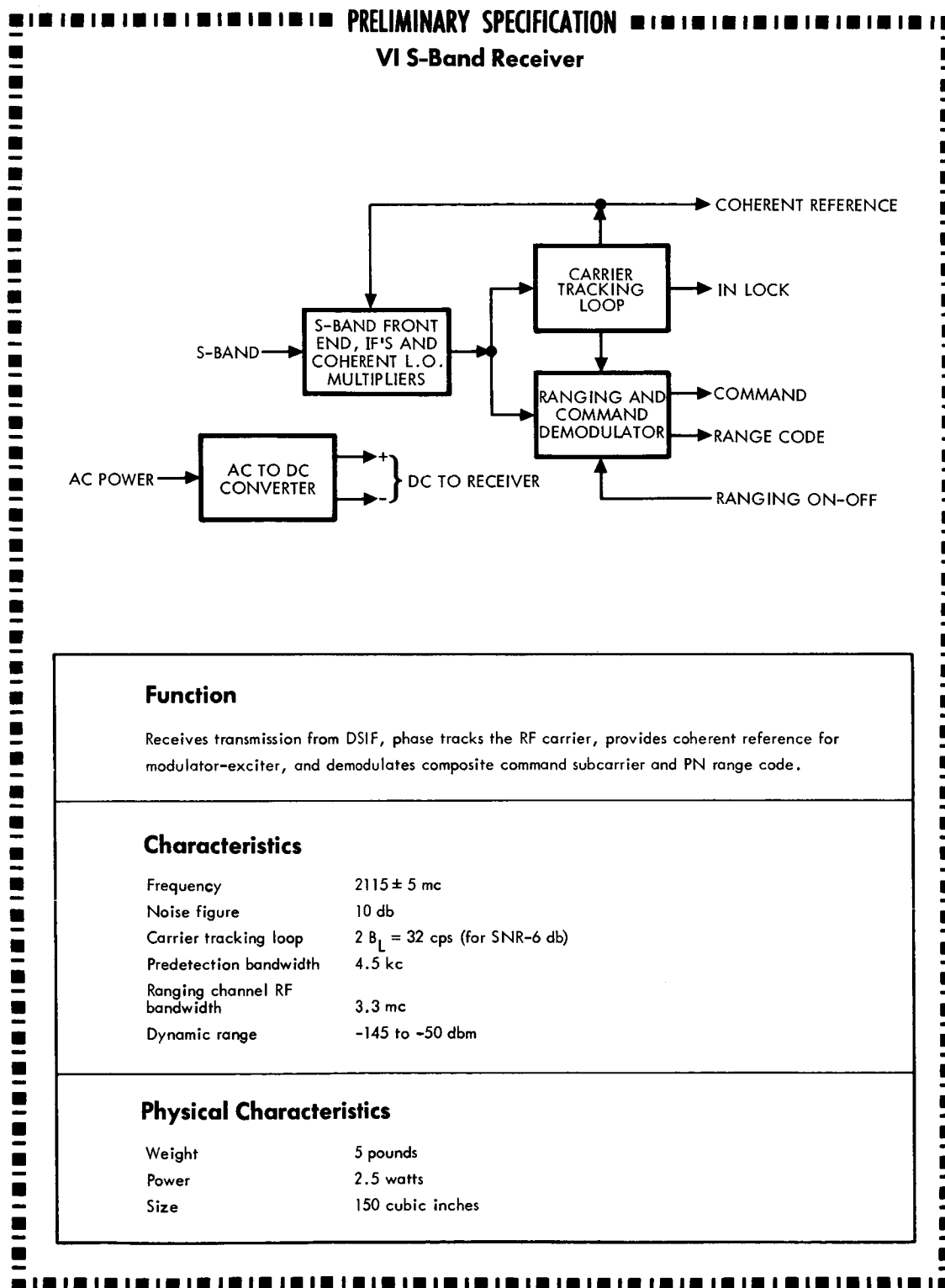
Figure 61. Preliminary Specification - VI S-Band Receiver
