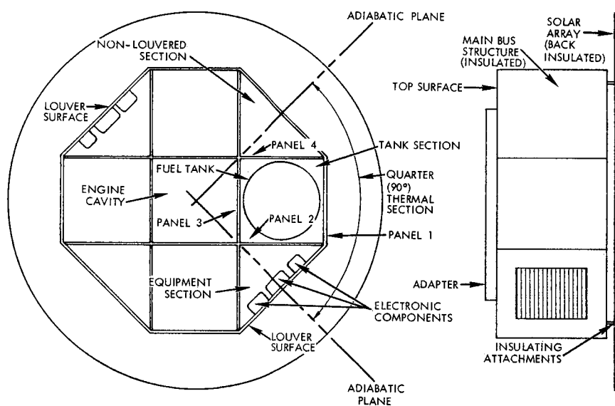
Figure 135. Mathematical Model Node Designation
