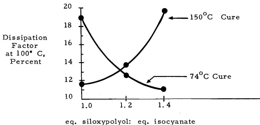
Figure 8. Dissipation factors of siloxyurethanes cured at various temperatures.
