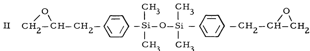
1,3-bis(epoxypropylphenyl)tetramethyldisiloxane
