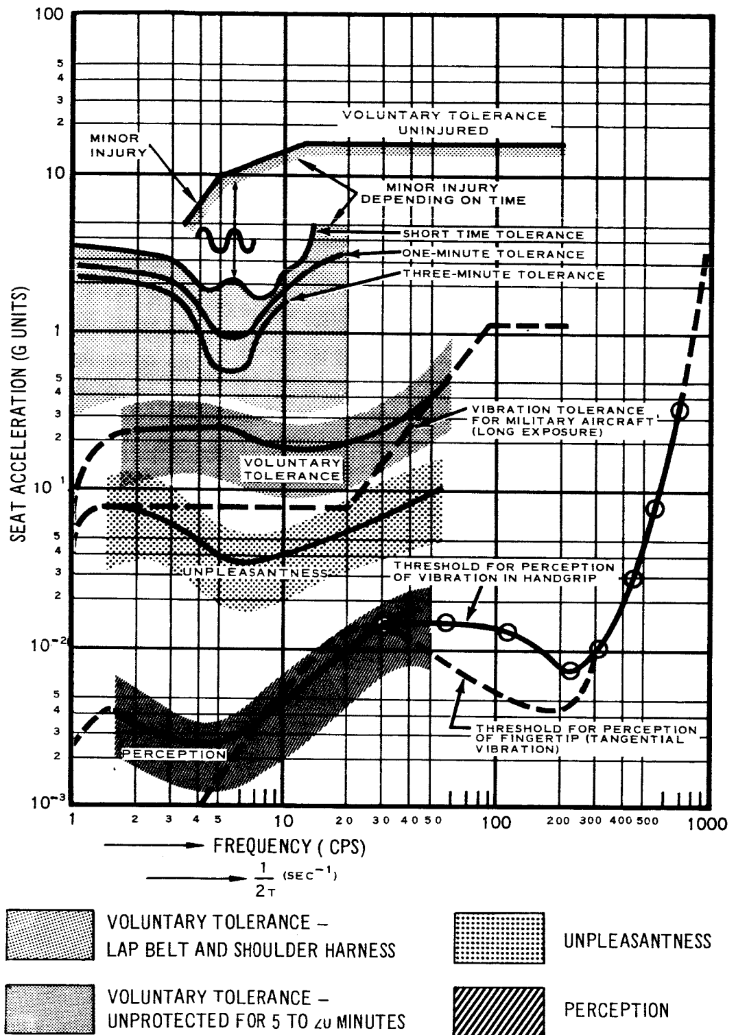
Figure 72. Criteria for vibration tolerance
