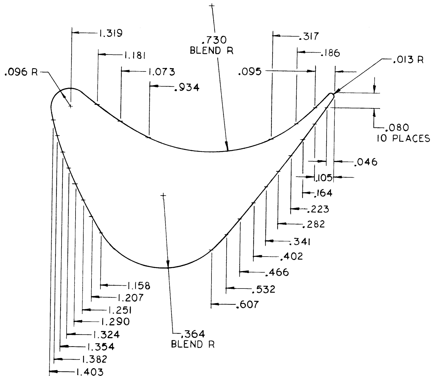
Figure 11. Reversing Vane Profile and Coordinates
