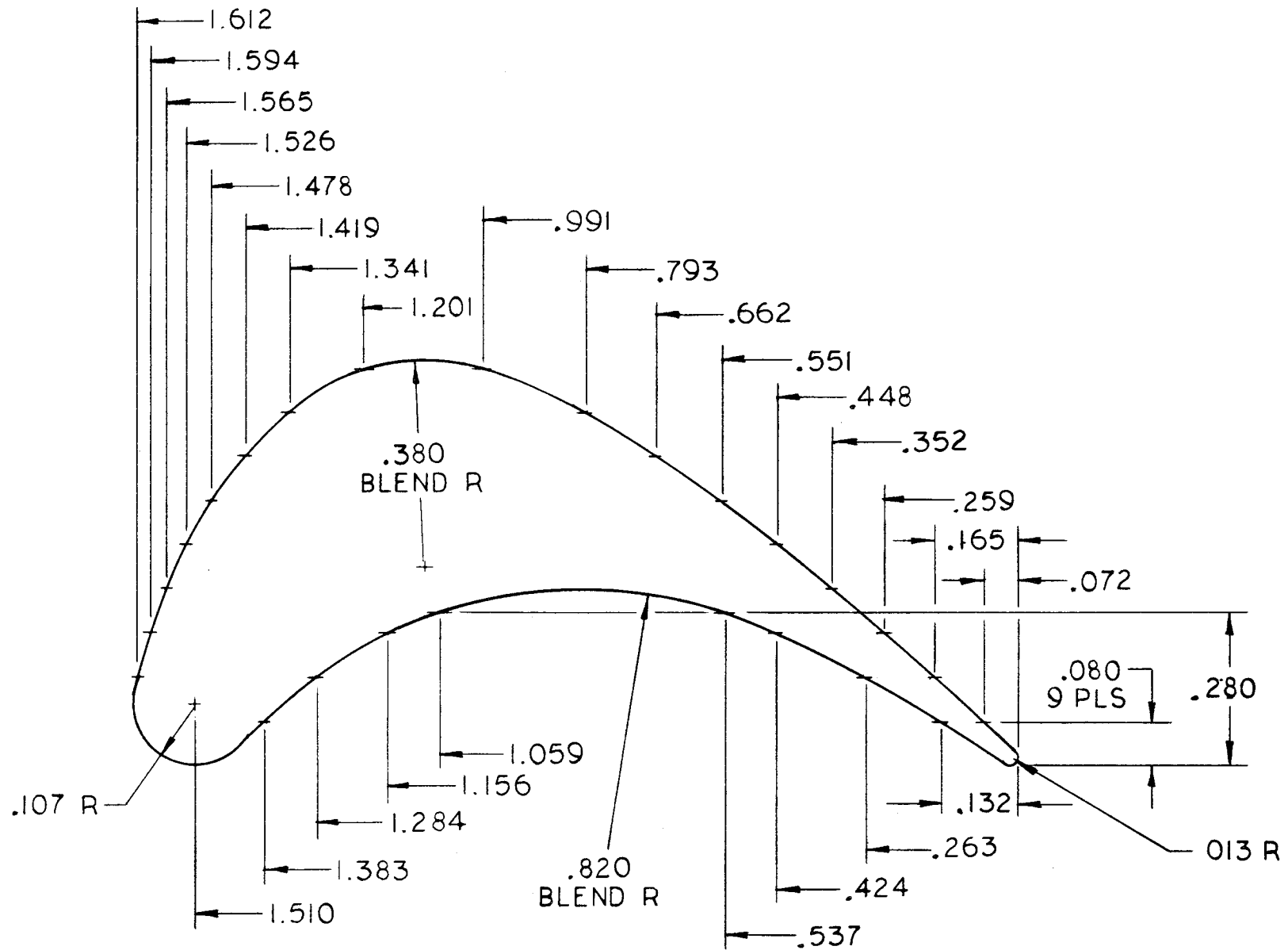
Figure 12. Second Rotor Blade Profile and Coordinates
