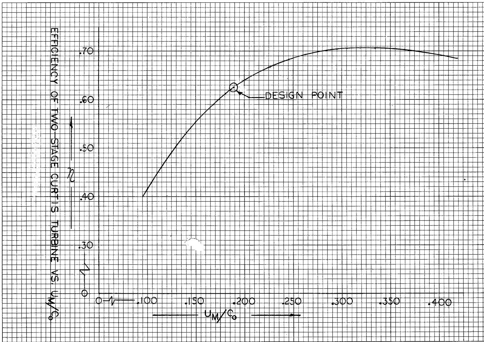
Figure 7. Efficiency of Two-Stage Curtis Turbine versus U_M/C_0
