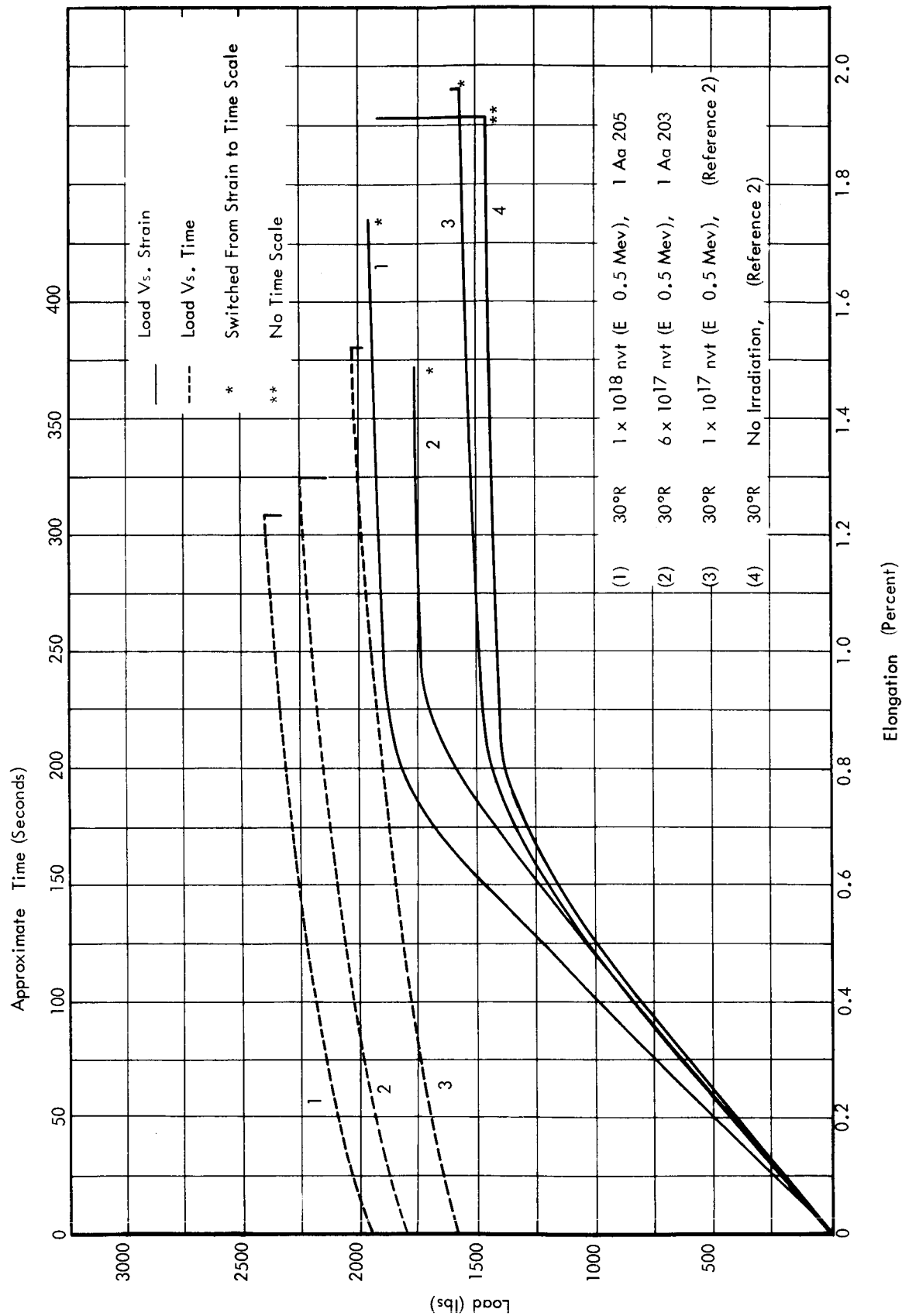
FIGURE 25 TYPICAL LOAD-ELONGATION CURVES FOR TITANIUM 55A
