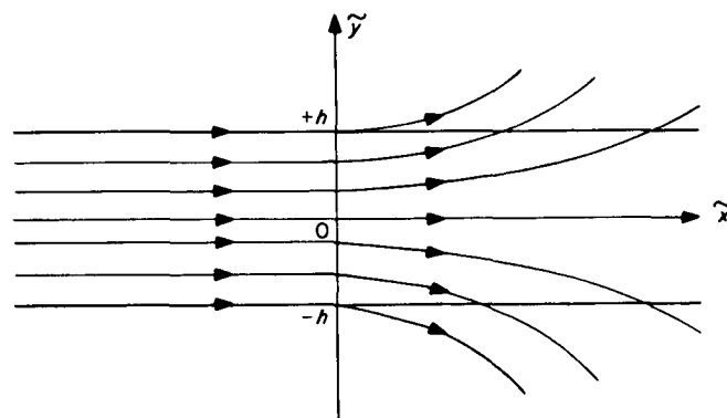
Fig. 2. Mathematical model: \tilde{B}_y^*(0, \tilde{y}) = 0
