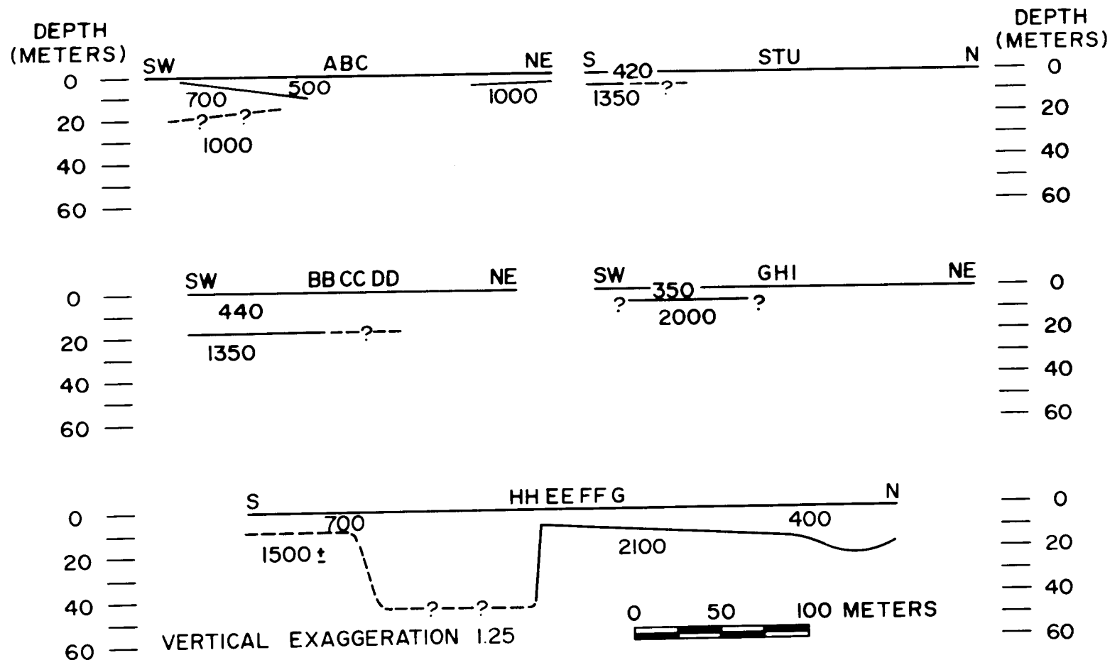
Figure 3.--Diagrammatic sections of profiles A B C, S T U, B B C C D D, G H I and H H E E F F G and spread H H. Velocities shown are in meters per second.
