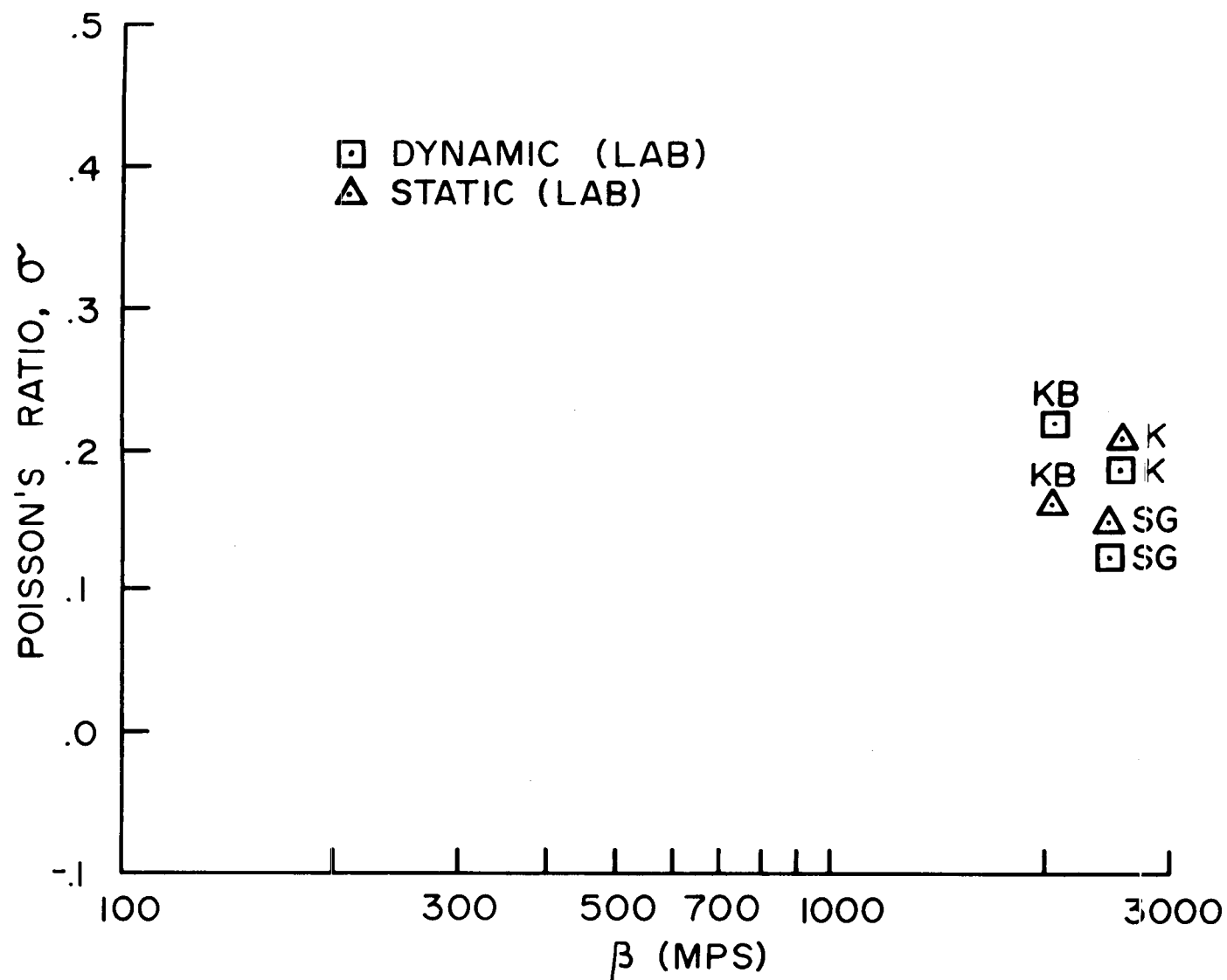
Figure 6.--Laboratory Poisson's ratio vs. SH-wave velocity.
