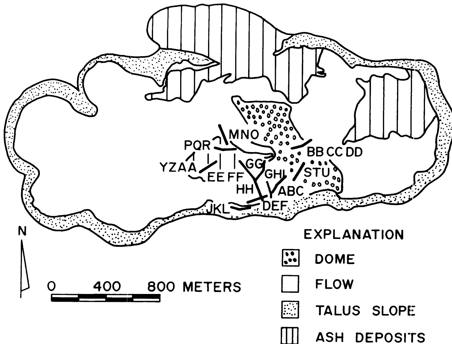
Figure 5.--Relation of refraction profiles and morphologic units of the Southern Coulee (after Loney, 1964).
