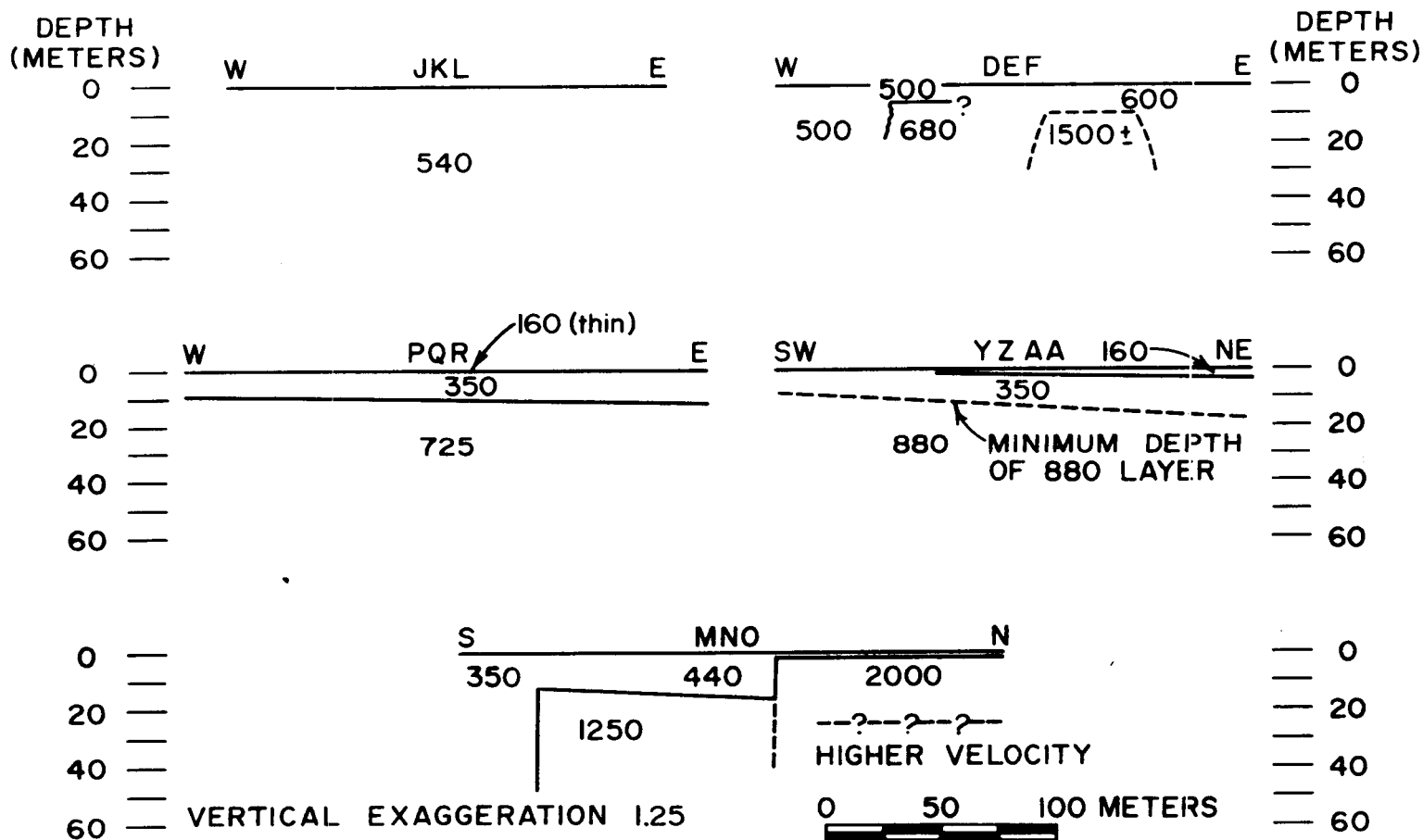
Figure 2.--Diagrammatic sections of profiles J K L, Y Z AA, P Q R, M N O, and D E F. Velocities shown are in meters per second.
