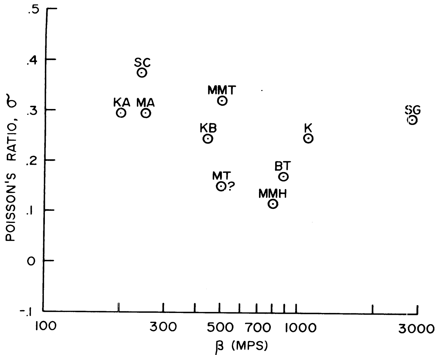
Figure 2.--In situ Poisson's ratio vs. SH-wave velocity.
