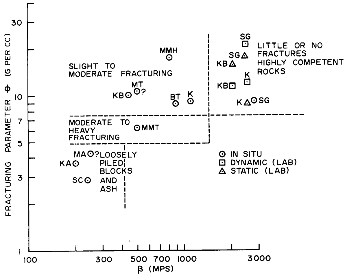
Figure 10.--Fracturing parameter as a function of SH-wave velocity.
