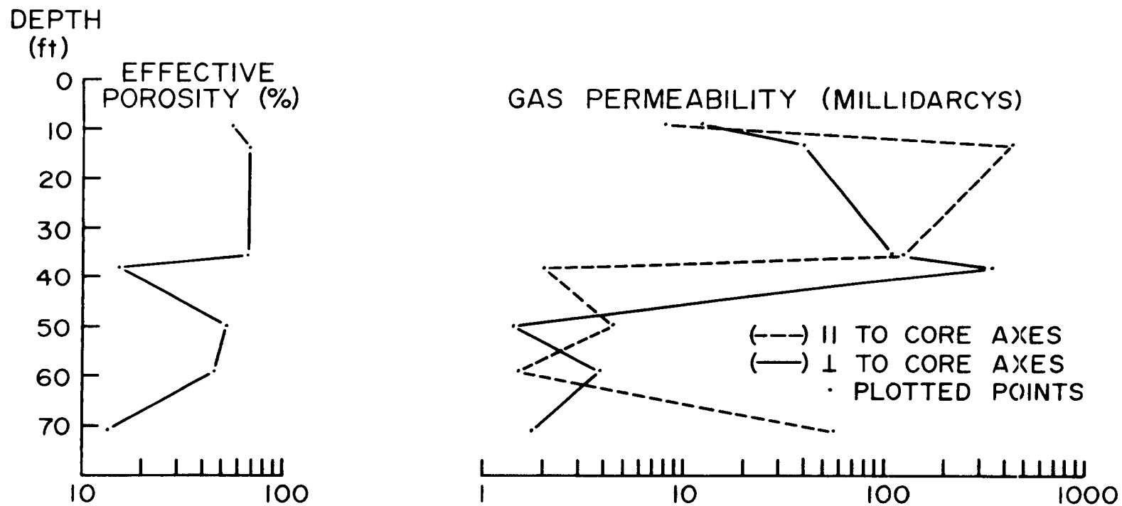
Figure 3.--Distribution of effective porosity and nitrogen permeability of pumice samples in the SC-2 drill hole.
