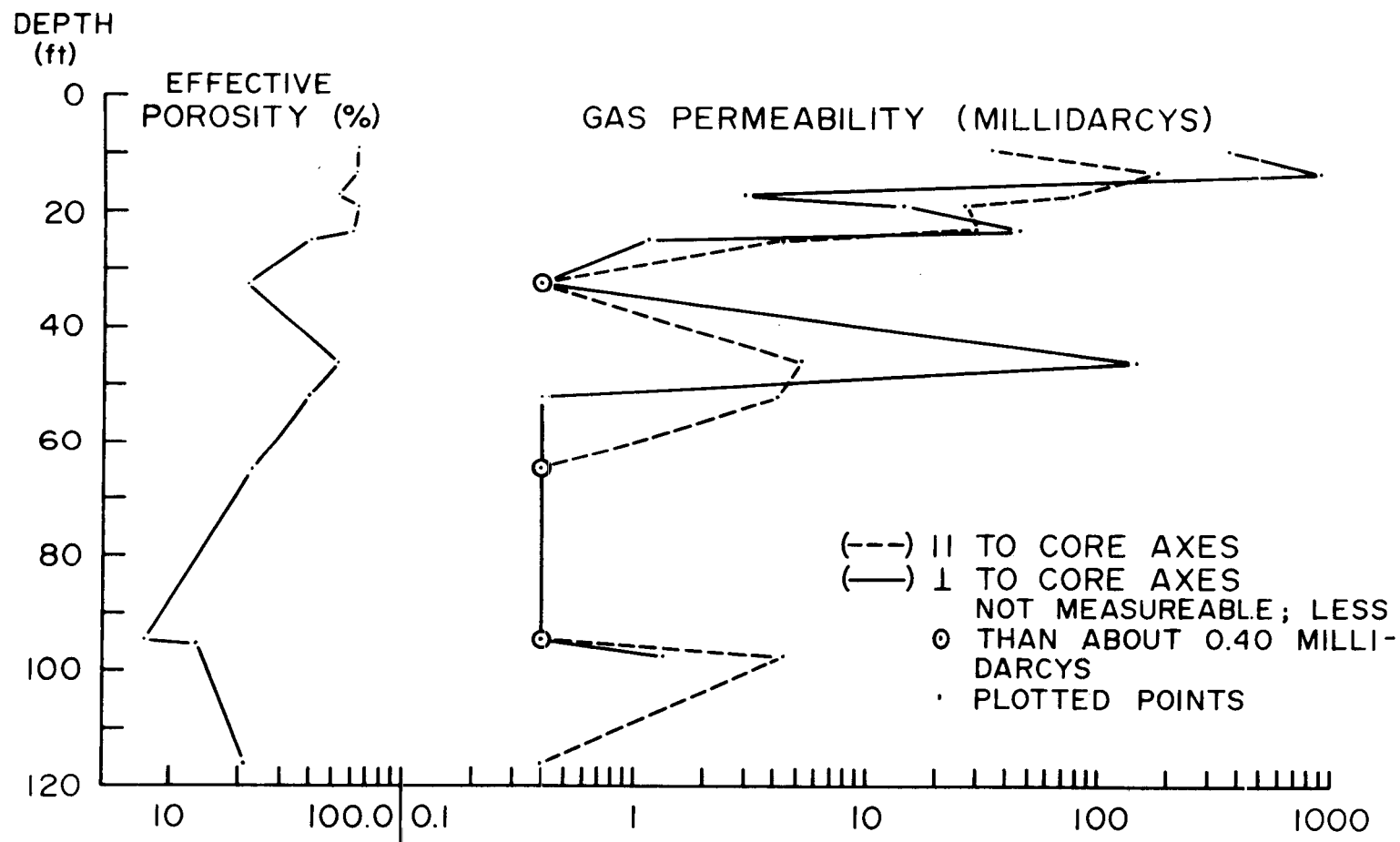
Figure 5.--Distribution of effective porosity and nitrogen permeability of pumice samples in the SC-4 drill hole.
