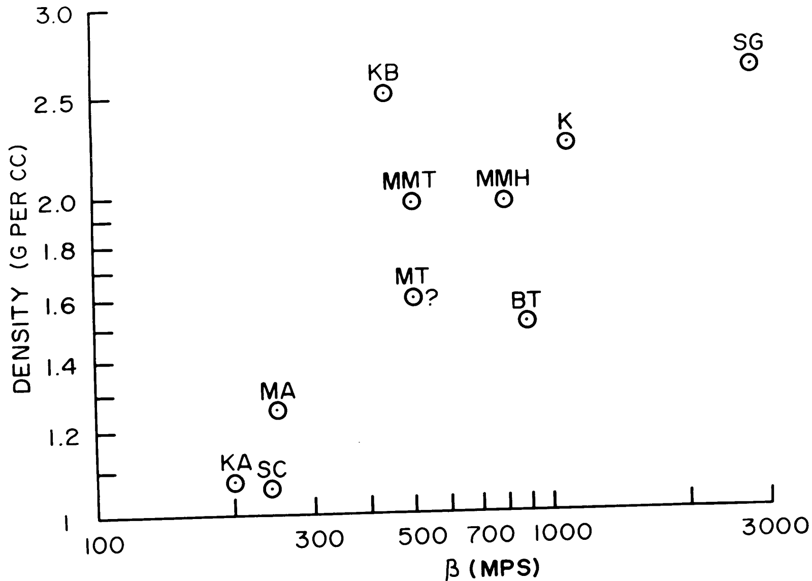
Figure 1.--Dry bulk density vs. SH-wave velocity.
