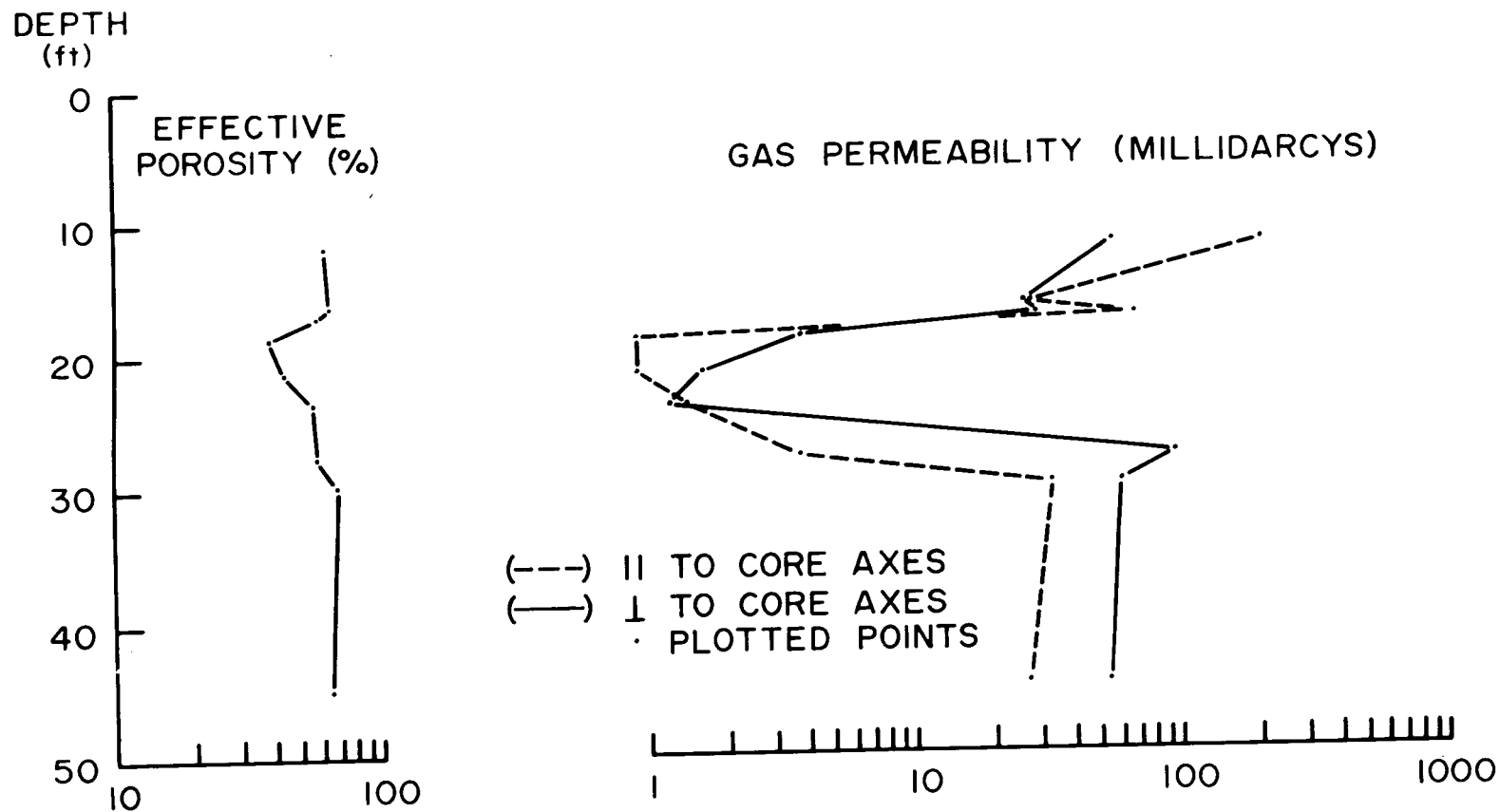
Figure 4.--Distribution of effective porosity and nitrogen permeability of pumice samples in the SC-3 drill hole Southern Coulee-Mono Craters, California.
