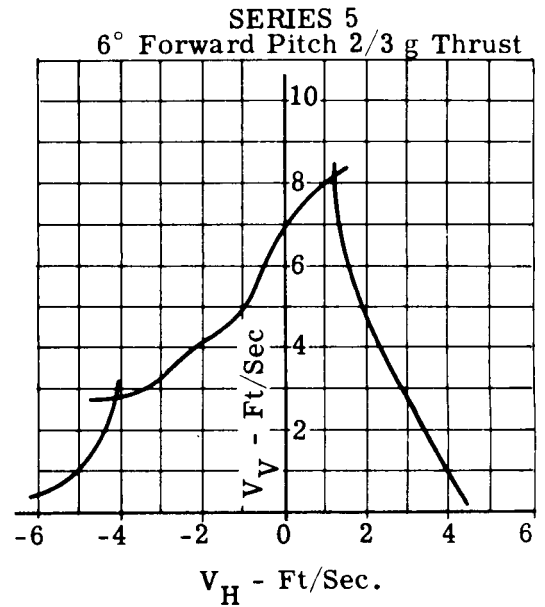
Figure 11. Vehicle Pitch (-6°)
