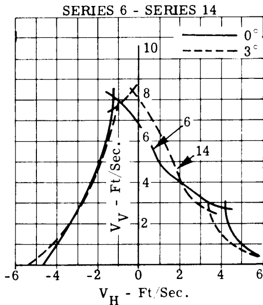
Figure 51. Effect of Ground Slope Pitched Vehicle ( 6^\circ )
