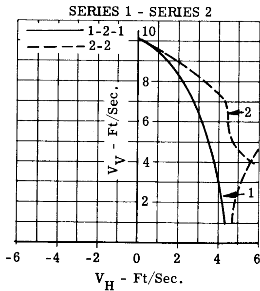
Figure 39. Effect of Yaw Standard Landing
