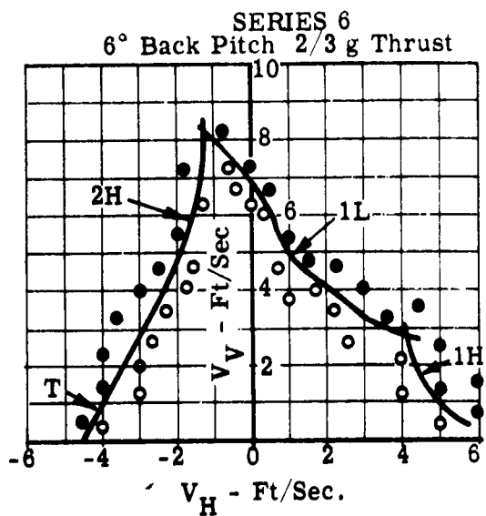
Figure 8. Vehicle Pitch 6°
