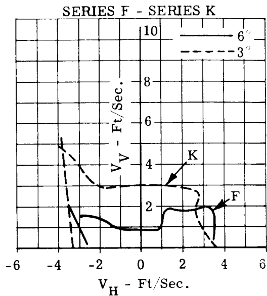
Figure 48. Effect of Pitch, 1-2-1 Yaw With 3° Ground Slope
