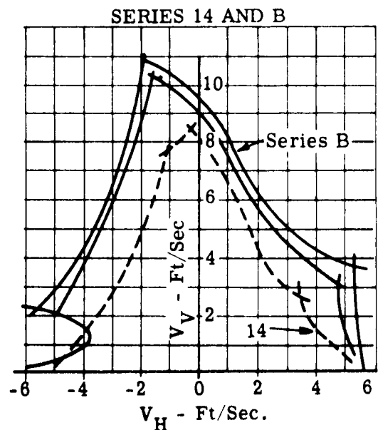
Figure 27. Effect of Increased Load Pitched Vehicle with Small Ground Slope
