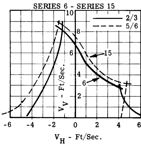
Figure 42. Effect of Thrust Pitched Vehicle ( 6^\circ )
