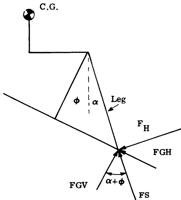
Figure B-3. Footpad Force Diagram
