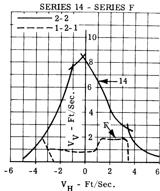
Figure 37. Effect of Yaw Pitched Vehicle ( 6^\circ ) With Ground Slope
