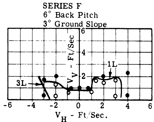
Figure 31. 1-2-1 Yaw With 6° Pitch and 3° Ground Slope
