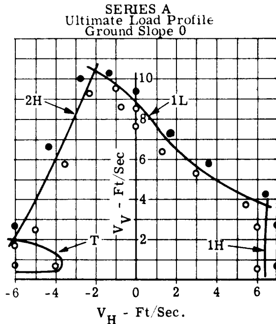
Figure 24. Ultimate Load With Pitched Vehicle ( 6^\circ )
