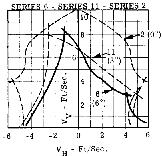
Figure 44. Effect of Pitch, 2-2 Yaw
