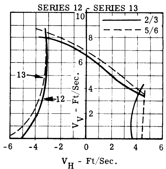
Figure 43. Effect of Thrust Ground Slope 3^\circ
