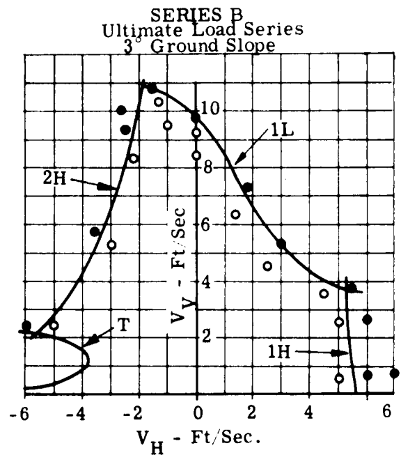
Figure 25. Ultimate Load With Pitched Vehicle ( 6^\circ ) and Small Ground Slope
