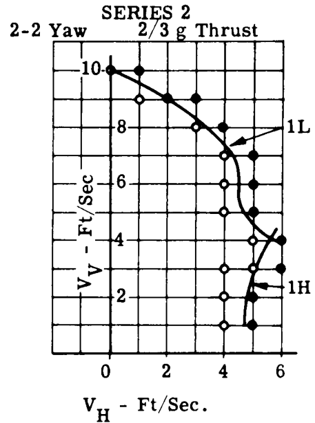
Figure 5. Standard Series With 2-2 Yaw
