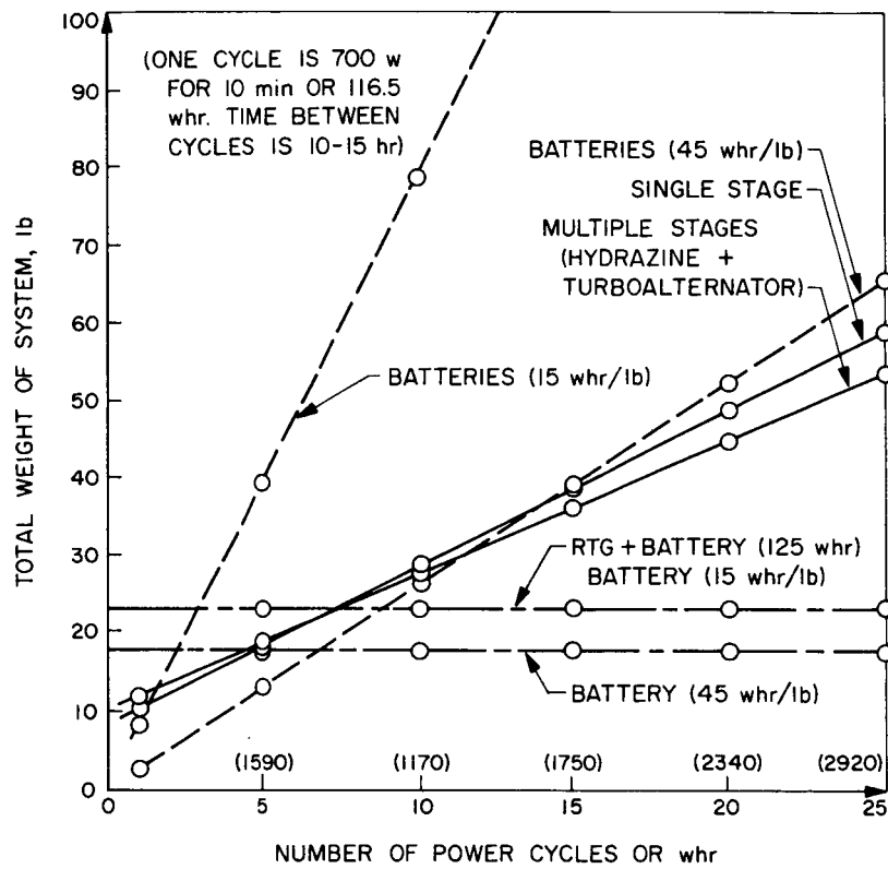
Fig. 1. Weight vs power cycles for various landing capsule power systems
