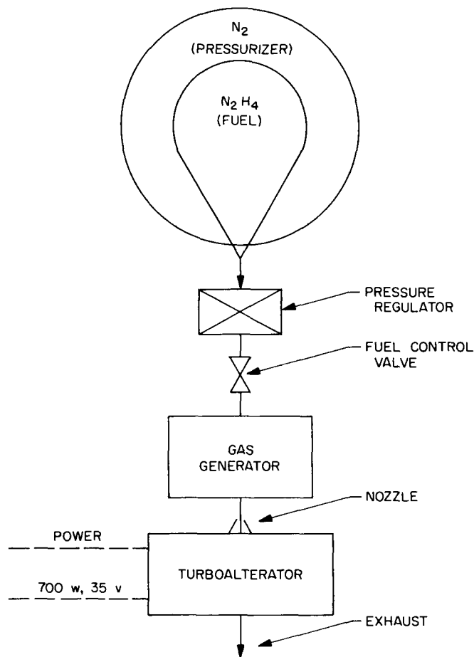
Fig. 3. Hydrazine-turboalternator system
