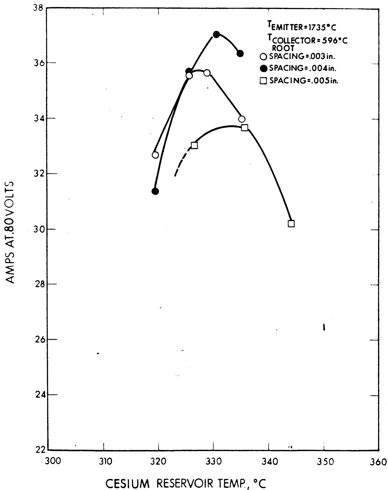
FIG. 2-3 RESERVOIR TEMPERATURE VERSUS CURRENT IN AMPERES WITH 0.003, 0.004, AND 0.005 INCH SPACING, T_{\text{COLLECTOR}} = 596^{\circ}\text{C} (all dc data points)
