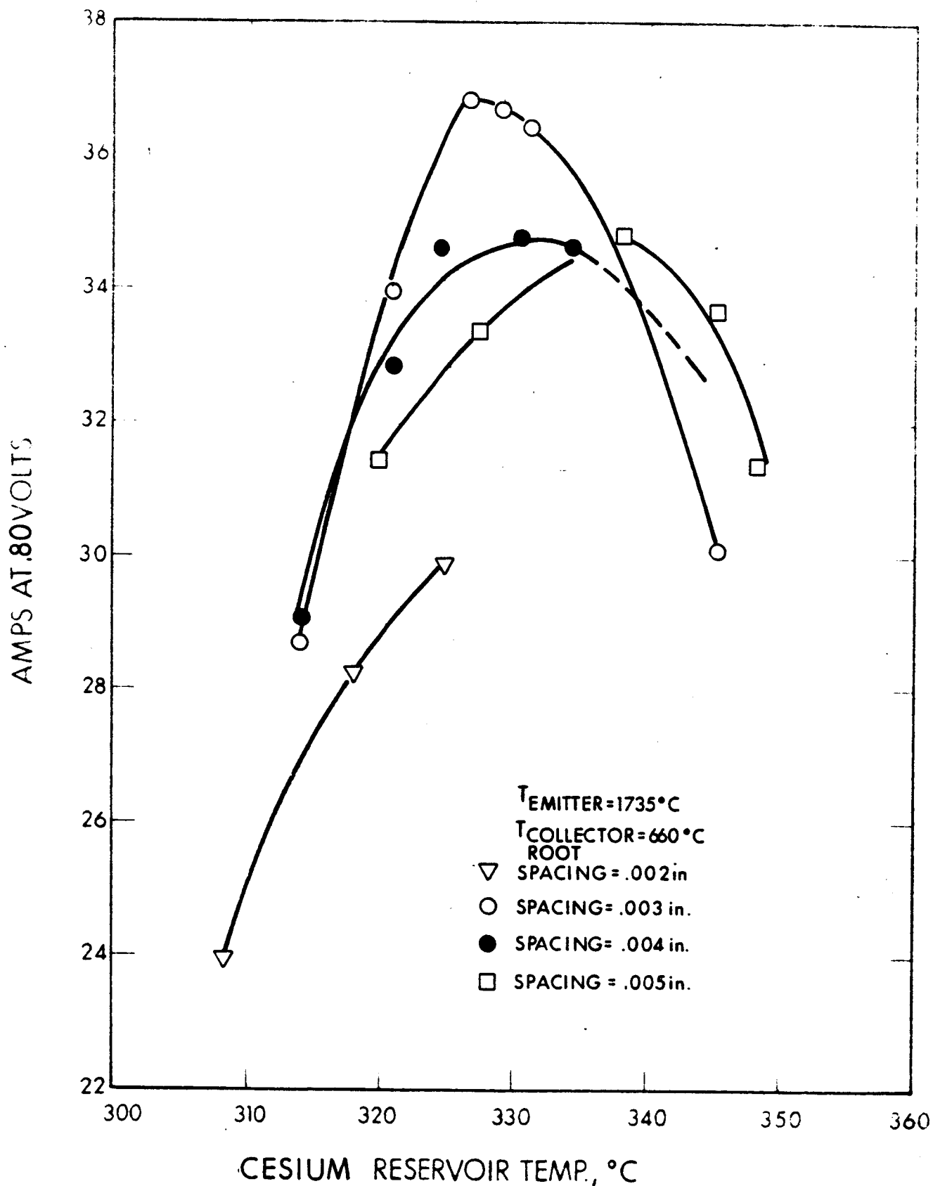
FIG. 2-5 RESERVOIR TEMPERATURE VERSUS CURRENT IN AMPERES WITH 0.002, 0.003, 0.004, AND 0.005 INCH SPACING, T_{\text{COLLECTOR}} = 660^{\circ}\text{C} (all dc data points)
