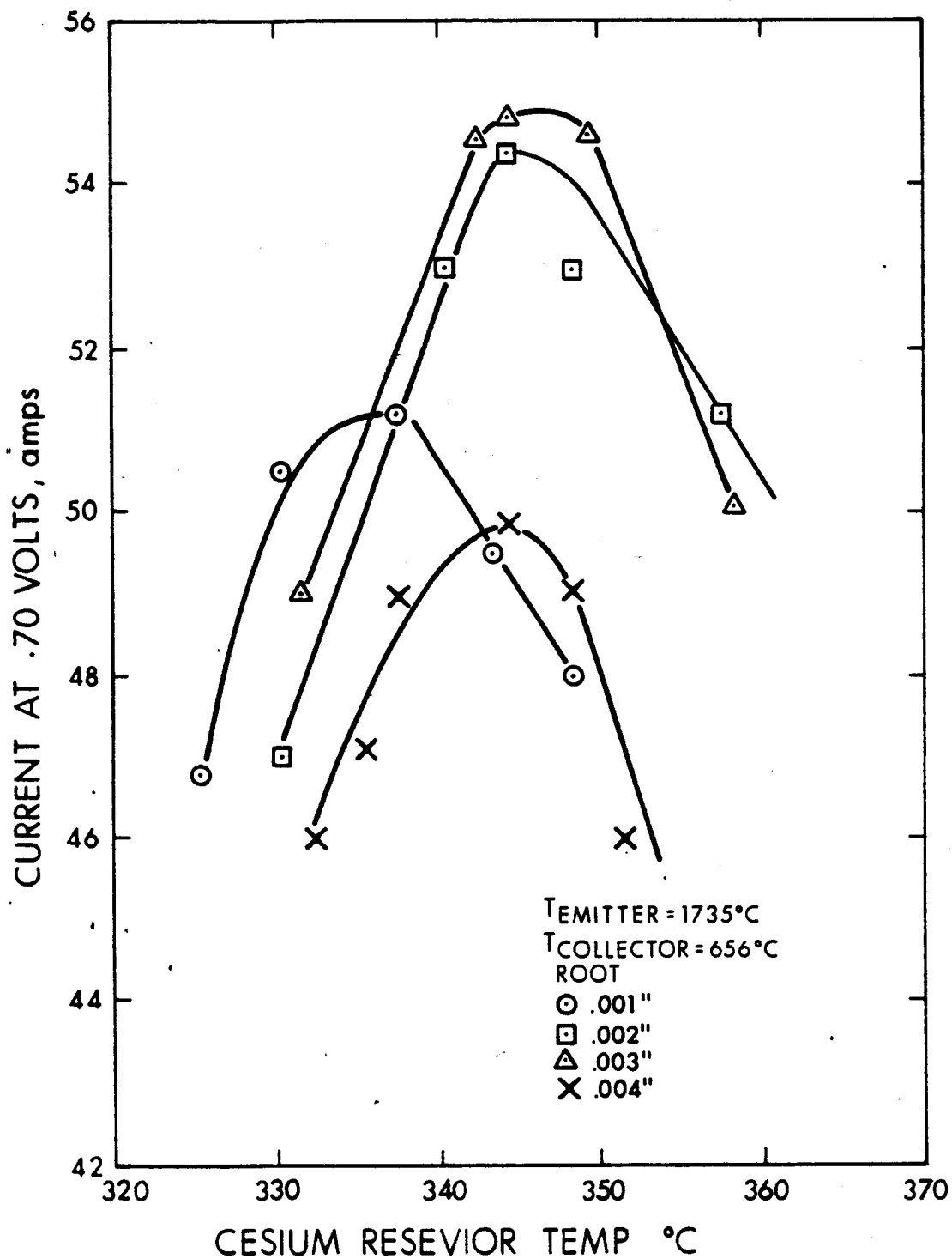
FIG. 2-6 0.7 VOLT CONVERTER OPTIMIZATION, T_{\text{COLLECTOR}} = 656-665^{\circ}\text{C} (all dc data points) ROOT
