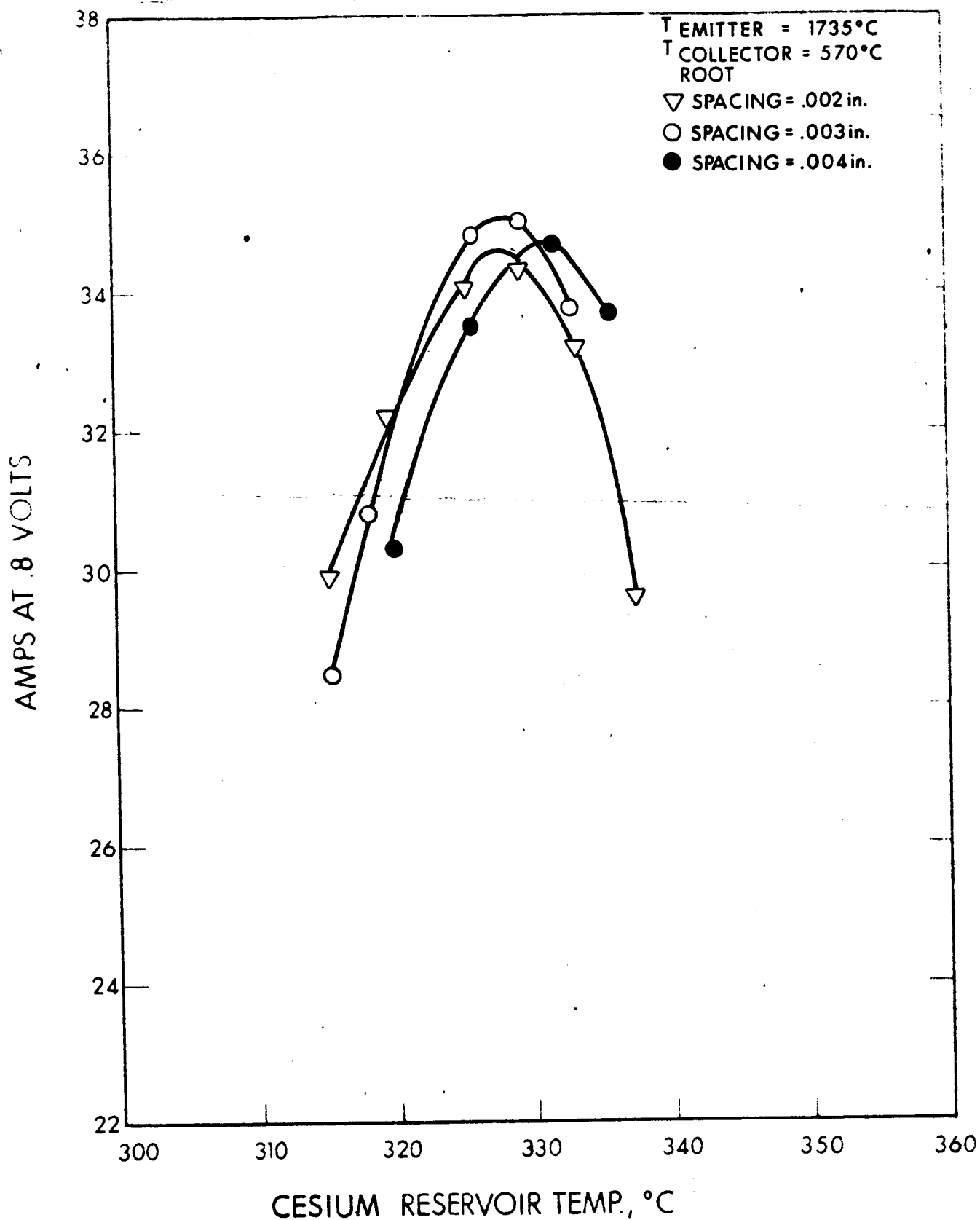
FIG. 2-2 RESERVOIR TEMPERATURE VERSUS CURRENT IN AMPERES WITH 0.002, 0.003, AND 0.004 INCH SPACING, T_{\text{COLLECTOR}} = 570^{\circ}\text{C} (all dc data points) ROOT
