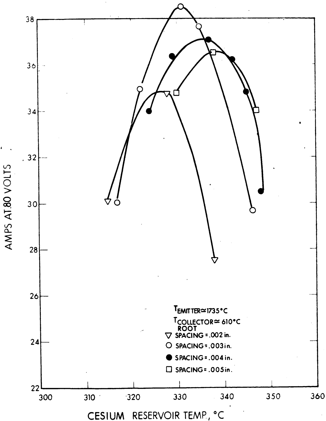
FIG. 2-4 RESERVOIR TEMPERATURE VERSUS CURRENT IN AMPERES WITH 0.002, 0.003, 0.004, and 0.005 INCH SPACING, T_{\text{COLLECTOR}} = 610^{\circ}\text{C} (all dc data points)
