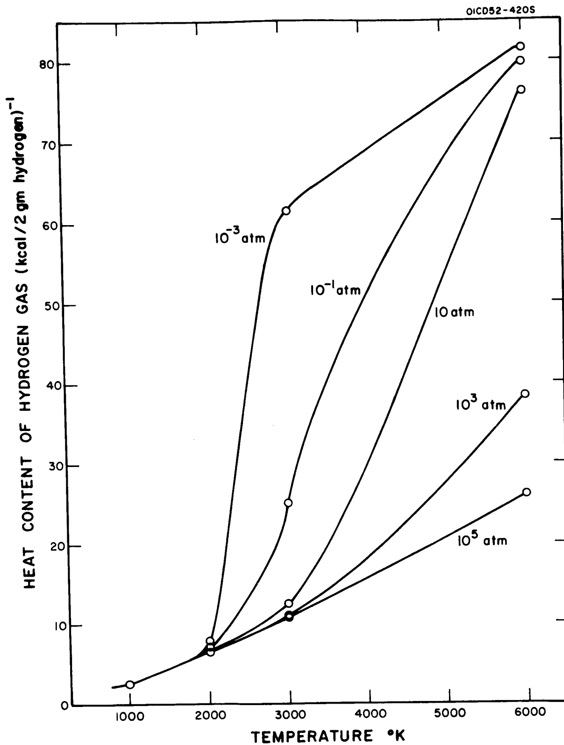
Figure 2. Heat content of 2 gm of hydrogen as a function of temperature and pressure.
