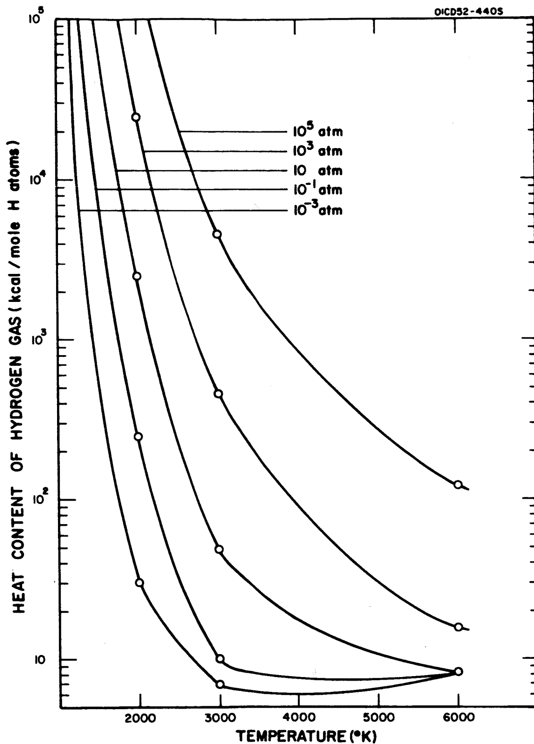
Figure 3. Heat content of hydrogen gas containing one mole of hydrogen atoms as a function of pressure and temperature.
