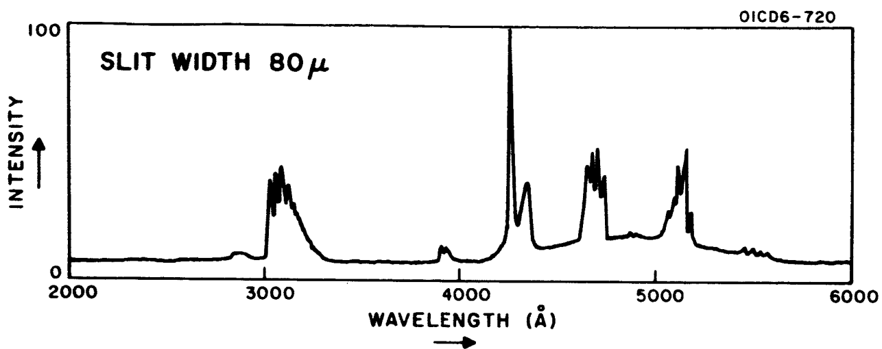
(a) Chemiluminescence spectrum of acetylene and atomic oxygen.
