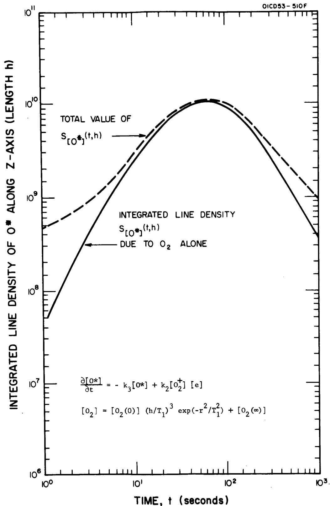
Figure 9. Integrated line density S_{[O^*]}(t,h) of O^* for Inter-penetrability model.
