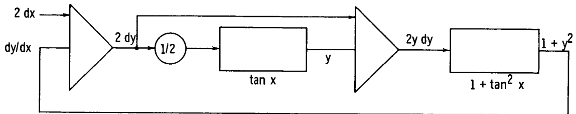
Figure 3.17. - Tan machine.
