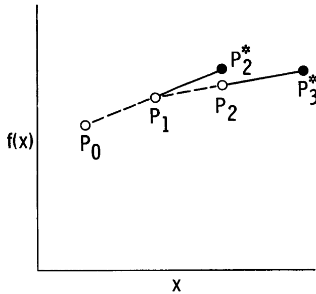
Figure 4. 11. - Scheme for piecewise linear extrapolation.
