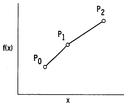
Figure 4.3. - Scheme for piecewise linear interpolation.
